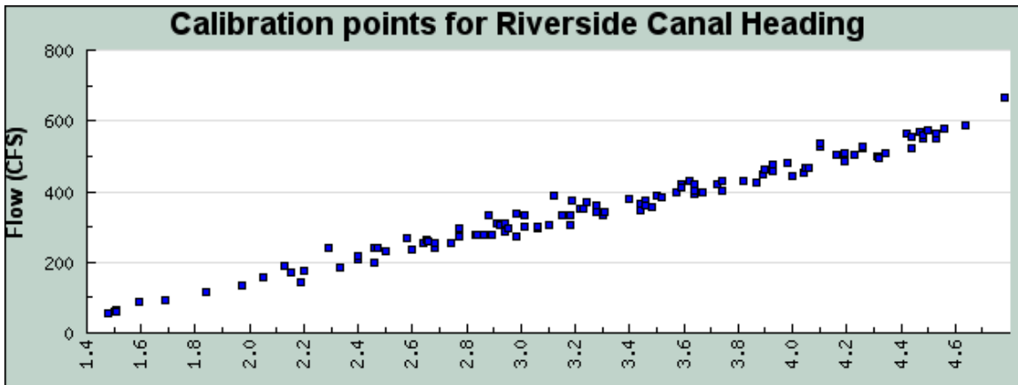
Figure 3 – Typical Calibration Chart
