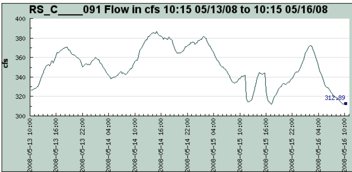
Figure 4 – Typical Hydrograph
