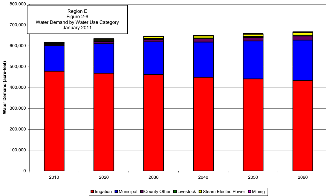
Figure 2-6. Projected Regional Water Demand by Water Use Category
