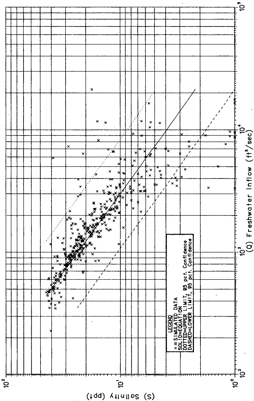
Figure 5-21. Average Monthly Salinity Versus Average Monthly Gaged Inflow, San Antonio Bay, 1940-1976
