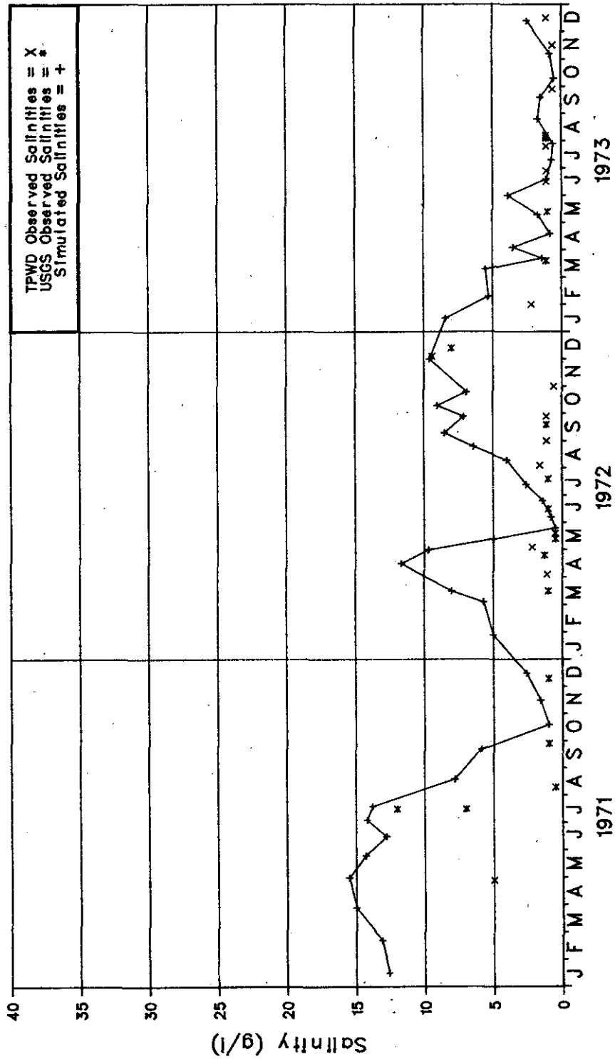
Figure 5-12. Comparison of Observed and Simulated Salinities, Guadalupe Estuary, Line 225, Site 02
