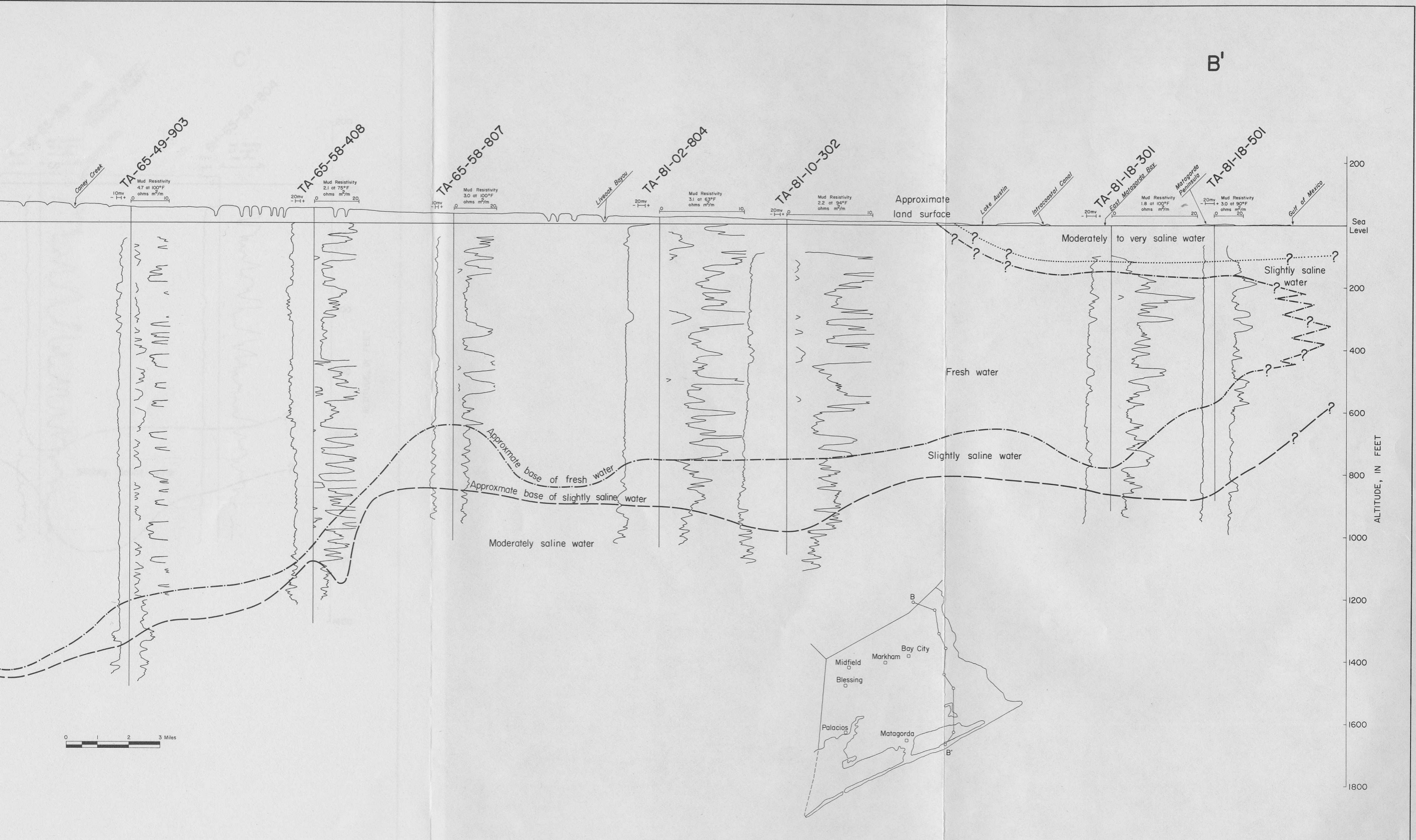
Figure 34 Section B-B' Showing Approximate Bases of Fresh Water and Slightly Saline Water
