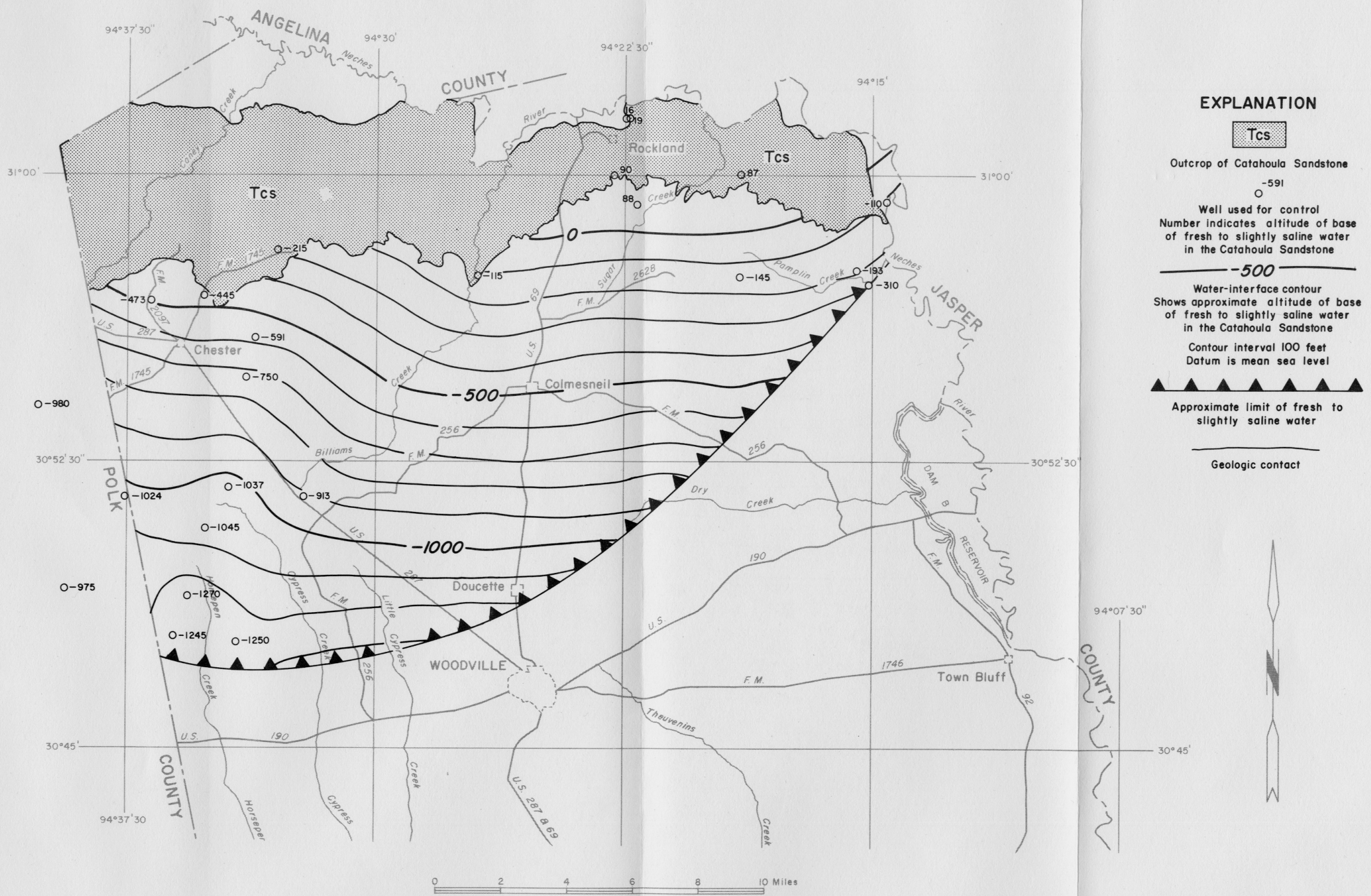
Figure 11 Approximate Altitude of the Base of Fresh to Slightly Saline Water in the Catahoula Sandstone, Northern Tyler County
