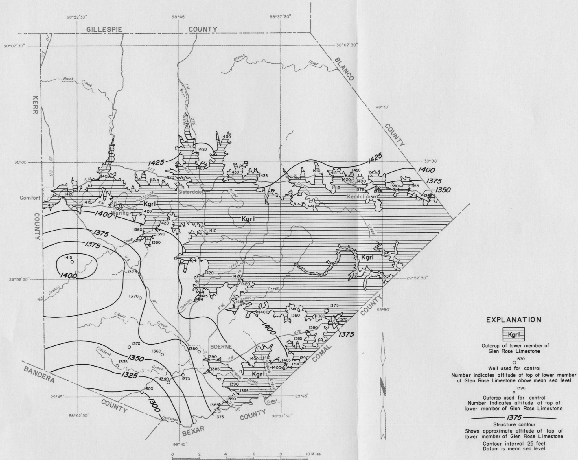
Figure 4 Altitude of the Top of the Lower Member of the Glen Rose Limestone
