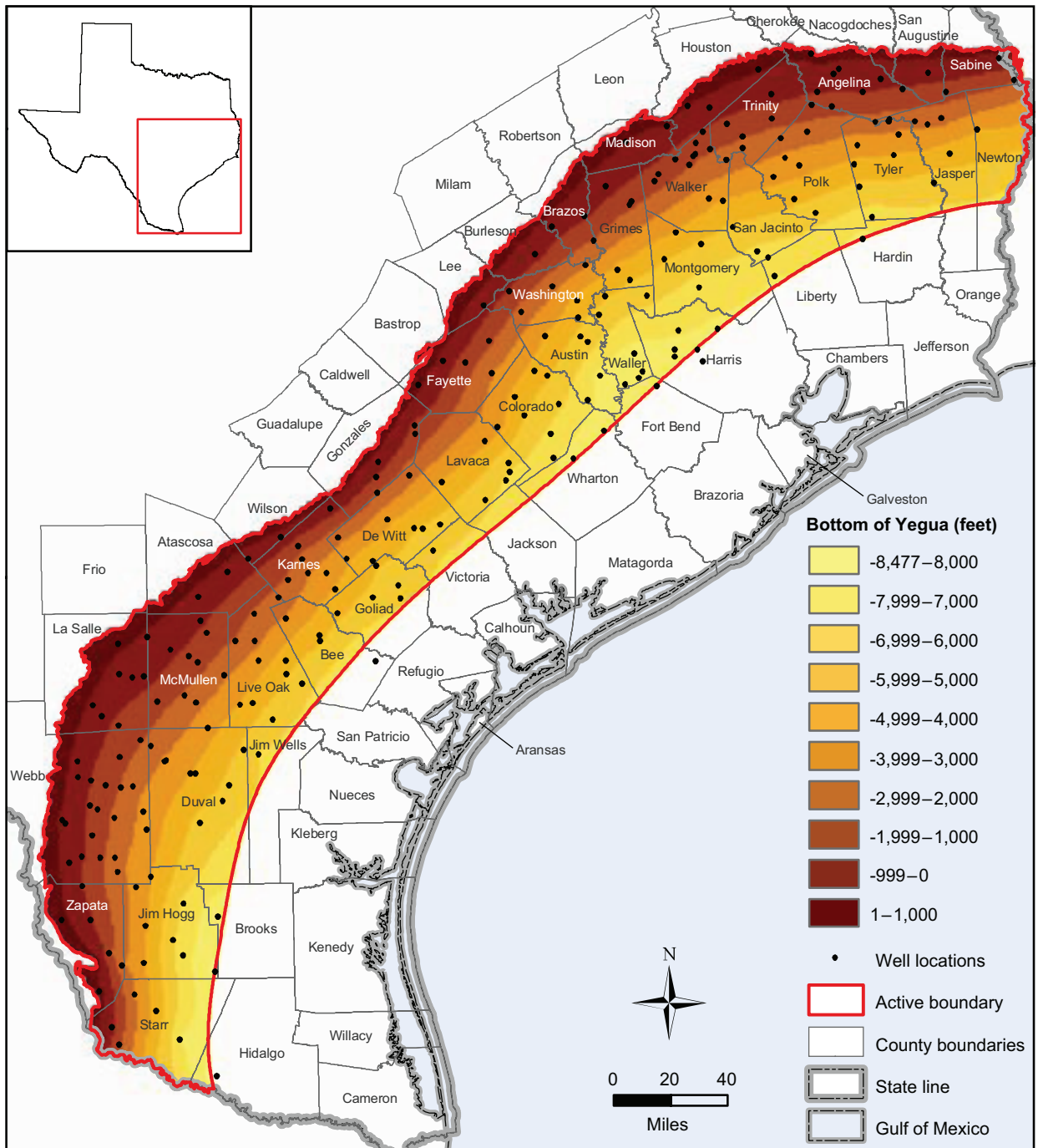
Figure 6-5. Base of Yegua-Jackson Aquifer (Knox and others, 2007).
