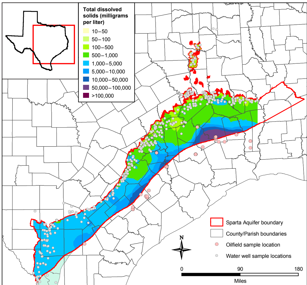
Figure 5-11. Map of total dissolved solids in the Sparta Aquifer and equivalent downdip section in Texas.
