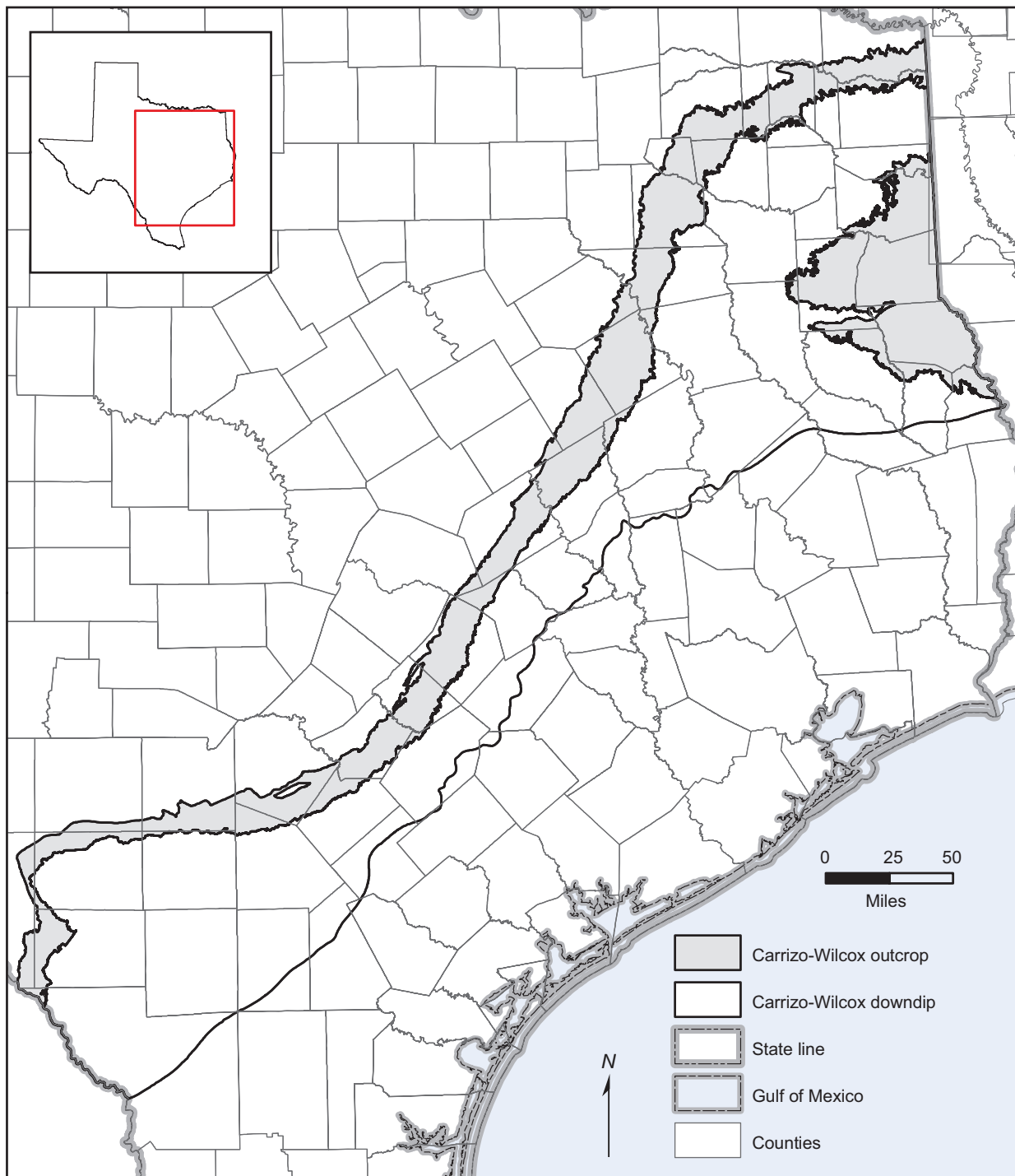
Figure 3-1. Location of Carrizo-Wilcox Aquifer in Texas.
