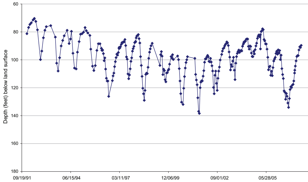
Figure 9-6. Seasonal historical water level declines in Carrizo Aquifer, Atascosa County, Well Number 68-60-912.
