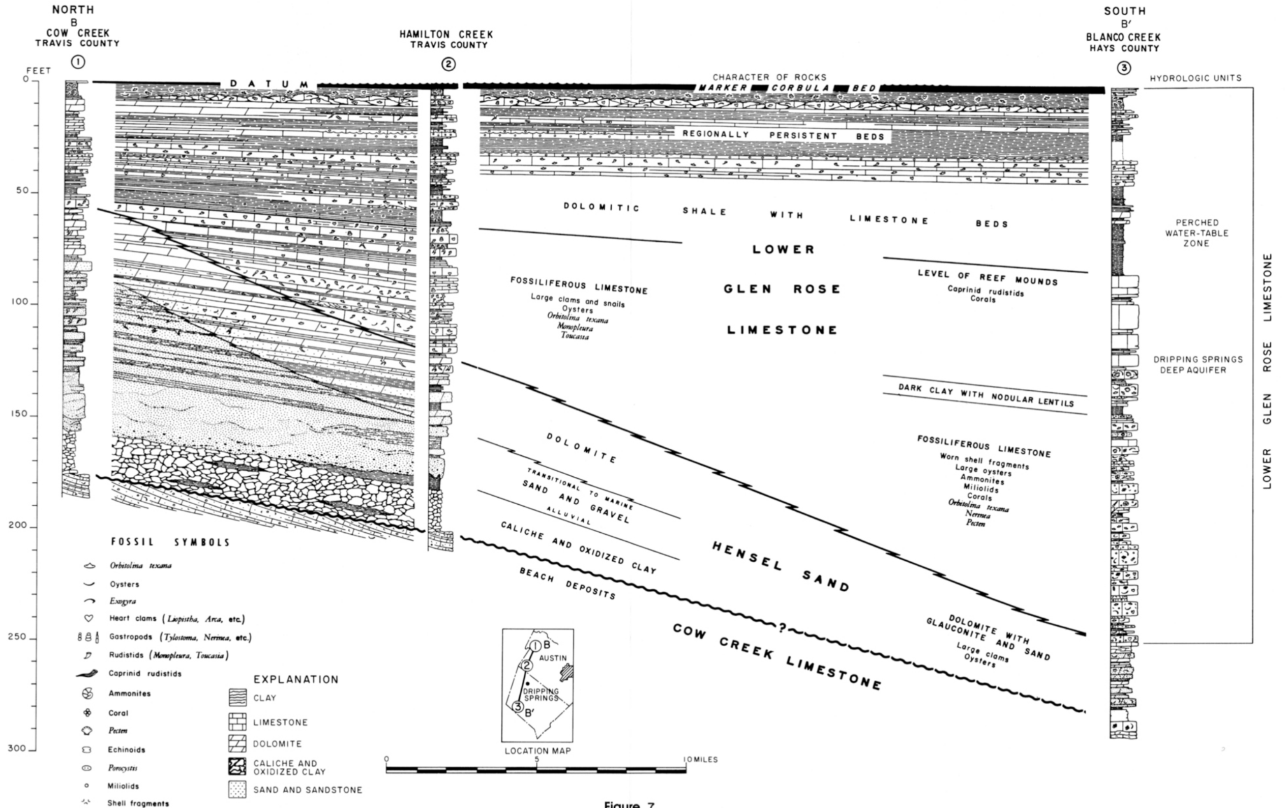
Figure 7 Geologic Strike Cross Section of the Lower Glen Rose Limestone
