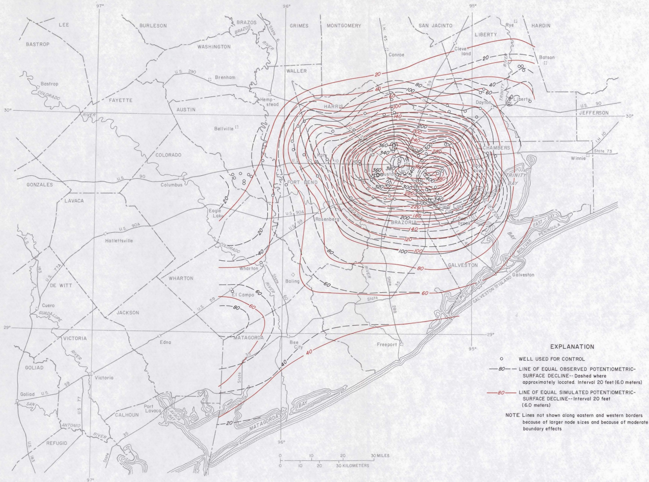
Figure 30 Observed and Simulated Declines in the Altitude of the Potentiometric Surface of the Evangeline Aquifer, Houston-Subregion Model, 1890-1973
