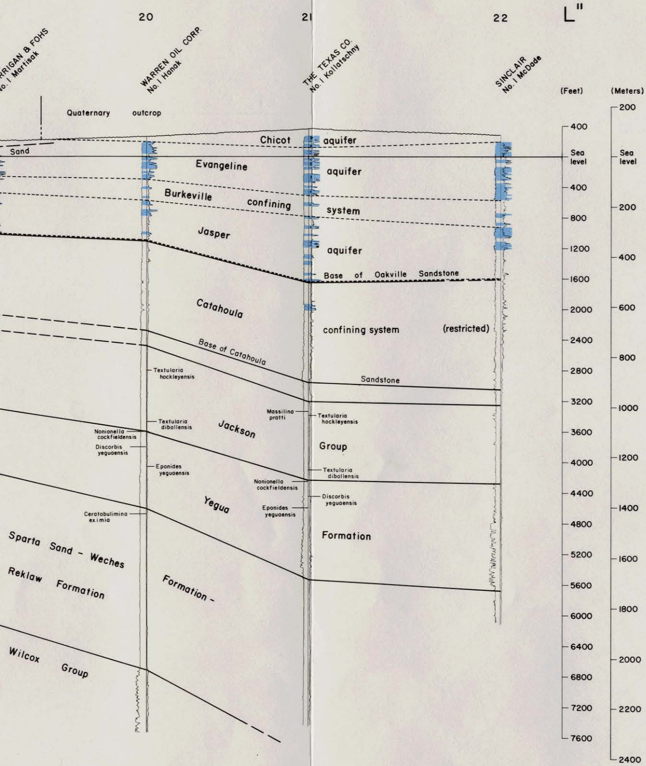
Geologic Section L'-L''
