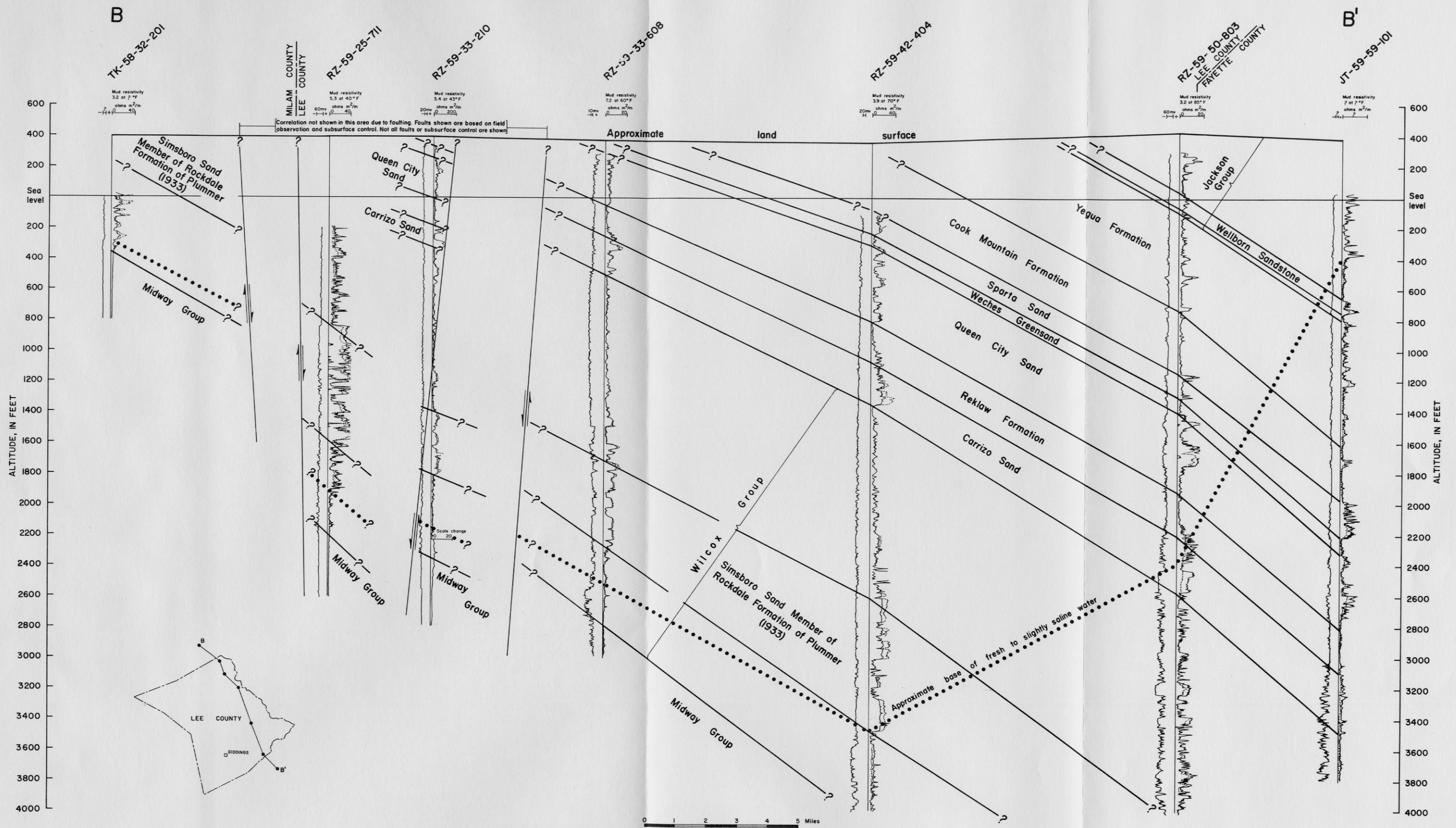
Plate 3 Geologic Section B-B', Milam, Lee, and Fayette Counties U. S. Geological Survey in cooperation with the Texas Water Development Board
