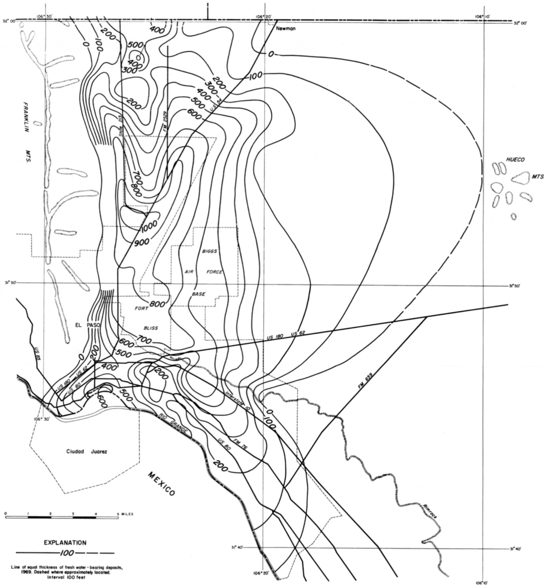
Figure 12 Approximate Saturated Thickness of Deposits Containing Fresh Water in the Hueco Bolson
