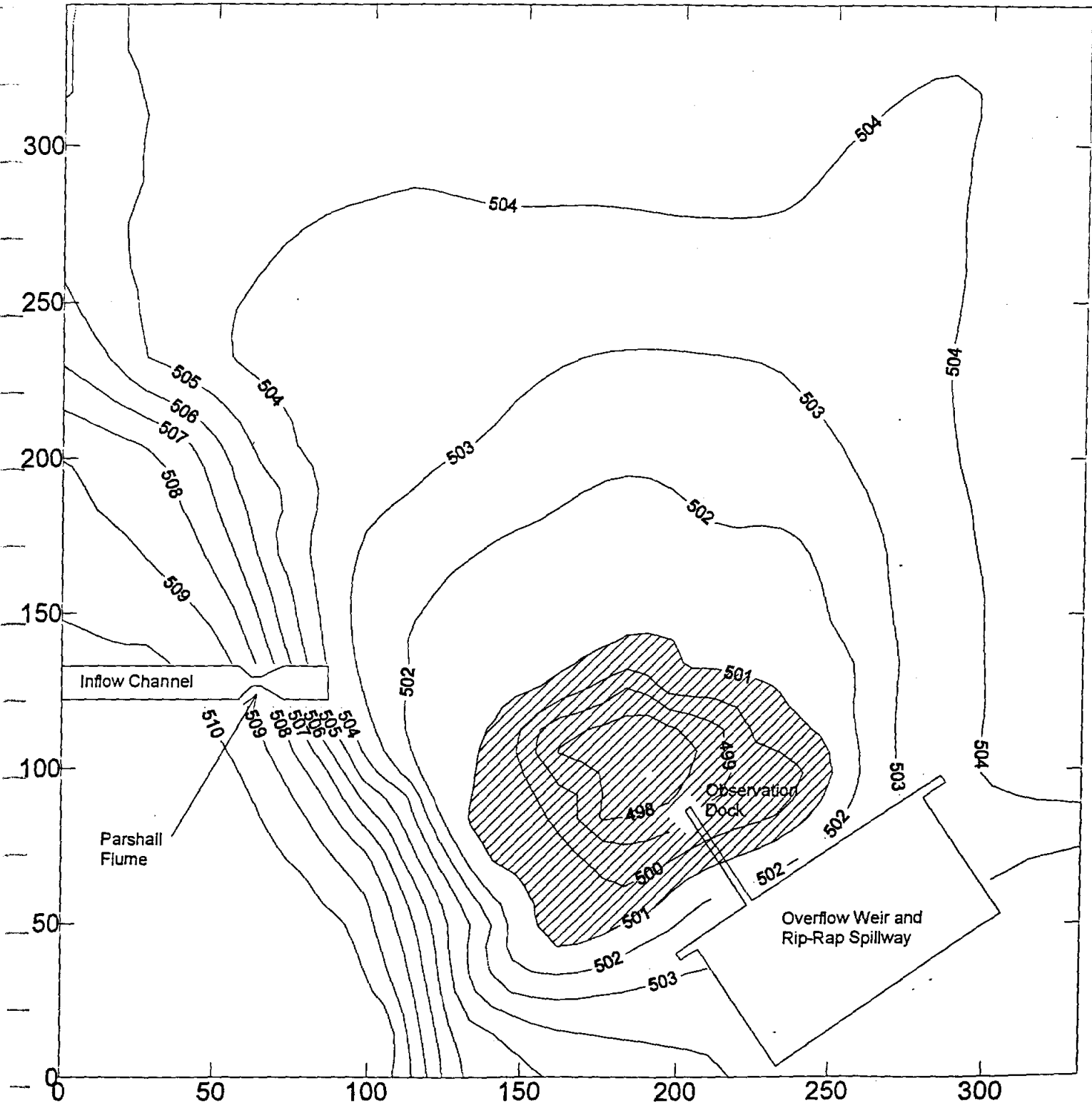
Figure 5 Mansfield Wetpond Bathymetric Survey, Nov. 5, 1996
