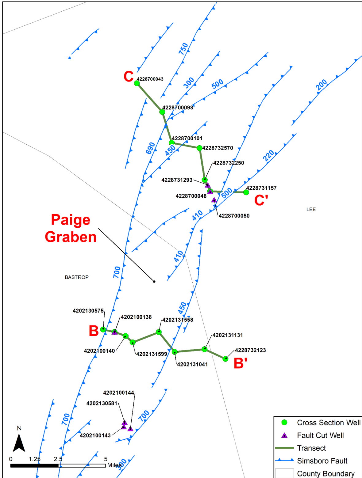
Figure 3.1.2.2a. Simsboro Formation faults and estimated fault offset (in feet) in the Paige Graben in Bastrop and Lee counties. Fault arrows point to the down-thrown side of the fault. The wells are labeled with their American Petroleum Institute number.
