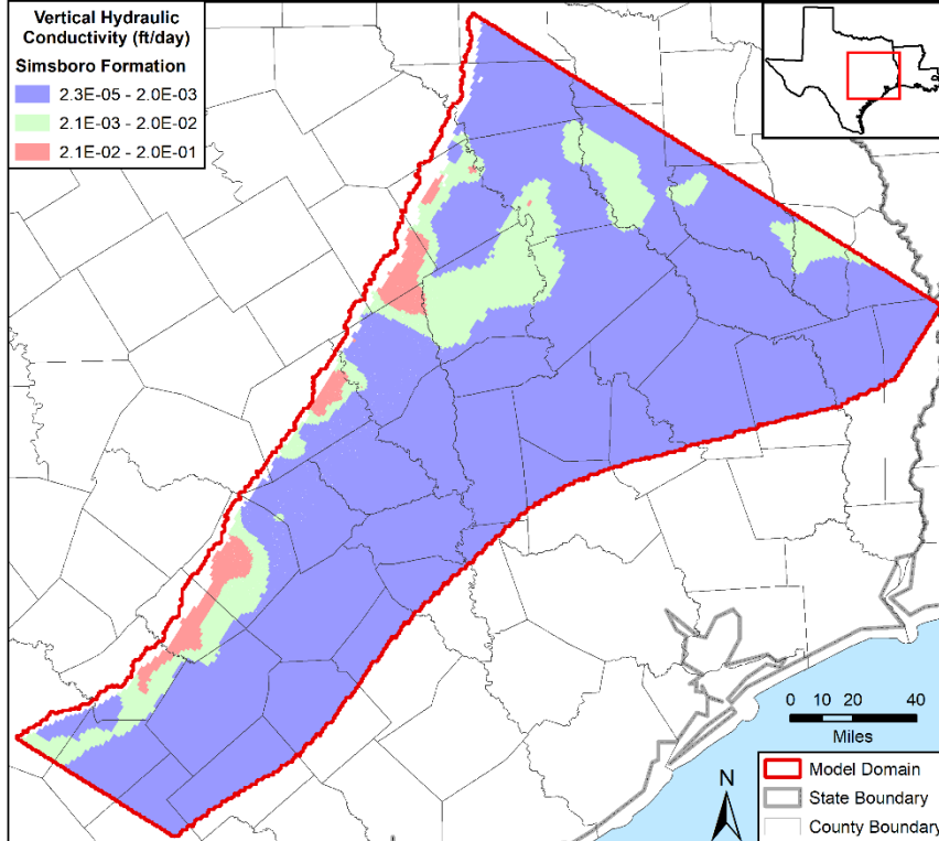
Figure 4.3.2r. Vertical hydraulic conductivity values in the calibrated model in feet per day (ft/day) for the Simsboro Formation in model layers 2 and 9.
