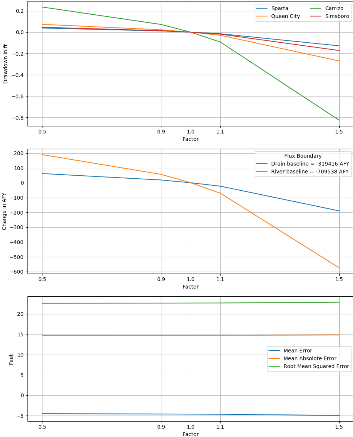
Figure 6.2.2m. Sensitivities of 2010 drawdown in hydrogeologic units (top), hydraulic boundary fluxes (center), and calibration statistics (bottom) to the specific storage of the Carrizo Aquifer for the transient model.
