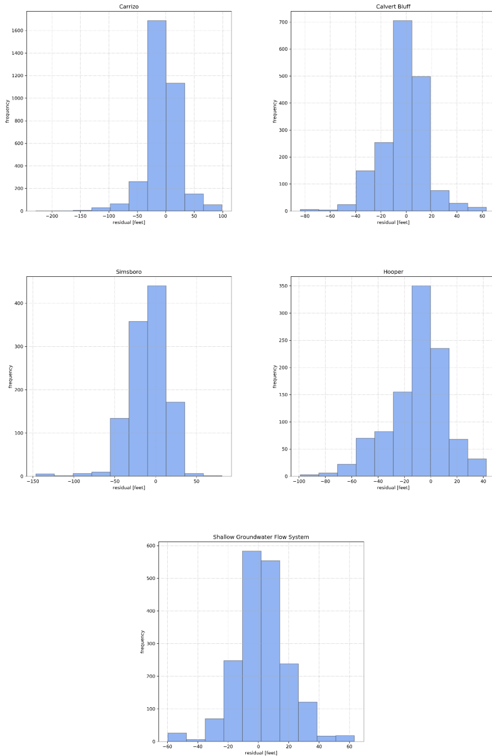
Figure 5.3.3I. Histograms of the hydraulic head residuals for all calibration targets in all wells in the Carrizo Aquifer, the Calvert Bluff Formation, the Simsboro Aquifer, the Hooper Aquifer, and the shallow groundwater flow system for the transient period 1930 to 2010.
