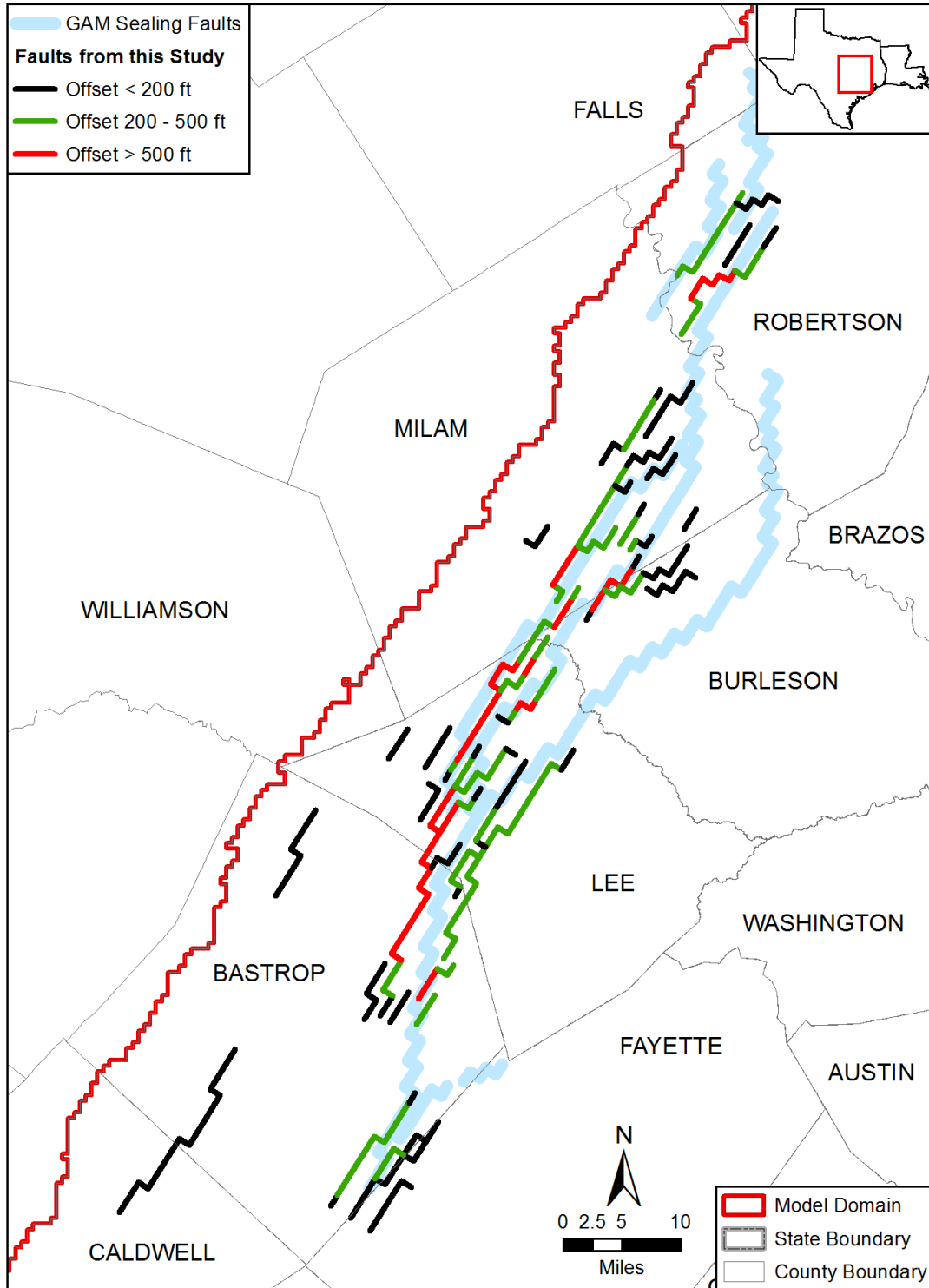
Figure 3.1.3a. Sealing faults in the groundwater availability model (GAM) for the central portion of the Carrizo-Wilcox, Queen City, and Sparta aquifers and the Simsboro Formation faults from this study sampled onto the groundwater availability model grid and color-coded based on the amount of offset between the Simsboro Formation updip and downdip of the fault.
