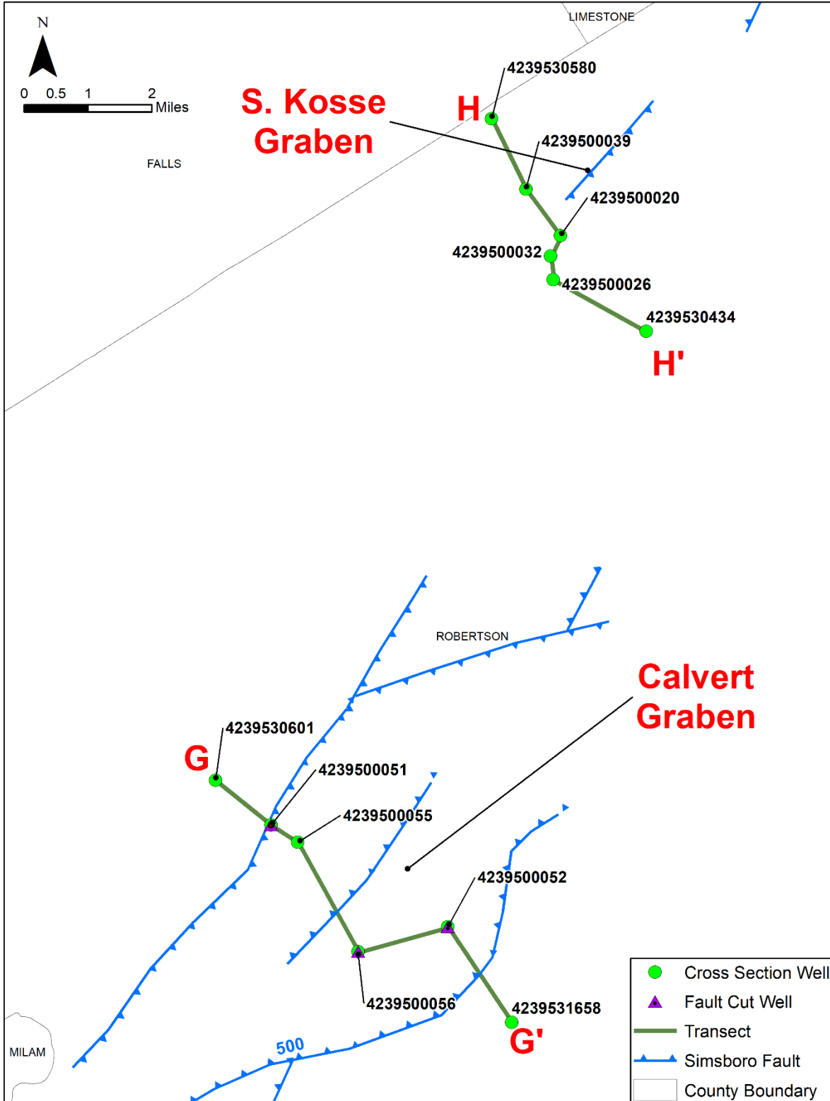
Figure 3.1.2.4a. Simsboro Formation faults and estimated fault offset (in feet) in the South (S.) Kosse and Calvert Grabens in Robertson County. Fault arrows point to the down-thrown side of the fault. The wells are labeled with their American Petroleum Institute number.
