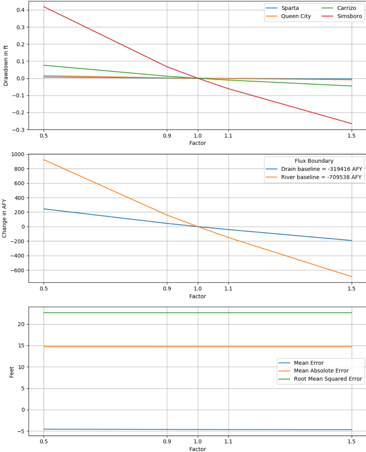
Figure 6.2.2p. Sensitivities of 2010 drawdown in hydrogeologic units (top), hydraulic boundary fluxes (center), and calibration statistics (bottom) to the specific yield of the Simsboro Formation for the transient model.
