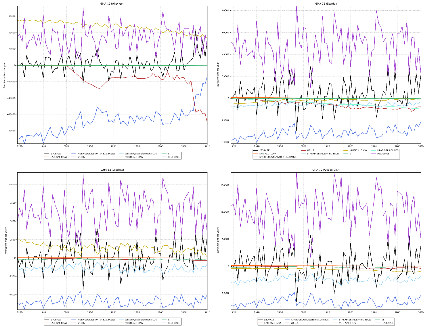
Figure 5.5.2j. Transient water budget for Groundwater Management Area 12 for the Colorado and Brazos rivers alluvium, Sparta Aquifer, Weches Formation, and Queen City Aquifer.
