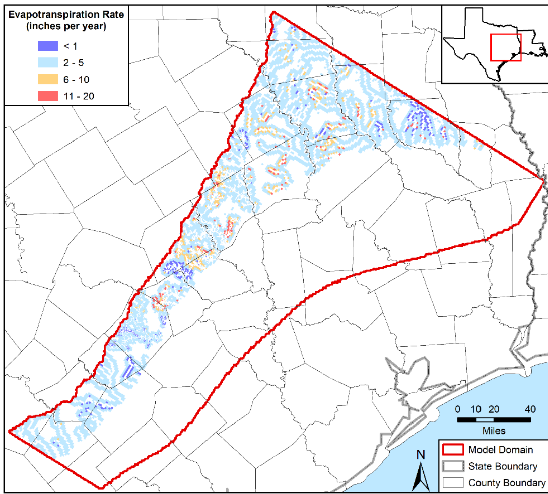
Figure 4.9a. Maximum evapotranspiration rate in inches per year for evapotranspiration cells.
