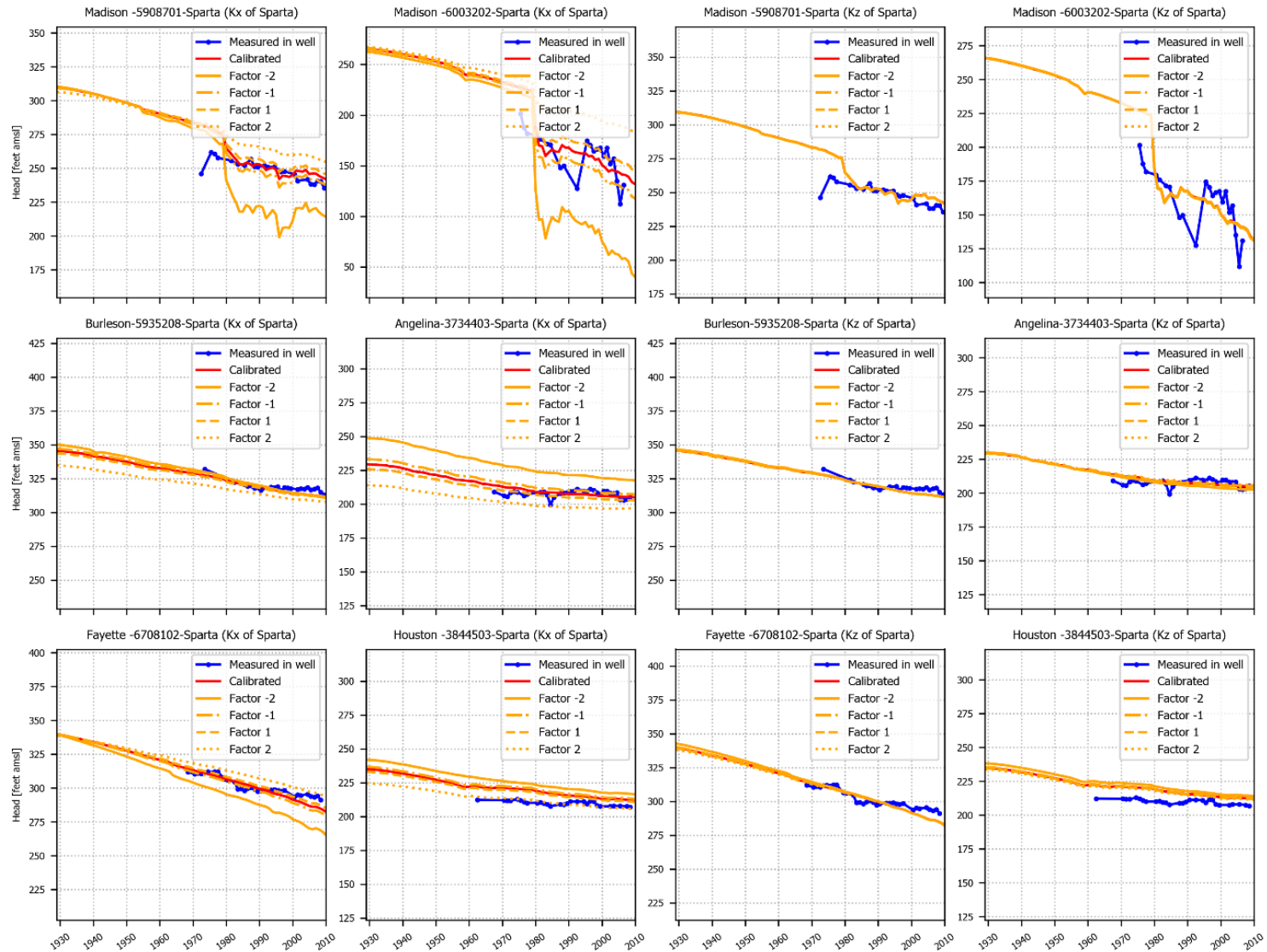
Figure 6.2.2u. Hydrographs showing sensitivity of heads (in feet above mean sea level) to changes in the horizontal and vertical hydraulic conductivity of the Sparta Aquifer for select wells completed in the Sparta Aquifer.
