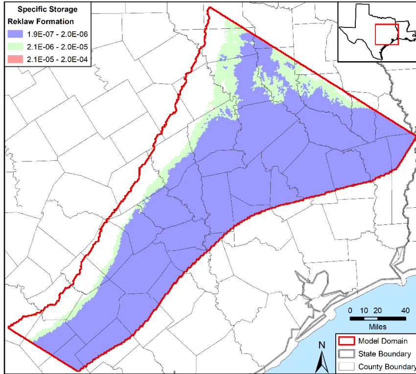
Figure 4.3.2y. Specific storage values in the calibrated model in feet -1 for the Reklaw Formation in model layers 2 and 6.
