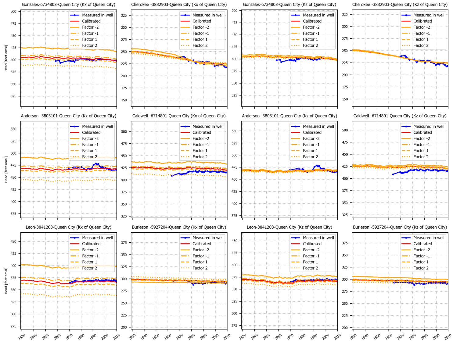
Figure 6.2.2v. Hydrographs showing sensitivity of heads (in feet above mean sea level) to changes in the horizontal and vertical hydraulic conductivity of the Queen City Aquifer for select wells completed in the Queen City Aquifer.
