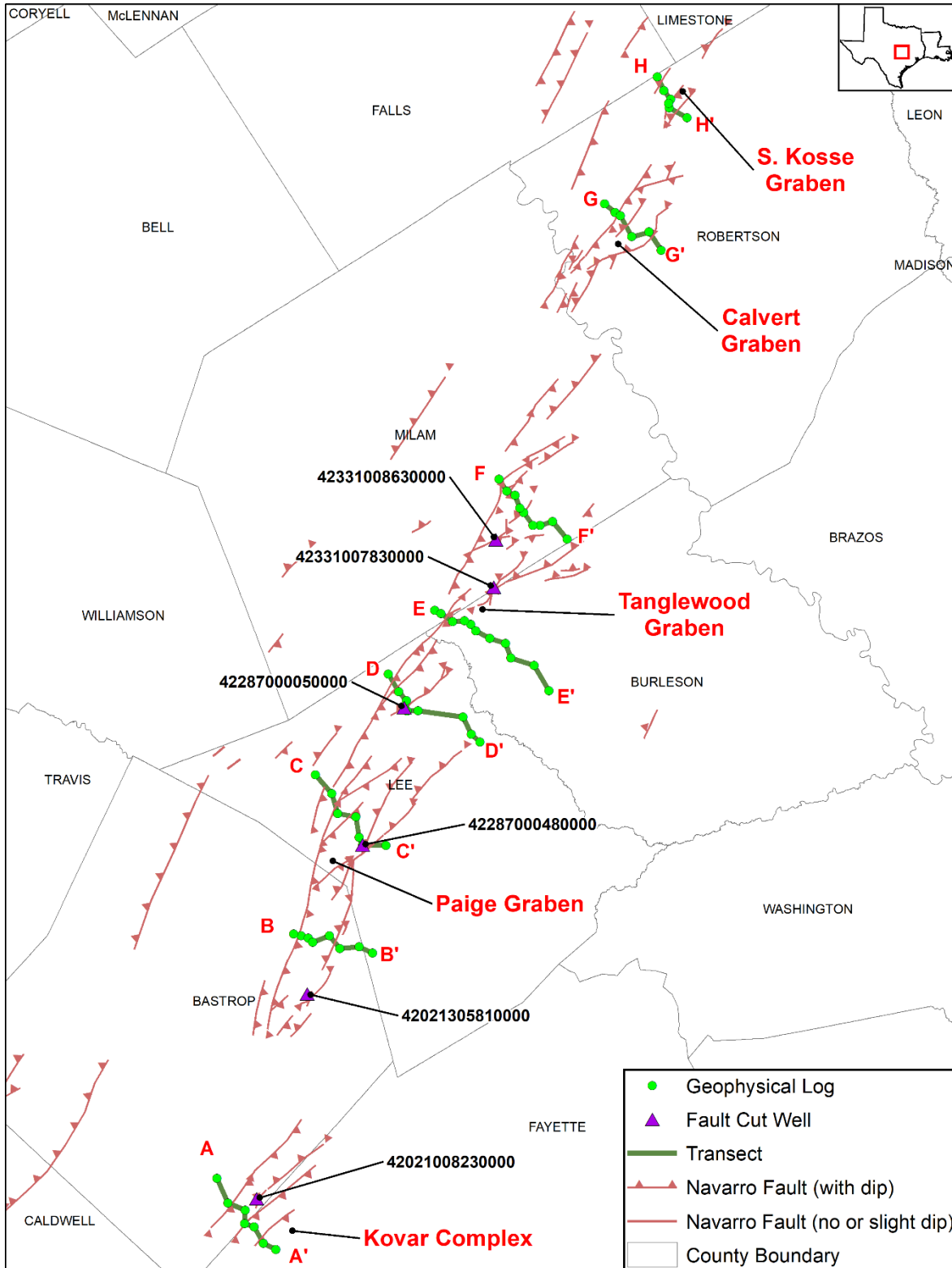
Figure 3.1.2g. Plan view map of the Milano Fault Zone showing the five named major areas of faulting, locations of cross-sections that transect the fault zone, and locations of fault cut wells shown in Figure 3.1.2d.
