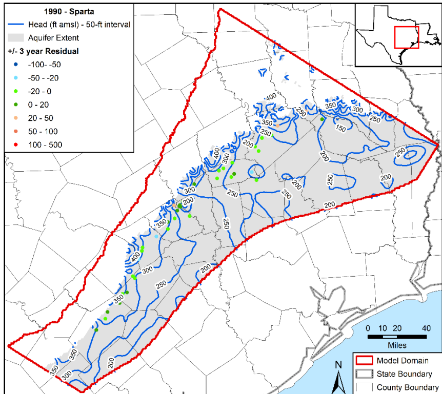
Figure 5.3.4i. Contours in feet (ft) above mean sea level (amsl) developed from simulated hydraulic heads for 1990 in the Sparta Aquifer with residuals posted.
