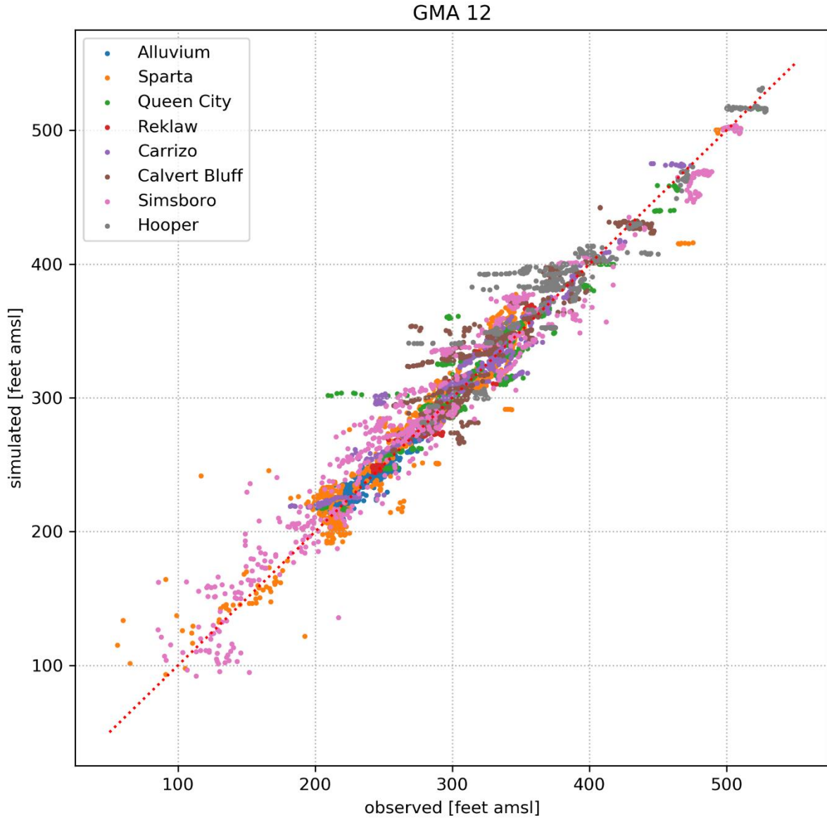
Figure 5.3.3h. Scatter plot of simulated versus observed hydraulic heads for the 4,767 water levels used as calibration targets in Groundwater Management Area 12 for the transient period 1930 to 2010.
