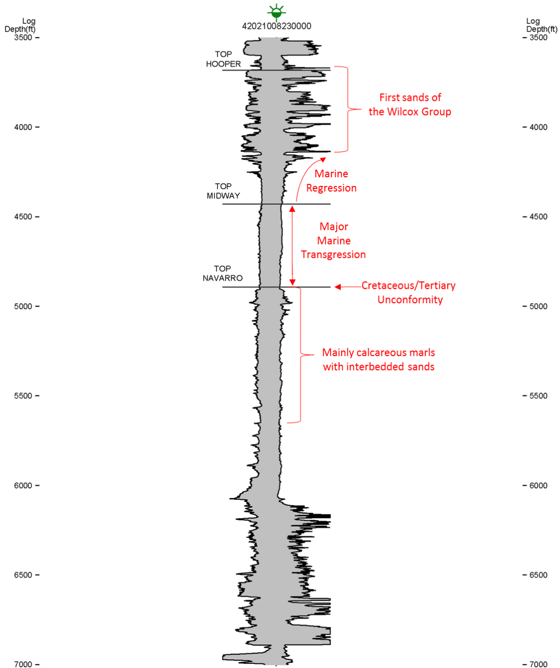
Figure 3.1.2a. Geophysical signature of the Navarro Group on both the spontaneous potential and resistivity logs.
