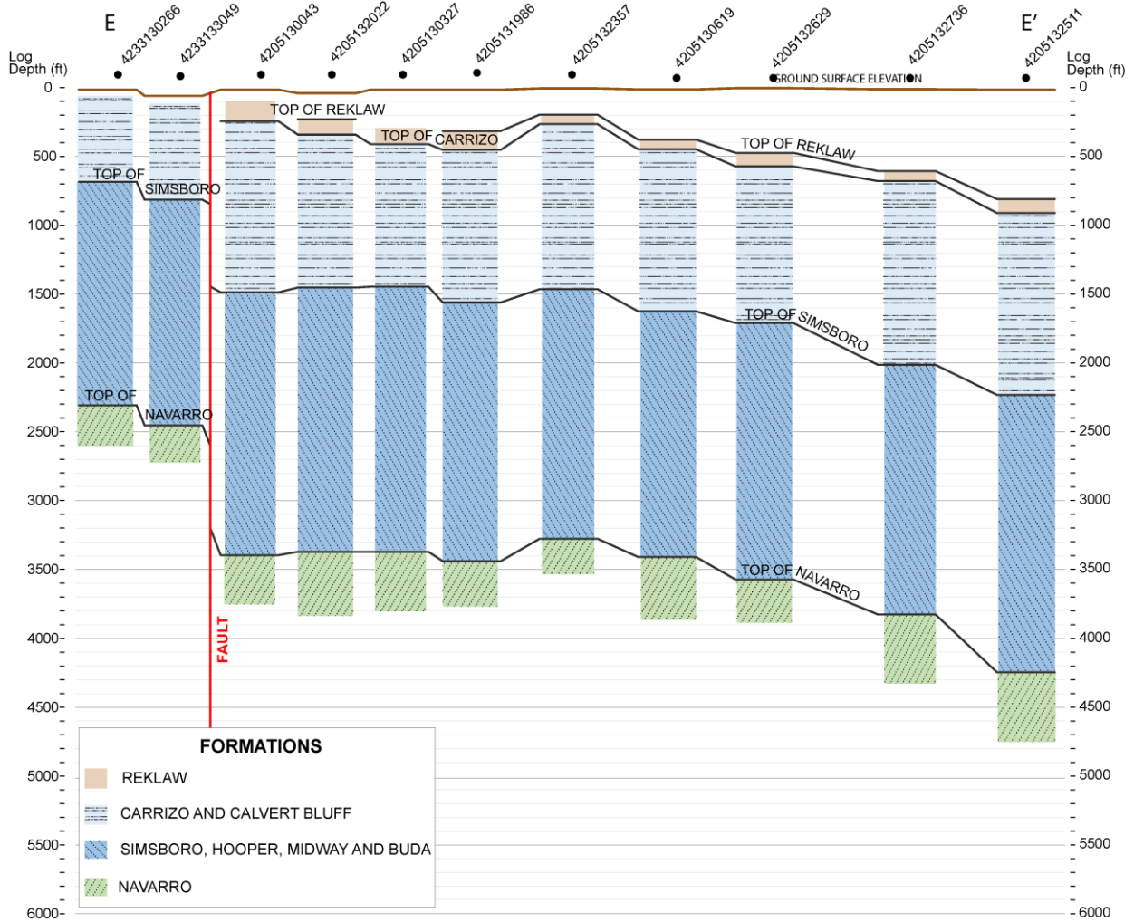
Figure 3.1.2.3c. Cross-section E-E' through the middle portion of the Tanglewood Graben showing the top surface of selected formations and mapped fault locations based on interpretation of geophysical logs in and near cross-section E-E'.
