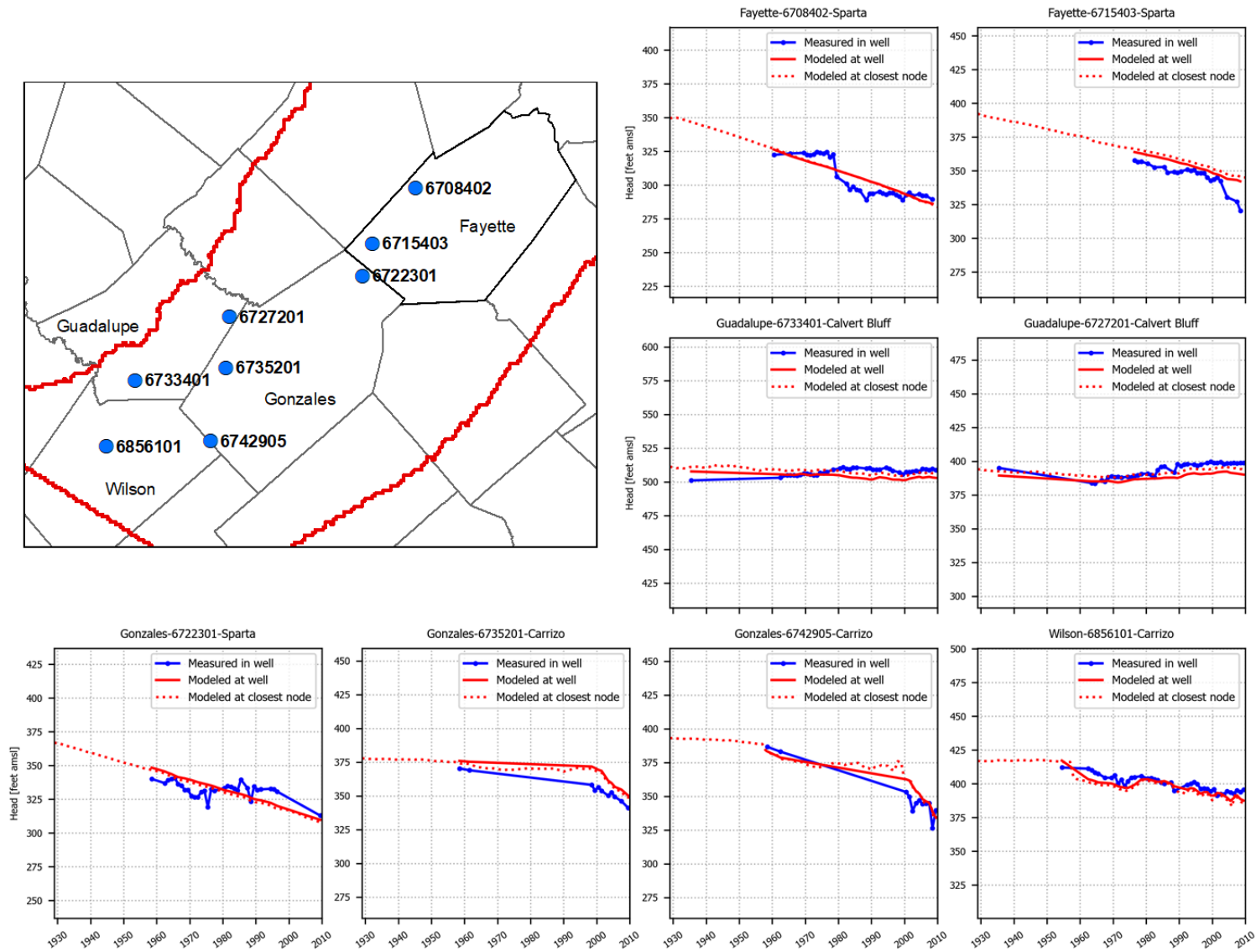
Figure 5.3.6i. Hydrographs showing simulated and measured hydraulic heads (in feet above mean sea level) in the Fayette County Groundwater Conservation District and Groundwater Management Area 13 at eight wells with state well numbers 6708402, 6715403, 6733401, 6727201, 6722301, 6735201, 6742905, and 6856101.
