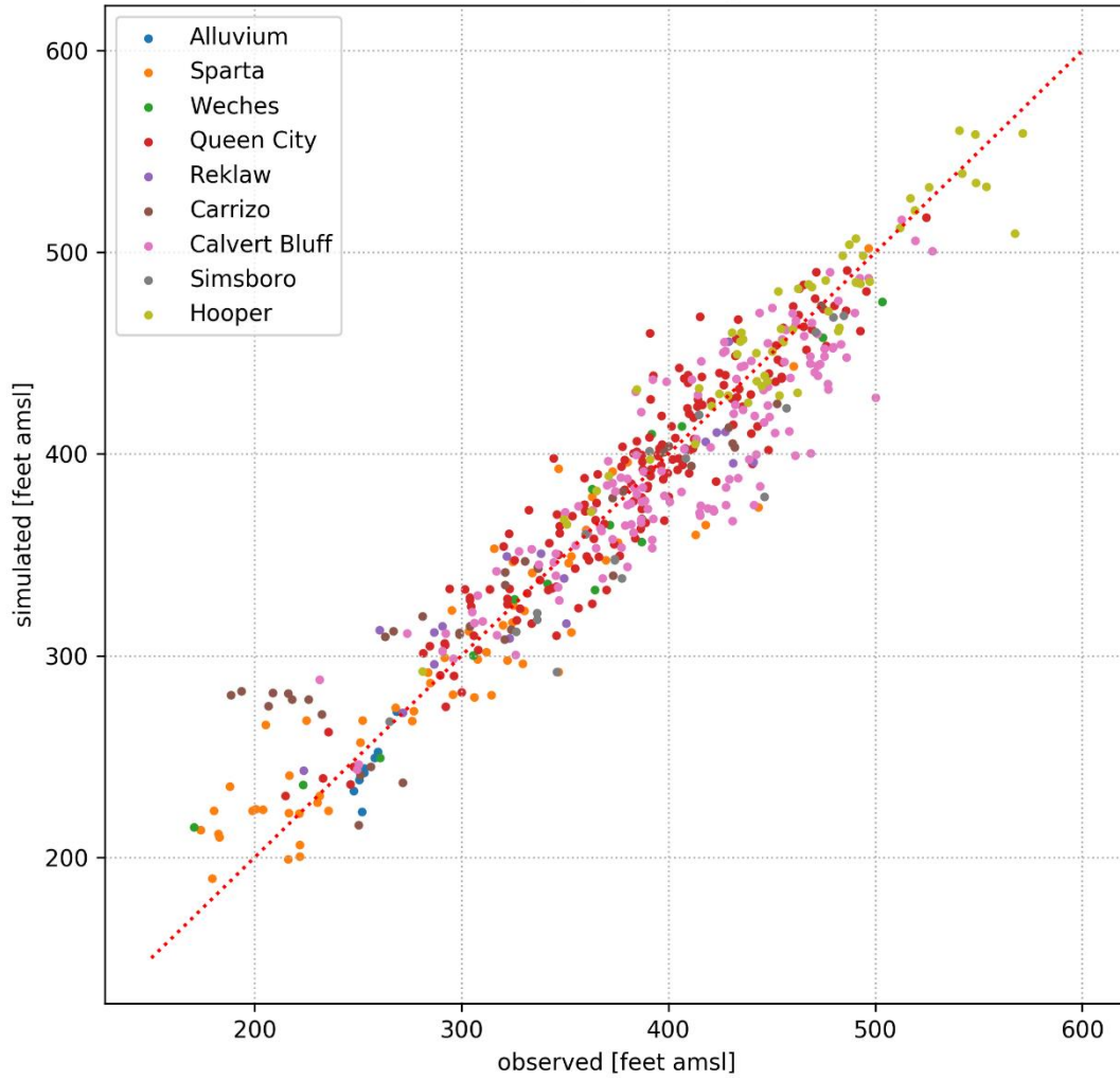
Figure 5.3.2a. Scatter plot of simulated versus observed hydraulic heads for 522 calibration targets across the entire model for the steady-state period.
