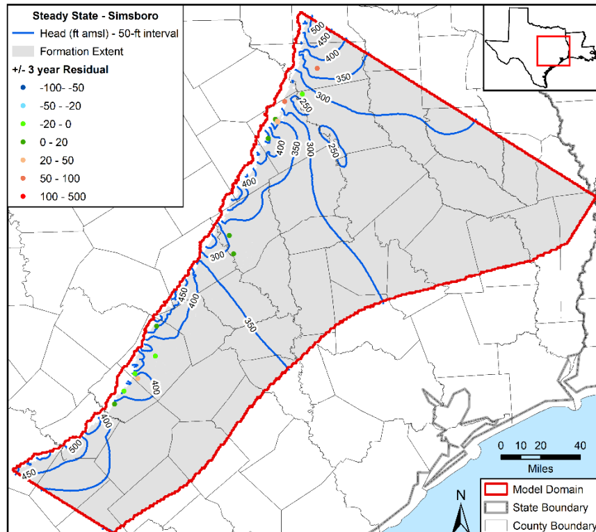
Figure 5.3.4jj. Contours in feet (ft) above mean sea level (amsl) developed from simulated hydraulic heads for steady-state conditions in the Simsboro Formation with residuals posted.
