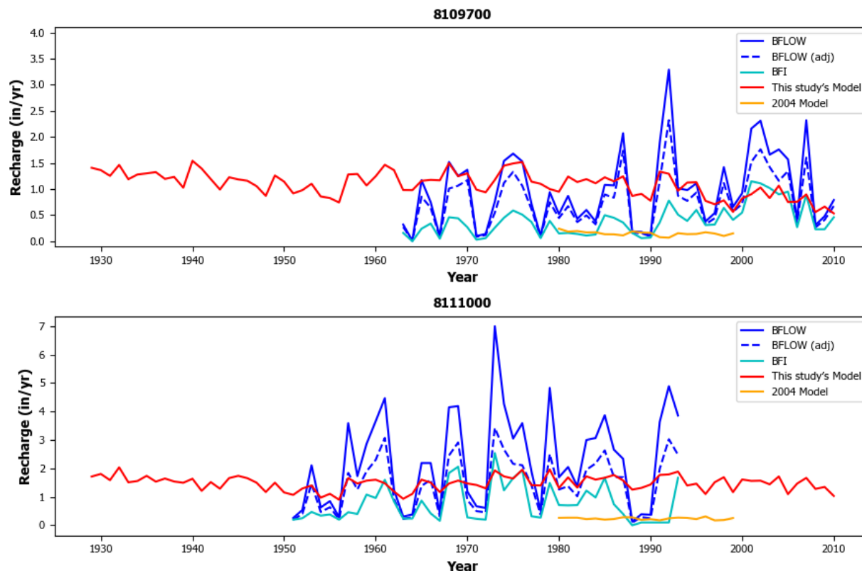
Figure 5.4.2b. Comparison of recharge rates (in inches per year) calculated from base flow for river gages 8109700 and 8111000 based on the Baseflow Program analysis and adjusted Baseflow Program values, the Base Flow Index Program analysis, and calculated from this study's model and the 2004 groundwater availability model by Kelley and others (2004). The model values equal the model calculated discharge to rivers/streams.
