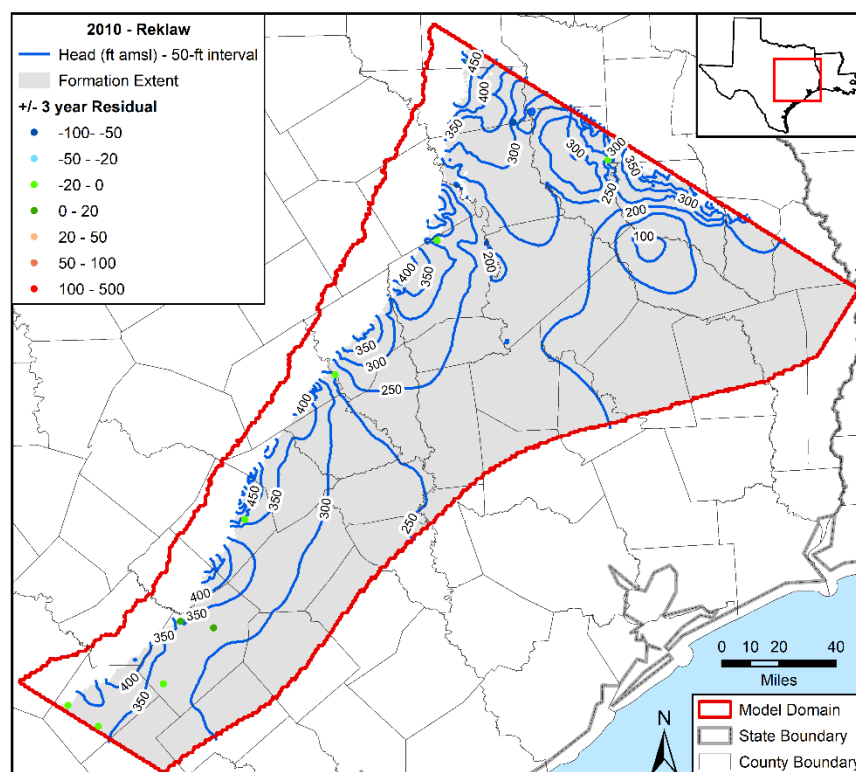
Figure 5.3.4y. Contours in feet (ft) above mean sea level (amsl) developed from simulated hydraulic heads for 2010 in the Reklaw Formation with residuals posted.
