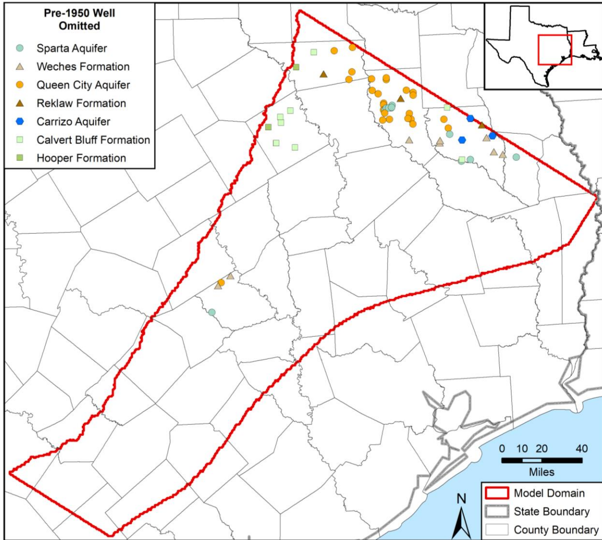
Figure 5.2b. Spatial distribution of wells with pre-1950 hydraulic heads that were not used as steady-state calibration targets because their head value was significantly different from the head value in nearby wells
