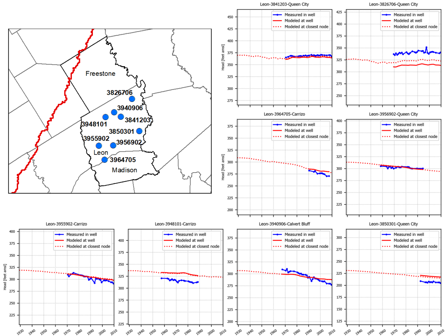
Figure 5.3.6h. Hydrographs showing simulated and measured hydraulic heads (in feet above mean sea level) in the Mid-East Texas Groundwater Conservation District at eight wells with state well numbers 3841203, 3826706, 3964705, 3956902, 3955902, 3948101, 3940906, and 3850301.
