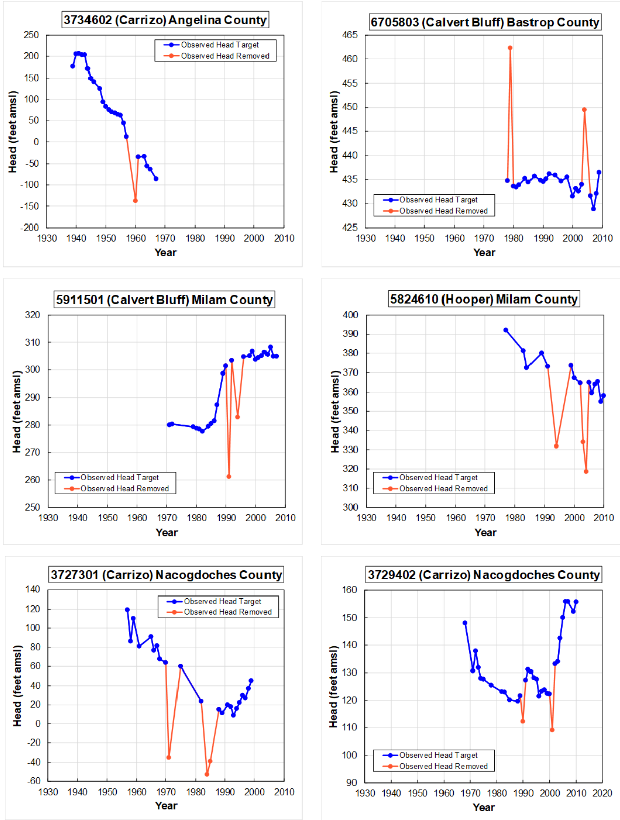
Figure 5.2c. Example of head measurements removed during development of transient calibration targets.
