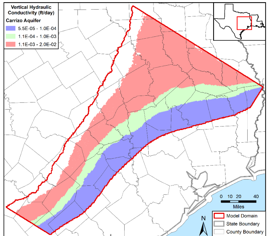
Figure 4.3.2p. Vertical hydraulic conductivity values in the calibrated model in feet per day (ft/day) for the Carrizo Aquifer in model layers 2 and 7.
