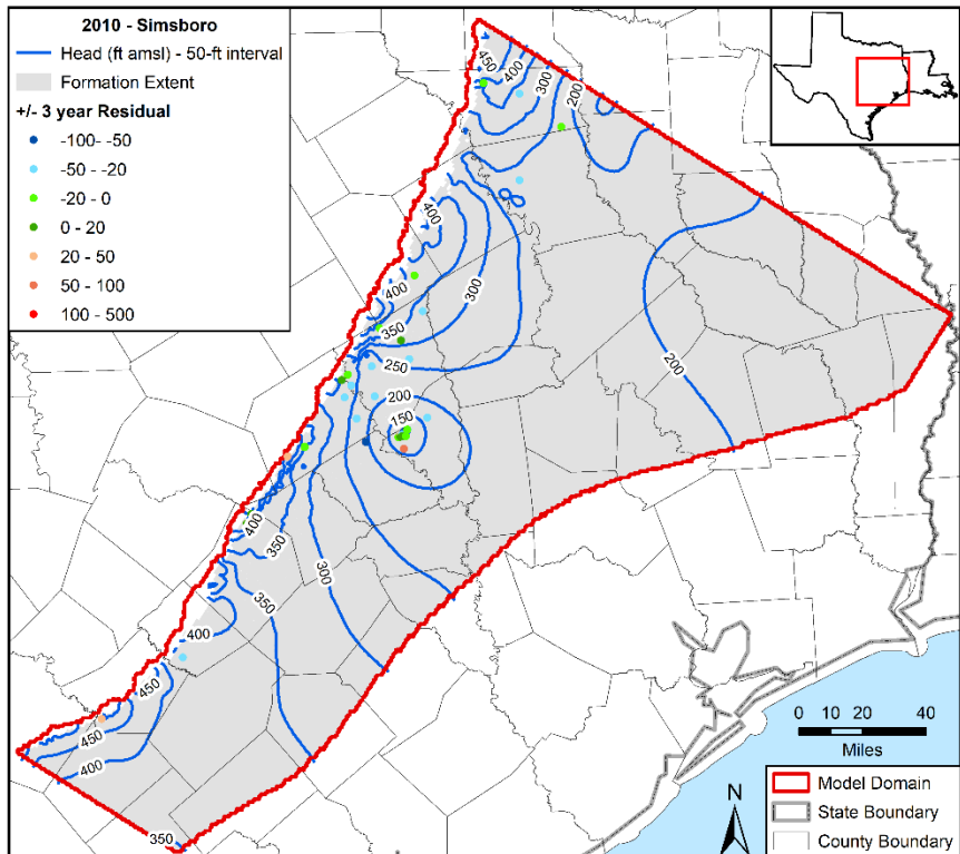
Figure 5.3.4nn. Contours in feet (ft) above mean sea level (amsl) developed from simulated hydraulic heads for 2010 in the Simsboro Formation with residuals posted.
