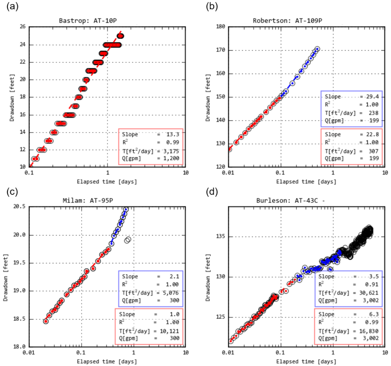
Figure 3.1.4.1b. Four example applications of the Cooper-Jacob analysis to calculate transmissivity for aquifer test classified as (a) “no change,” (b) “small decrease,” (c) “large decrease,” and (d) “increase” in calculated transmissivity values over time.
