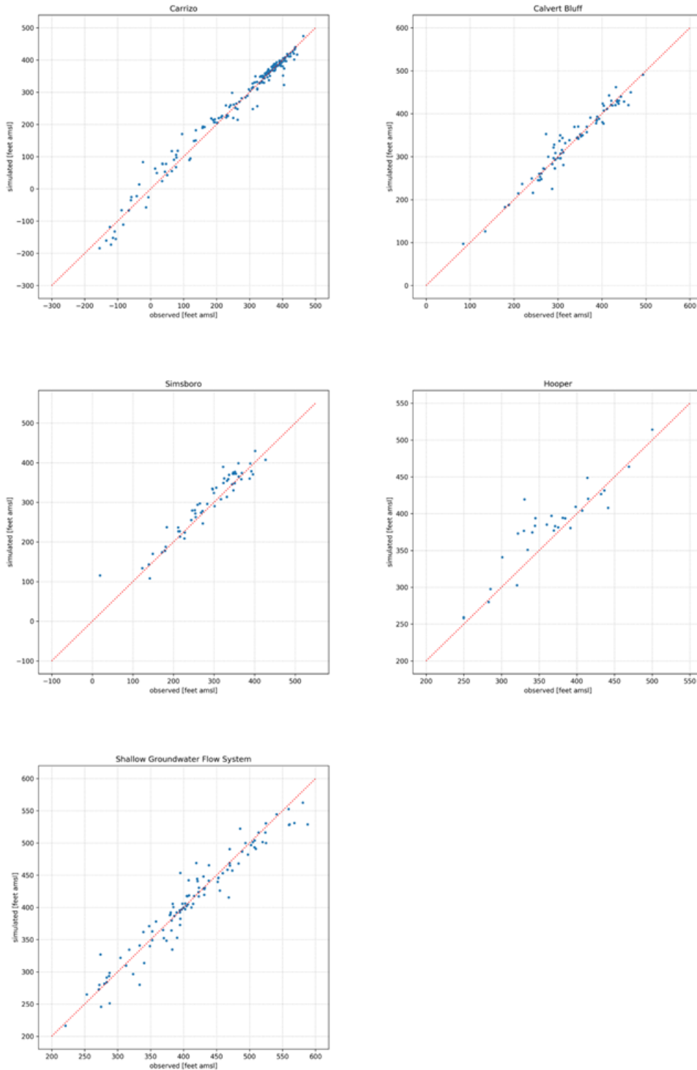
Figure 5.3.3d. Scatter plots of the average simulated versus average observed hydraulic heads at wells with calibration targets in the Carrizo Aquifer, the Calvert Bluff Formation, the Simsboro Formation, the Hooper Formation and the shallow groundwater flow system for the transient period 1930 to 2010.
