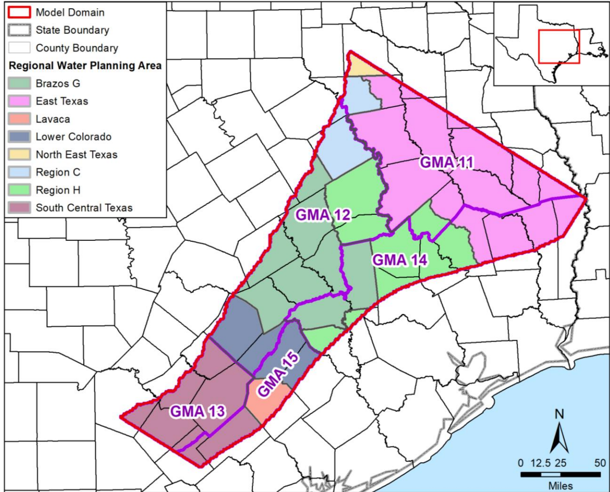
Figure 2.2d. Groundwater management areas (GMAs) and regional water planning areas in the active model area (TWDB, 2014a).
