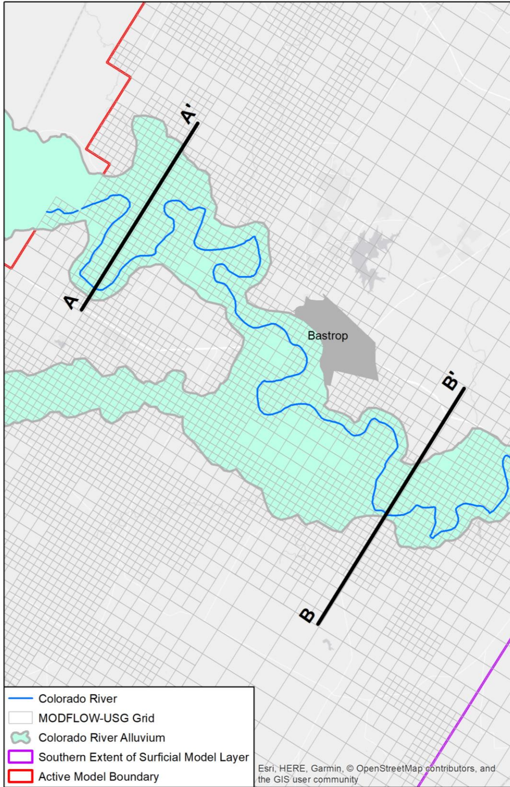
Figure 3.4.1a. Areal extent of the Colorado River alluvium mapped onto the numerical grid for the updated groundwater availability model for the central portion of the Carrizo-Wilcox, Queen City, and Sparta aquifers.
