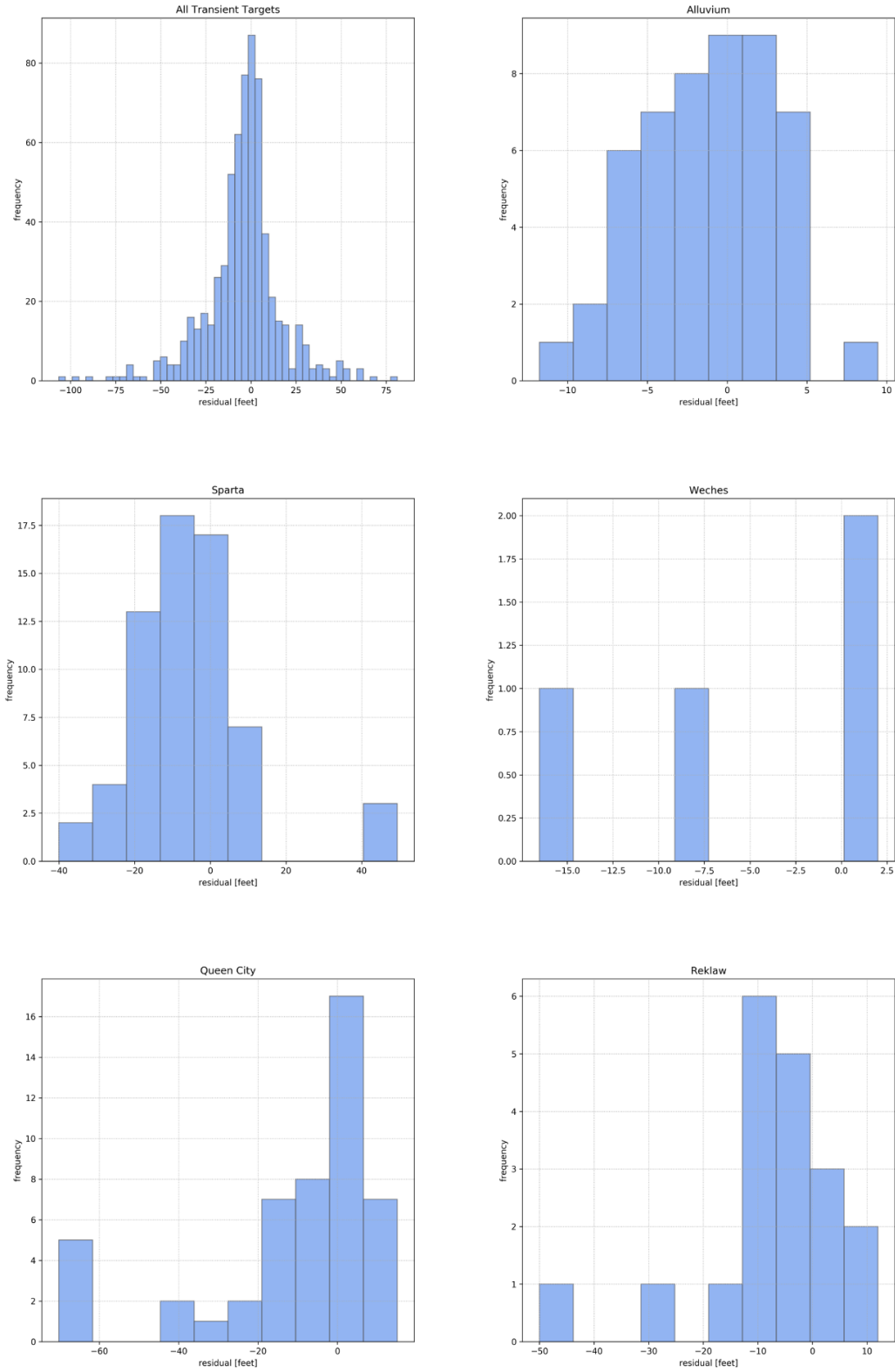
Figure 5.3.3e. Histograms of the average hydraulic head residuals for wells in the entire model domain, the Brazos River alluvium, the Sparta Aquifer, the Weches Formation, the Queen City Aquifer, and the Reklaw Formation for the transient period 1930 to 2010.
