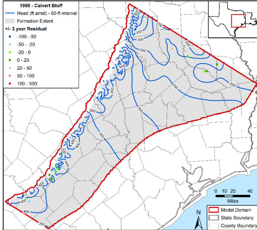
Figure 5.3.4ff. Contours in feet (ft) above mean sea level (amsl) developed from simulated hydraulic heads for 1950 in the Calvert Bluff Formation with residuals posted.
