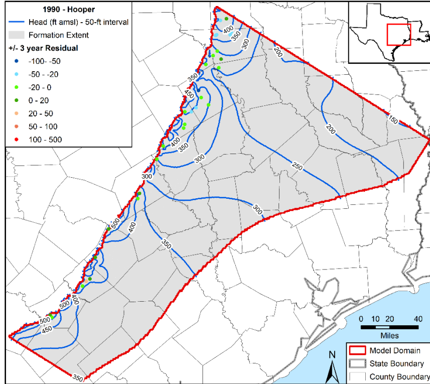
Figure 5.3.4rr. Contours in feet (ft) above mean sea level (amsl) developed from simulated hydraulic heads for 1990 in the Hooper Formation with residuals posted.
