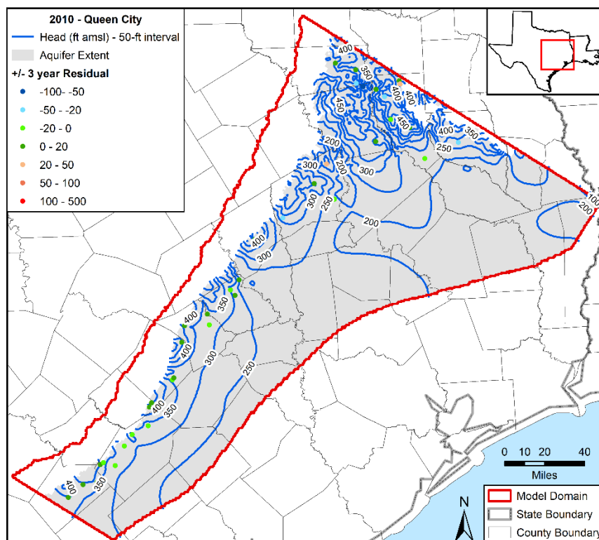
Figure 5.3.4t. Contours in feet (ft) above mean sea level (amsl) developed from simulated hydraulic heads for 2010 in the Queen City Aquifer with residuals posted.
