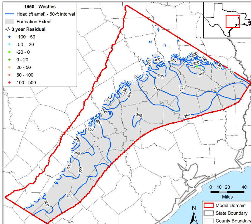
Figure 5.3.4l. Contours in feet (ft) above mean sea level (amsl) developed from simulated hydraulic heads for 1950 in the Weches Formation with residuals posted.
