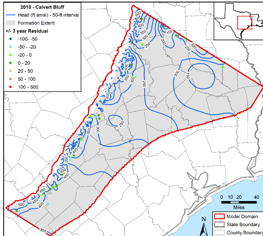
Figure 5.3.4ii. Contours in feet (ft) above mean sea level (amsl) developed from simulated hydraulic heads for 2010 in the Calvert Bluff Formation with residuals posted.
