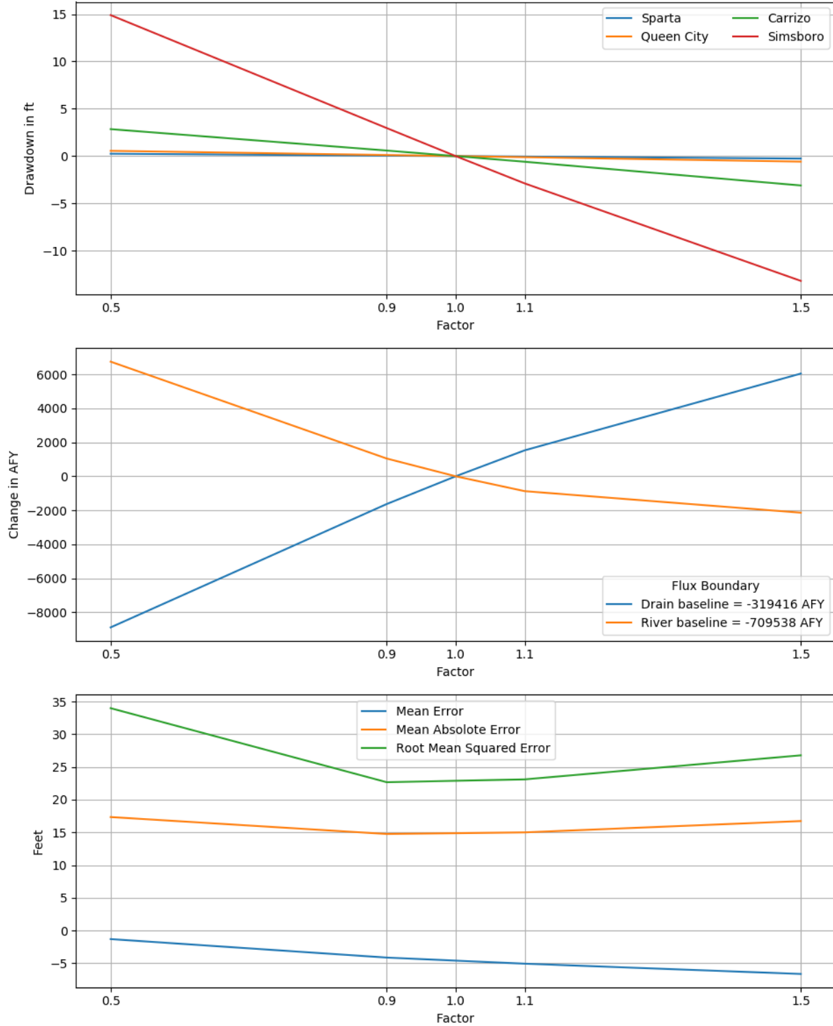
Figure 6.2.2g. Sensitivities of 2010 drawdown in hydrogeologic units (top), hydraulic boundary fluxes (center), and calibration statistics (bottom) to the horizontal hydraulic conductivity of the Simsboro Formation for the transient model.
