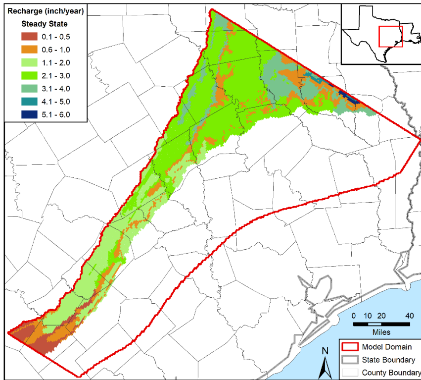
Figure 4.6a. Spatial distribution of recharge in inches per year for steady-state conditions.
