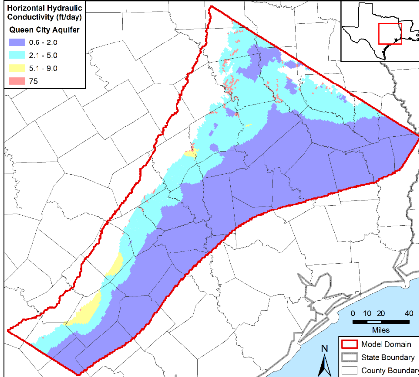
Figure 4.3.2d. Horizontal hydraulic conductivity values in the calibrated model in feet per day (ft/day) for the Queen City Aquifer in model layers 2 and 5.
