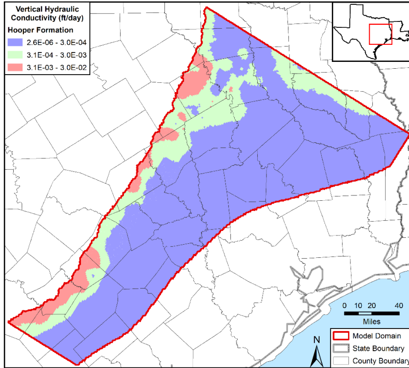
Figure 4.3.2s. Vertical hydraulic conductivity values in the calibrated model in feet per day (ft/day) for the Hooper Formation in model layers 2 and 10.
