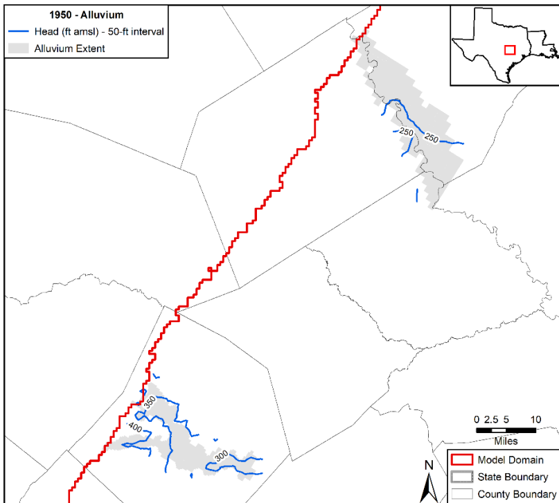
Figure 5.3.4b. Contours in feet (ft) above mean sea level (amsl) developed from simulated hydraulic heads for 1950 in the Colorado and Brazos rivers alluvium. No calibration targets available for this time.
