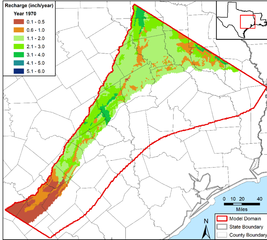
Figure 4.6c. Spatial distribution of recharge in inches per year for 1970.
