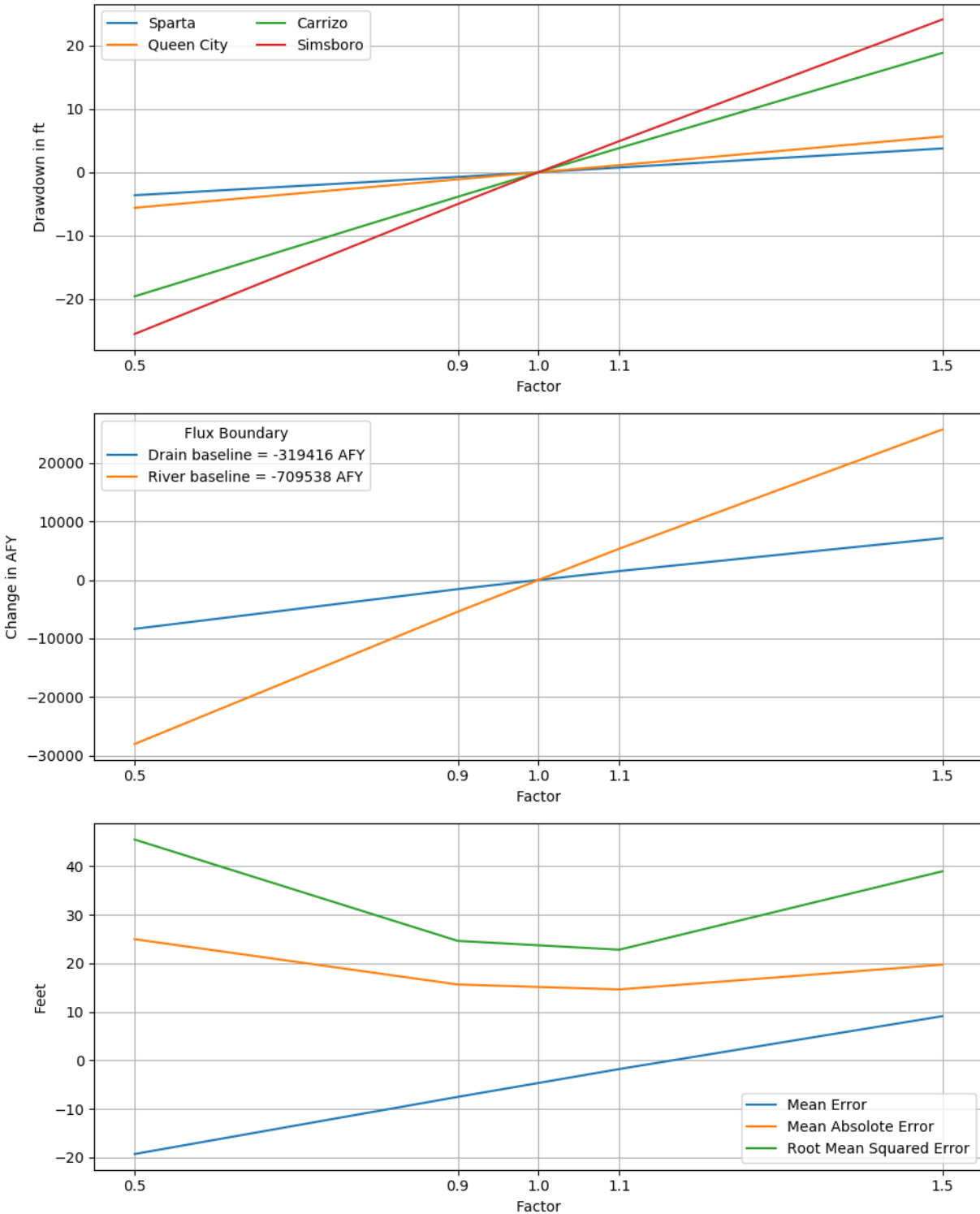
Figure 6.2.2t. Sensitivities of 2010 drawdown in hydrogeologic units (top), hydraulic boundary fluxes (center), and calibration statistics (bottom) to the pumping rate for the transient model.
