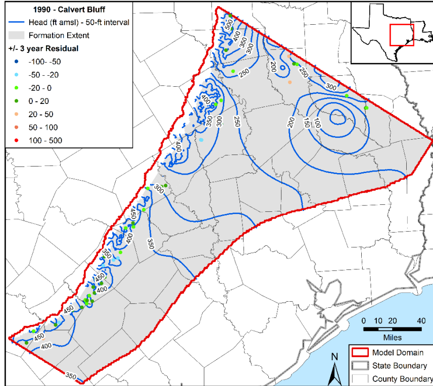
Figure 5.3.4hh. Contours in feet (ft) above mean sea level (amsl) developed from simulated hydraulic heads for 1990 in the Calvert Bluff Formation with residuals posted.
