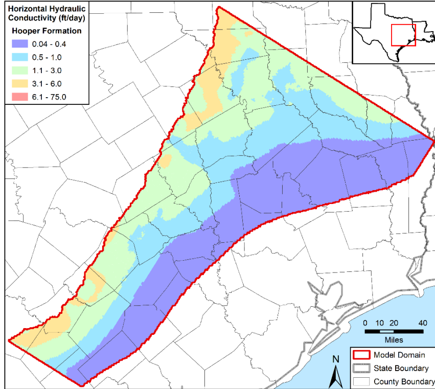
Figure 4.3.2i. Horizontal hydraulic conductivity values in the calibrated model in feet per day (ft/day) for the Hooper Formation in model layers 2 and 10.
