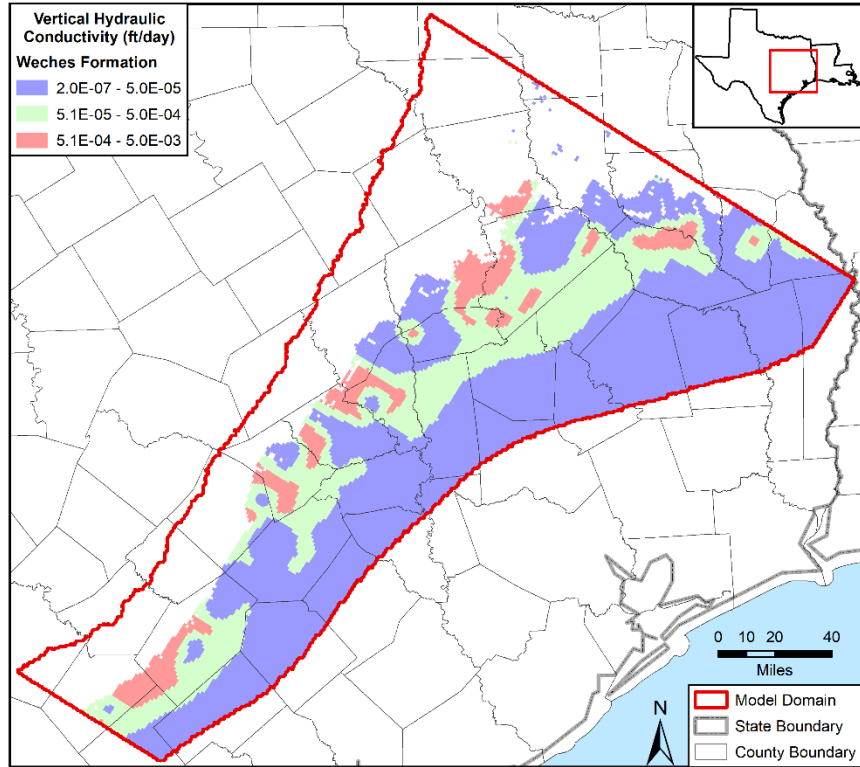
Figure 4.3.2m. Vertical hydraulic conductivity values in the calibrated model in feet per day (ft/day) for the Weches Formation in model layers 2 and 4.
