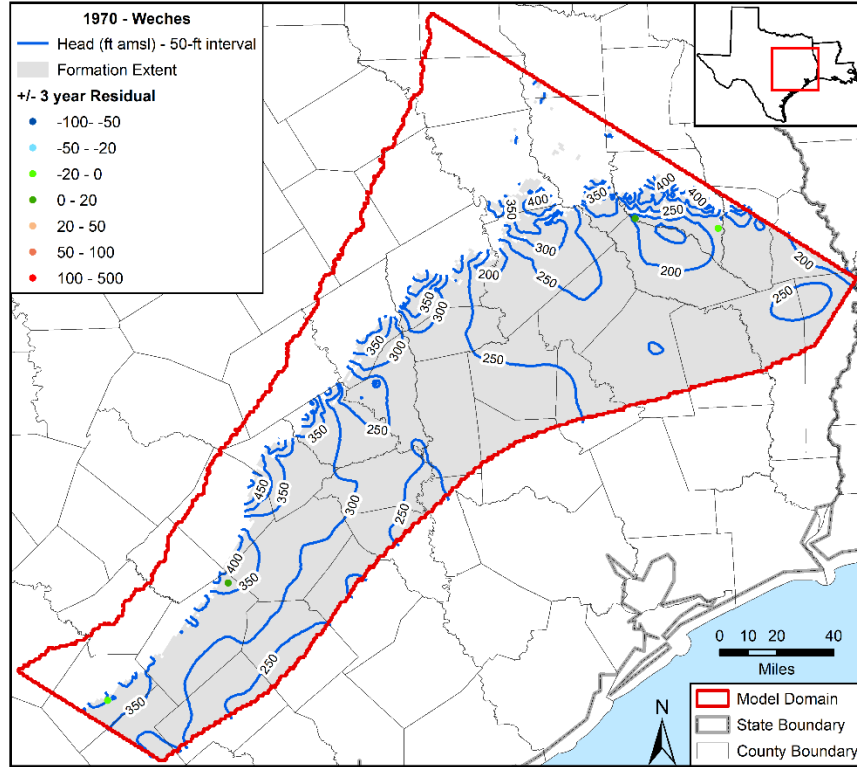
Figure 5.3.4m. Contours in feet (ft) above mean sea level (amsl) developed from simulated hydraulic heads for 1970 in the Weches Formation with residuals posted.
