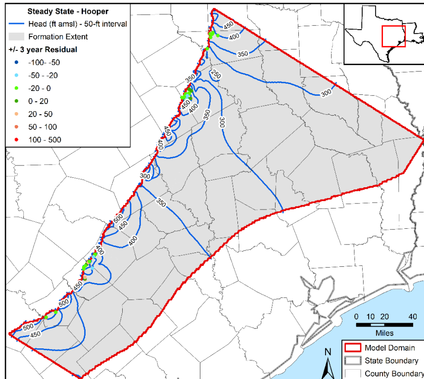
Figure 5.3.4oo. Contours in feet (ft) above mean sea level (amsl) developed from simulated hydraulic heads for steady-state conditions in the Hooper Formation with residuals posted.
