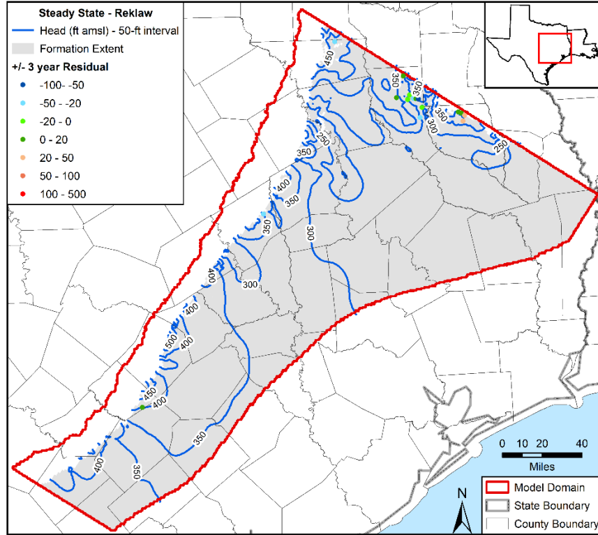
Figure 5.3.4u. Contours in feet (ft) above mean sea level (amsl) developed from simulated hydraulic heads for steady-state conditions in the Reklaw Formation with residuals posted.
