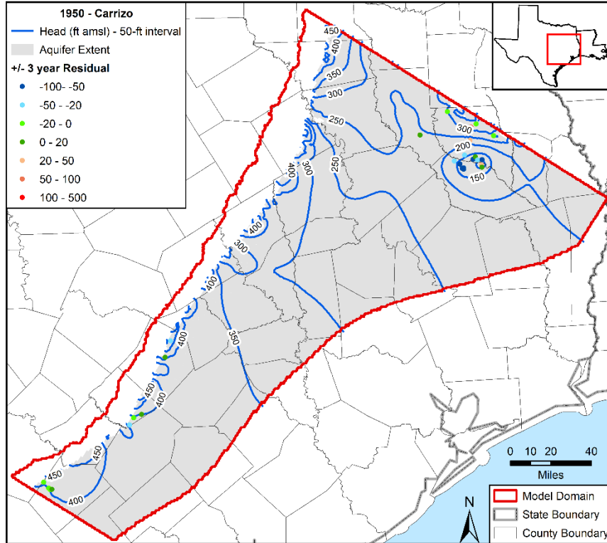
Figure 5.3.4aa. Contours in feet (ft) above mean sea level (amsl) developed from simulated hydraulic heads for 1950 in the Carrizo Aquifer with residuals posted.
