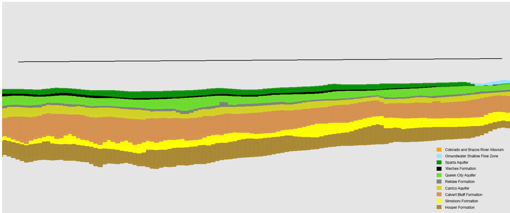
Figure 4.2.10. Vertical cross-section showing the model layers along strike cross-section C-C'.
