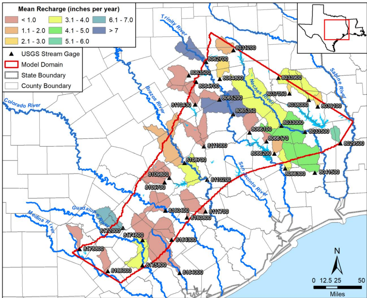
Figure 3.3.3a. Long-term average annual recharge calculated from hydrograph separation using the Base Flow Index Program.
