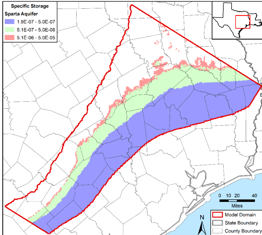
Figure 4.3.2v. Specific storage values in the calibrated model in feet -1 for the Sparta Aquifer in model layers 2 and 3.
