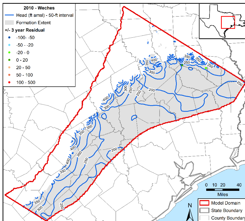
Figure 5.3.4o. Contours in feet (ft) above mean sea level (amsl) developed from simulated hydraulic heads for 2010 in the Weches Formation with residuals posted.
