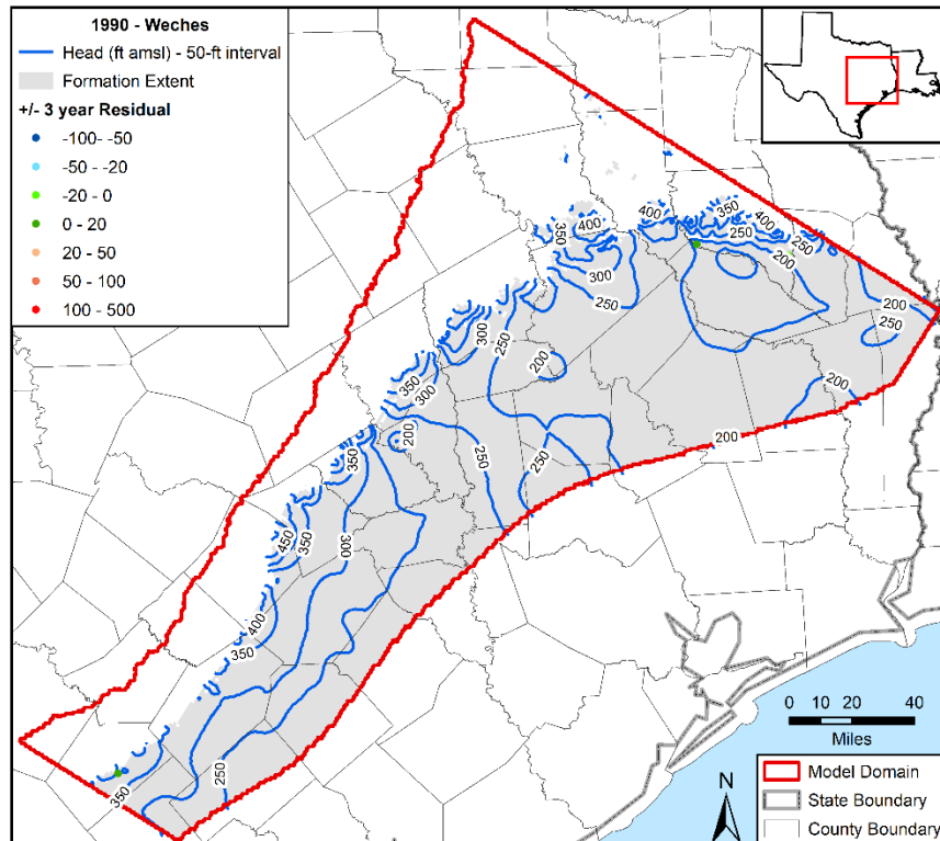
Figure 5.3.4n. Contours in feet (ft) above mean sea level (amsl) developed from simulated hydraulic heads for 1990 in the Weches Formation with residuals posted.
