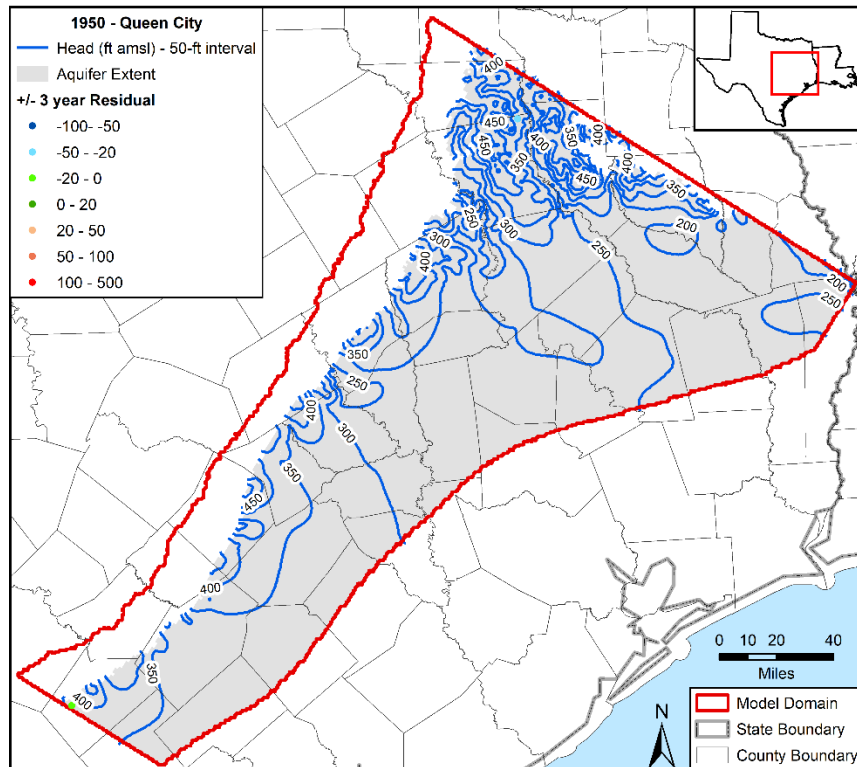
Figure 5.3.4q. Contours in feet (ft) above mean sea level (amsl) developed from simulated hydraulic heads for 1950 in the Queen City Aquifer with residuals posted.
