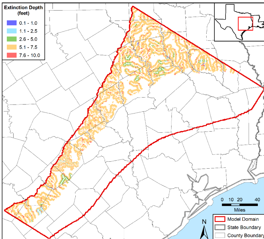
Figure 4.9b. Extinction depth in feet for evapotranspiration cells.
