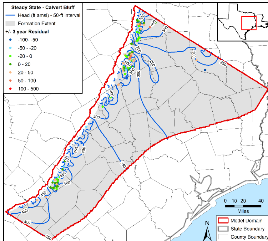
Figure 5.3.4ee. Contours in feet (ft) above mean sea level (amsl) developed from simulated hydraulic heads for steady-state conditions in the Calvert Bluff Formation with residuals posted.
