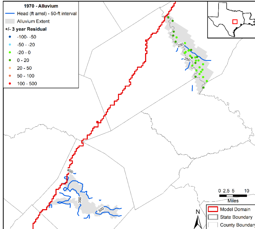
Figure 5.3.4c. Contours in feet (ft) above mean sea level (amsl) developed from simulated hydraulic heads for 1970 in the Colorado and Brazos rivers alluvium with residuals for the Brazos River alluvium posted.
