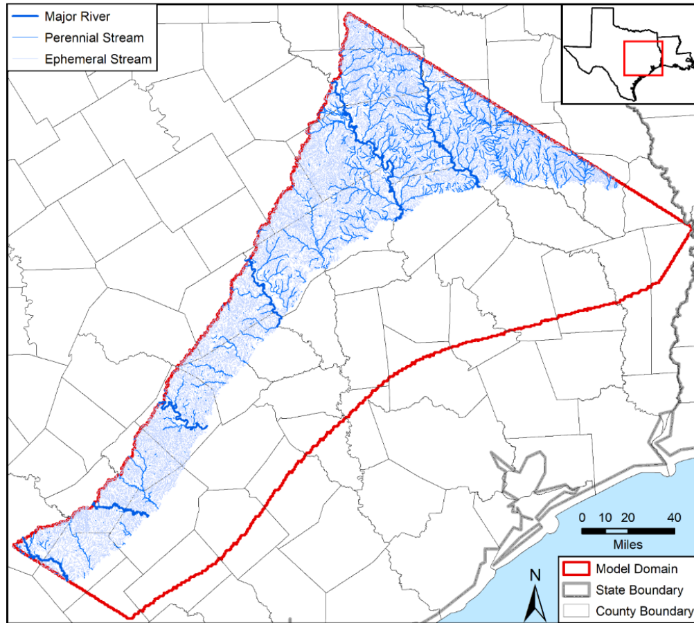
Figure 4.5a. Locations of major rivers and perennial and ephemeral streams in the outcrop areas based on United States Geological Survey national hydrograph data.
