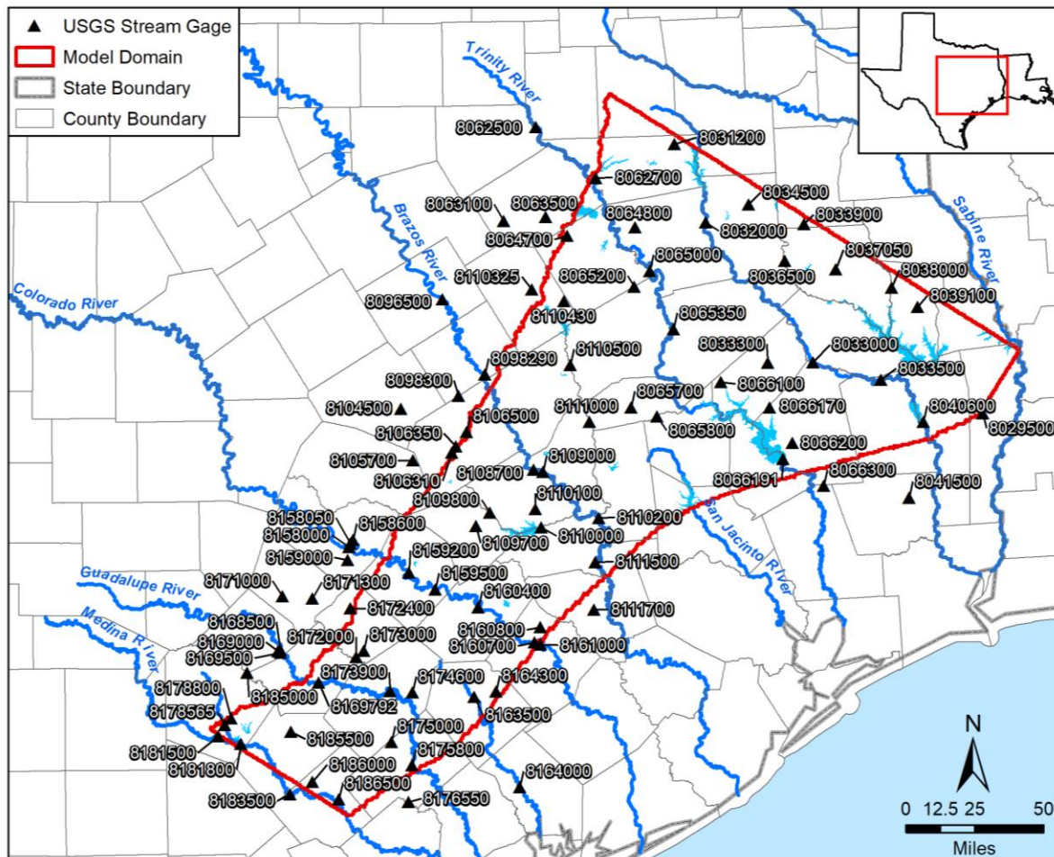
Figure 3.3.2.1a. Location of the 55 United States Geologic Survey (USGS) river gages considered for analysis using hydrograph separation to calculate base flow.
