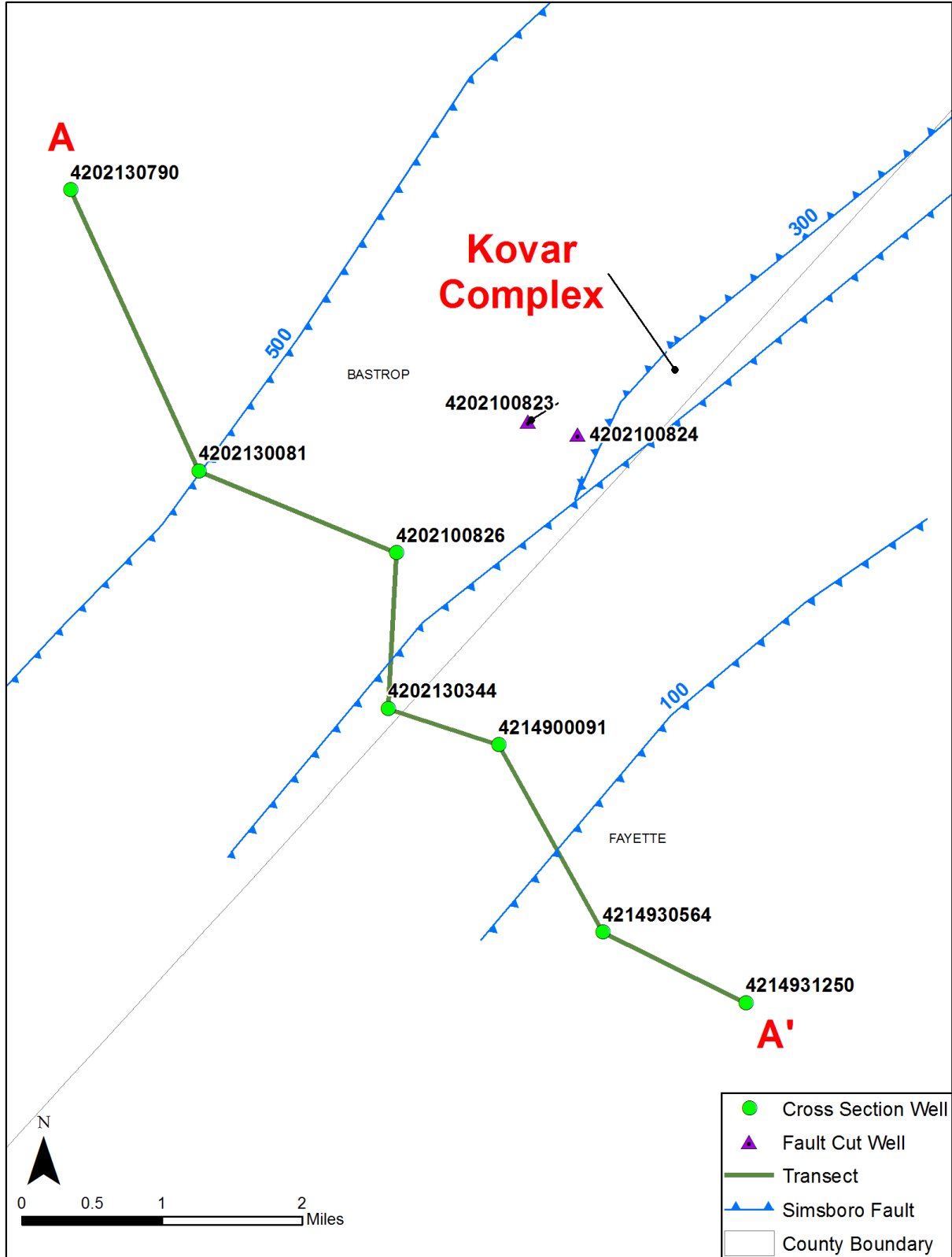
Figure 3.1.2.1a. Simsboro Formation faults and estimated fault offset (in feet) in the Kovar Complex in Bastrop and Fayette counties. Fault arrows point to the down-thrown side of the fault. The wells are labeled with their American Petroleum Institute number.
