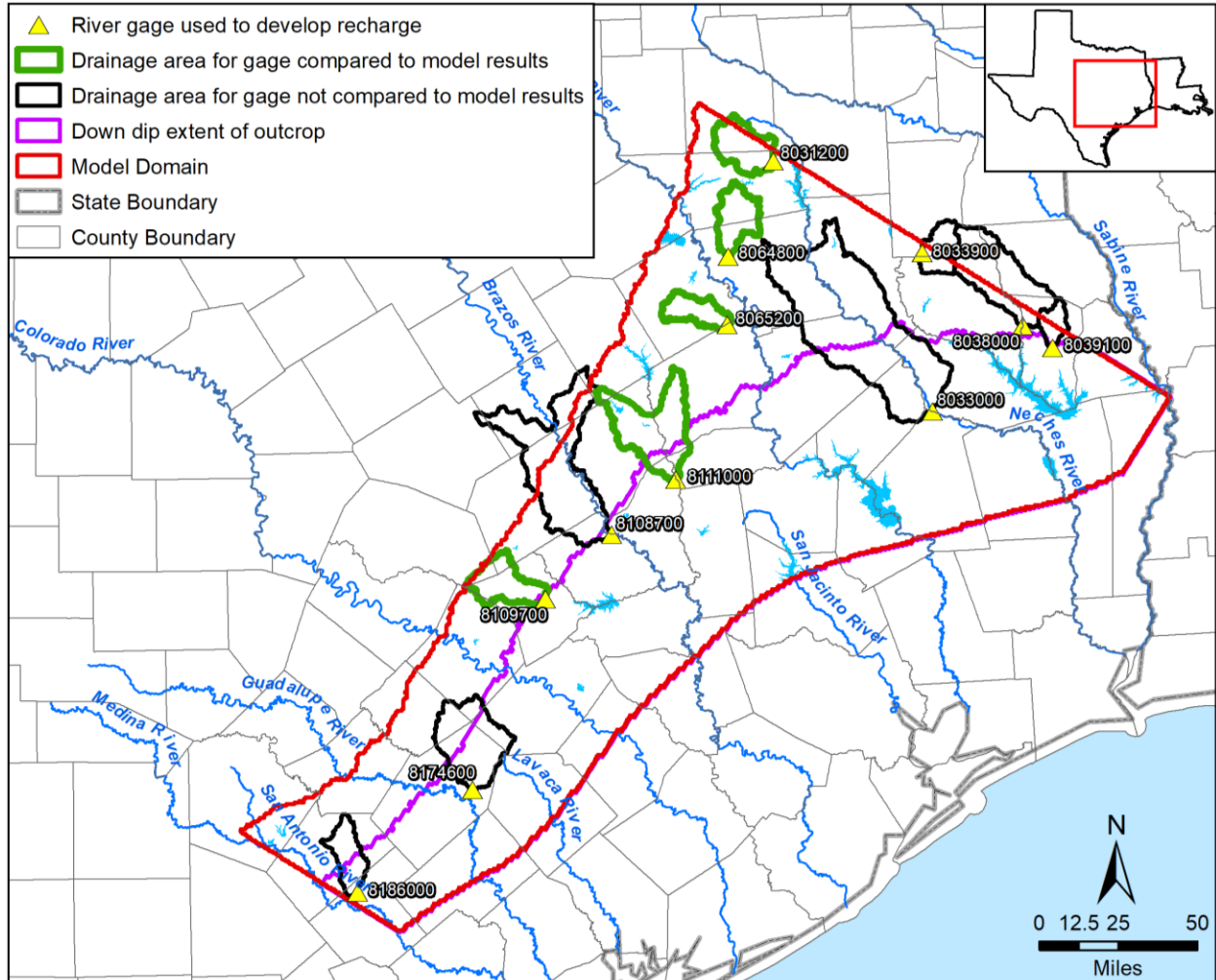
Figure 5.4a. Location of five out of 12 river gages used to develop regression between recharge rate and annual precipitation that have watersheds with more than 90 percent of their area in the outcrop of the model domain.
