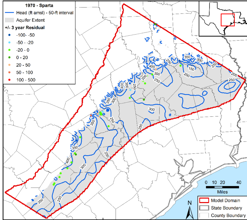
Figure 5.3.4h. Contours in feet (ft) above mean sea level (amsl) developed from simulated hydraulic heads for 1970 in the Sparta Aquifer with residuals posted.
