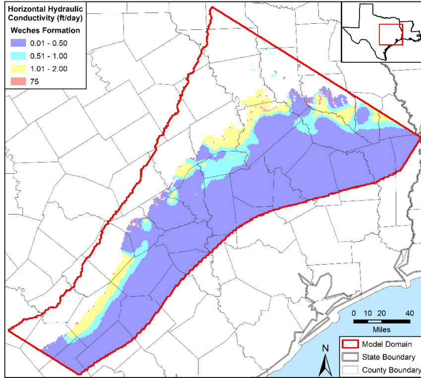
Figure 4.3.2c. Horizontal hydraulic conductivity values in the calibrated model in feet per day (ft/day) for the Weches Formation in model layers 2 and 4.
