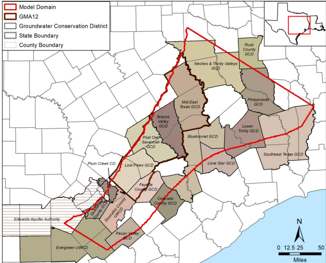
Figure 2.2e. Groundwater conservation districts (GCDs) in the active model area (TWDB, 2017b).
