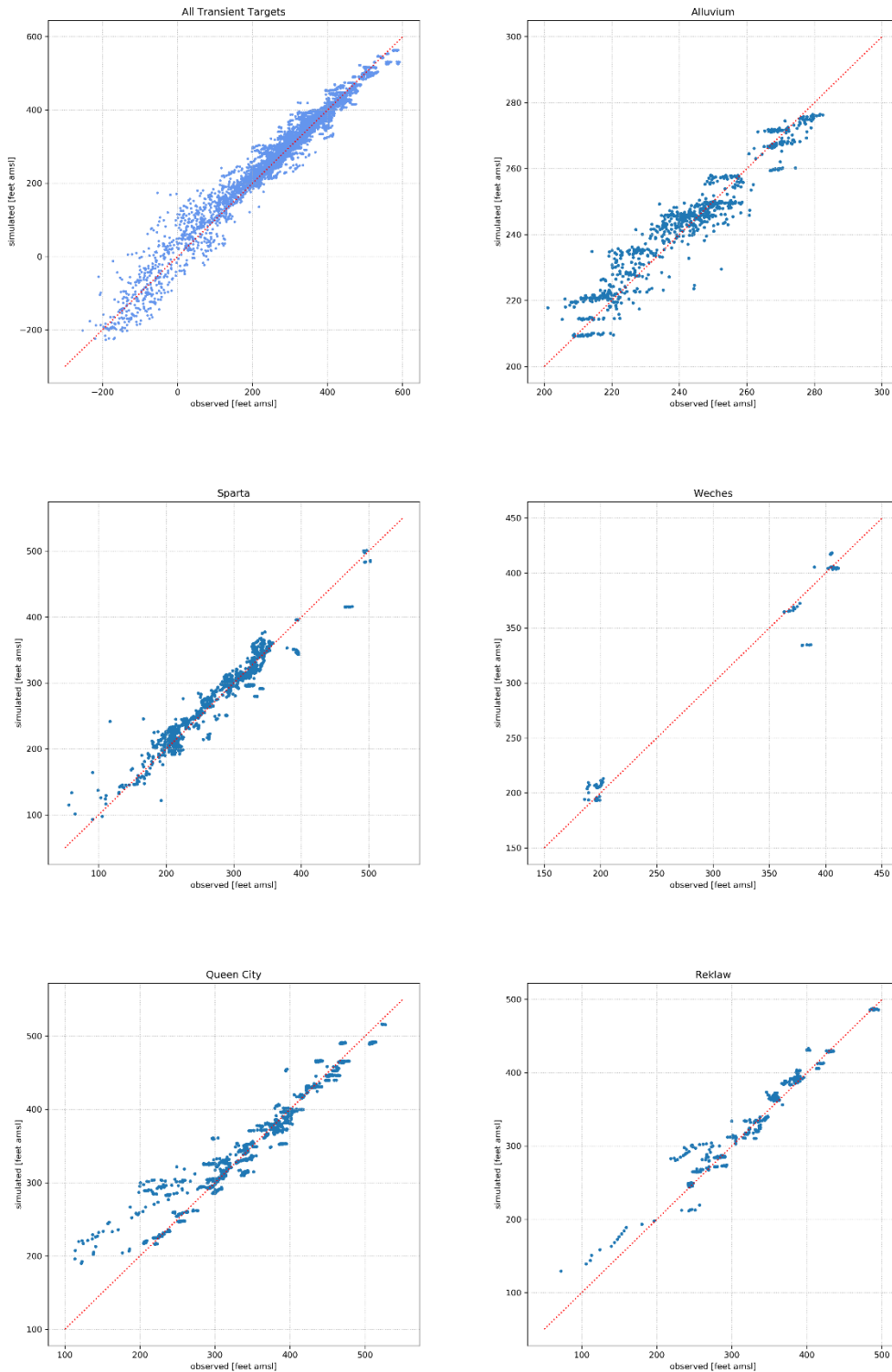
Figure 5.3.3i. Scatter plots of simulated versus observed hydraulic heads for all calibration targets in all wells in the entire model domain, the Brazos River alluvium, the Sparta Aquifer, the Weches Formation, the Queen City Aquifer, and the Reklaw Formation for the transient period 1930 to 2010.
