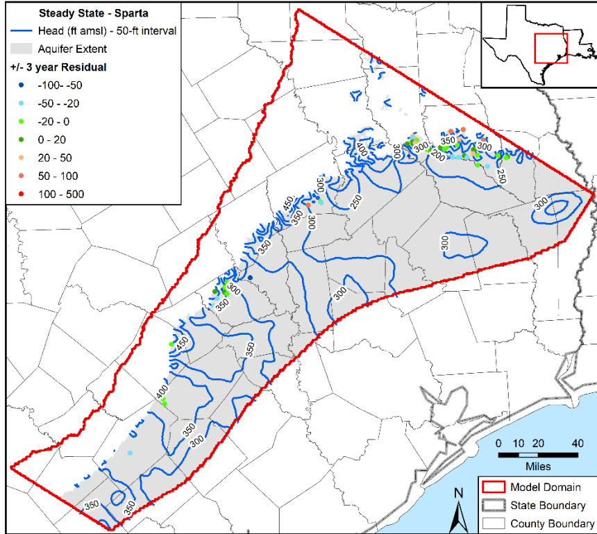
Figure 5.3.4f. Contours in feet (ft) above mean sea level (amsl) developed from simulated hydraulic heads for steady-state conditions in the Sparta Aquifer with residuals posted.
