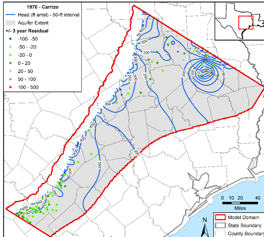
Figure 5.3.4bb. Contours in feet (ft) above mean sea level (amsl) developed from simulated hydraulic heads for 1970 in the Carrizo Aquifer with residuals posted.
