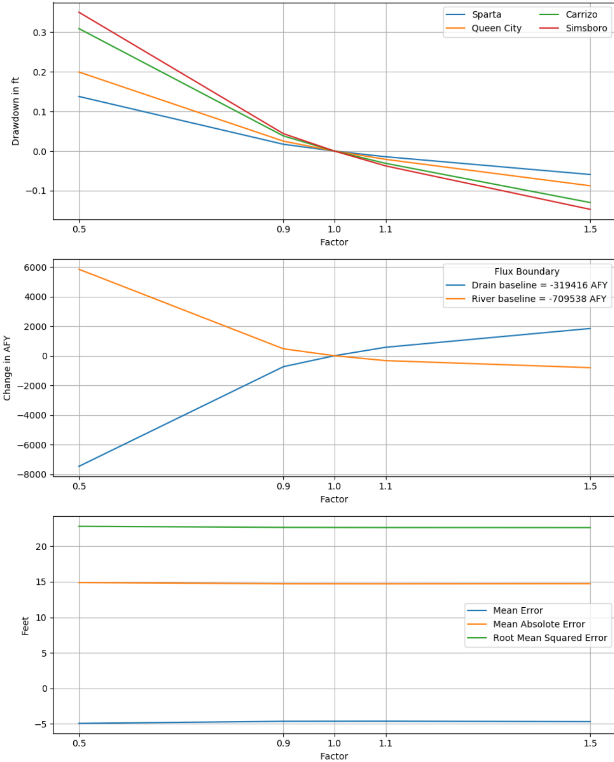
Figure 6.2.2s. Sensitivities of 2010 drawdown in hydrogeologic units (top), hydraulic boundary fluxes (center), and calibration statistics (bottom) to the conductance of river cells for the transient model.
