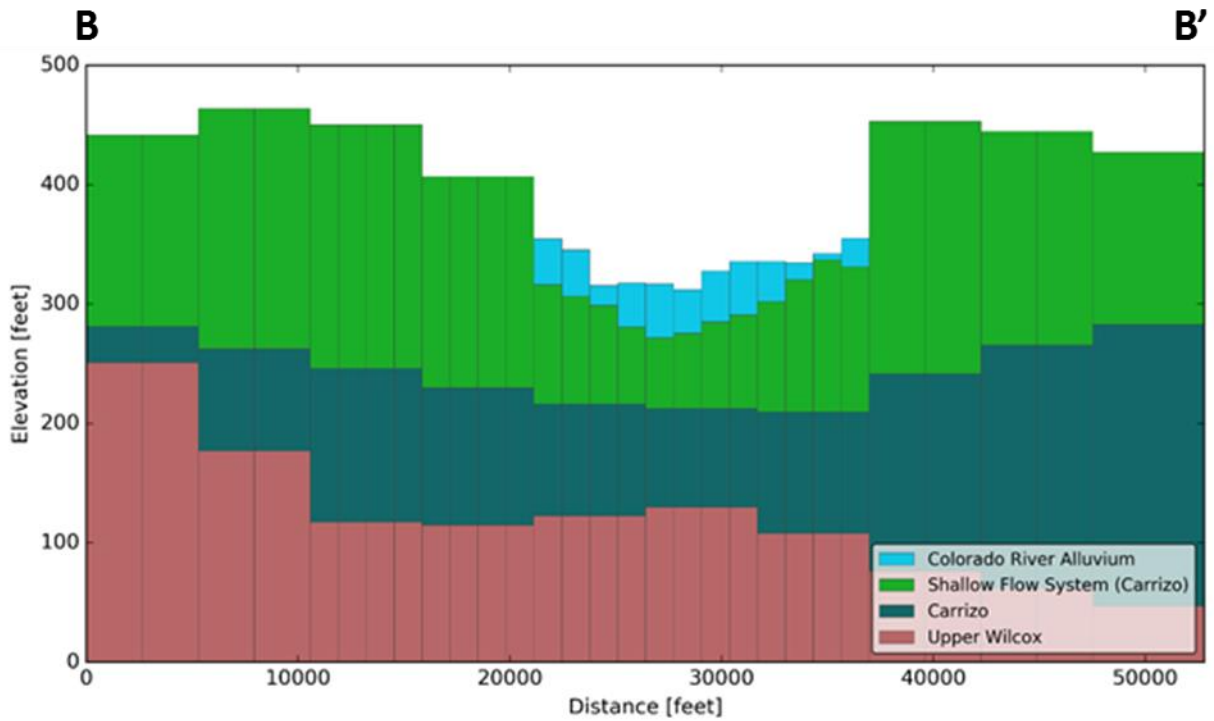
Figure 3.4.1c. Vertical cross-section for the updated model showing the model layers in the upper 400 feet along transect B-B' shown in Figure 3.4.1a.
