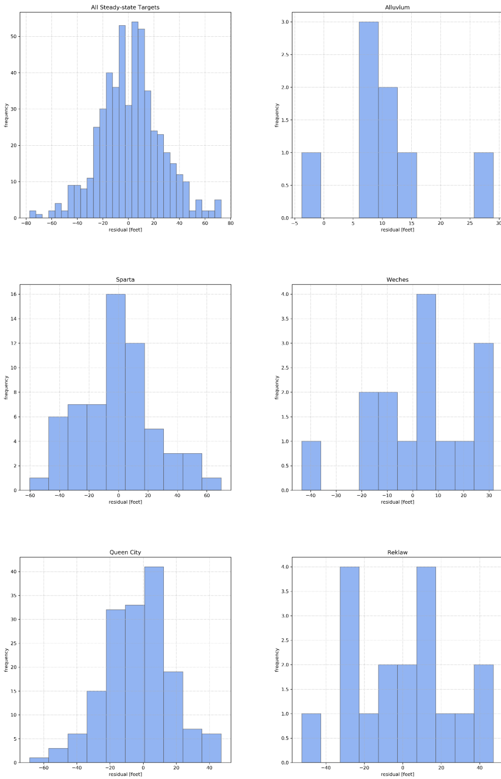
Figure 5.3.2d. Histograms of the hydraulic head residuals for the entire model domain, the Brazos River alluvium, the Sparta Aquifer, the Weches Formation, the Queen City Aquifer, and the Reklaw Formation the across the entire model domain for the steady-state period.
