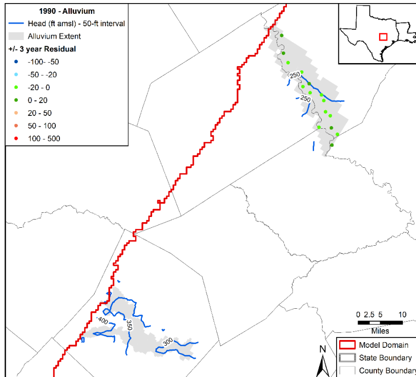
Figure 5.3.4d. Contours in feet (ft) above mean sea level (amsl) developed from simulated hydraulic heads for 1990 in the Colorado and Brazos rivers alluvium with residuals for the Brazos River alluvium posted.
