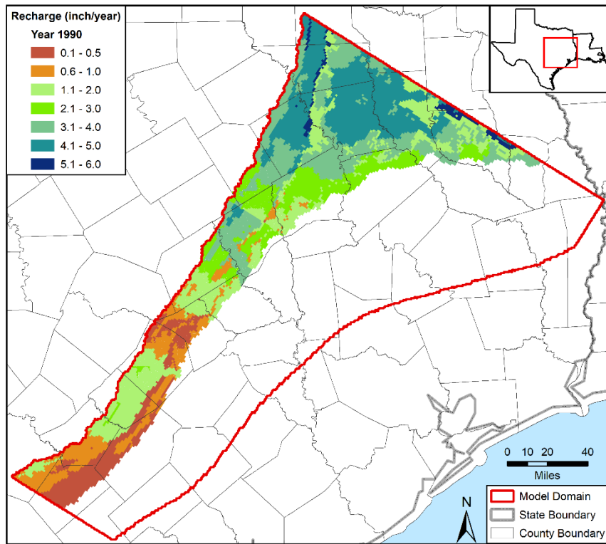
Figure 4.6d. Spatial distribution of recharge in inches per year for 1990.
