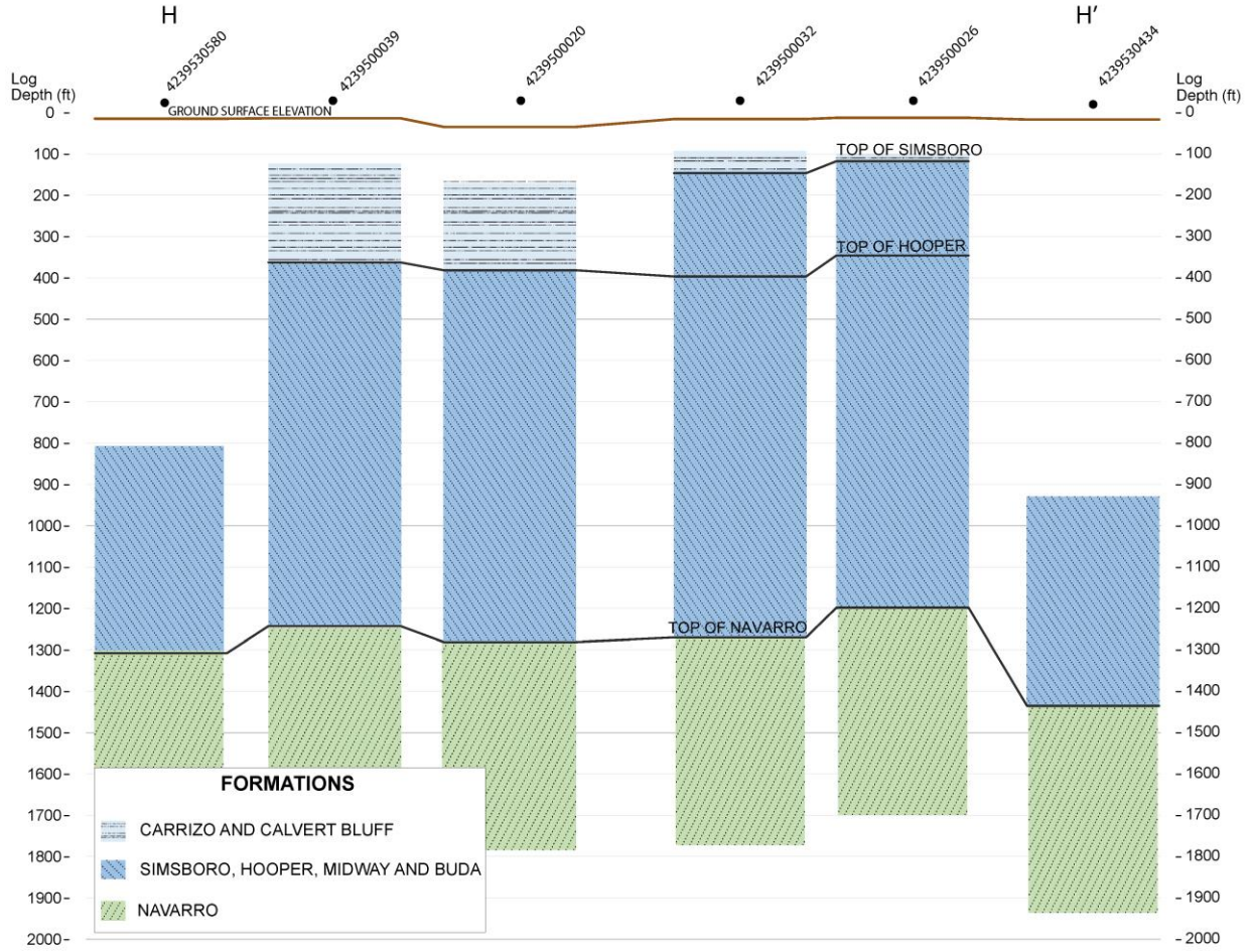
Figure 3.1.2.4c. Cross-section H-H' through the South Kosse Graben showing the top surface of selected formations and mapped fault locations based on interpretation of geophysical logs in and near cross-section H-H'.
