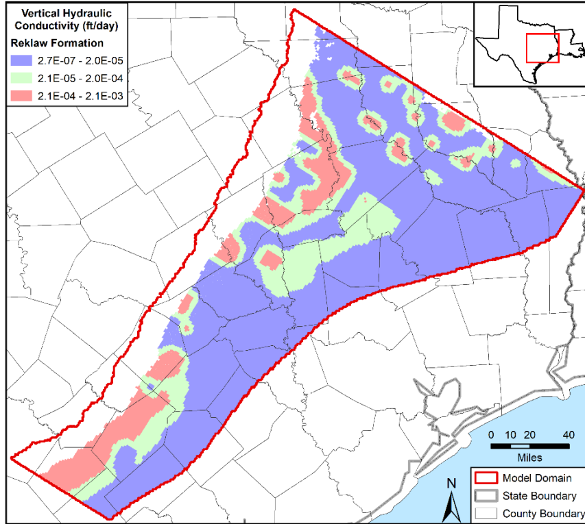
Figure 4.3.2o. Vertical hydraulic conductivity values in the calibrated model in feet per day (ft/day) for the Reklaw Formation in model layers 2 and 6.
