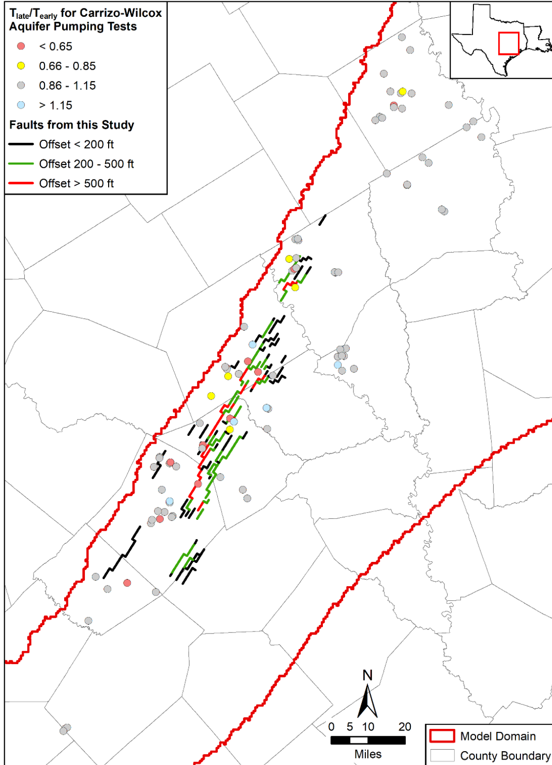
Figure 3.1.4.1g. Spatial distribution of aquifer tests performed in the Carrizo-Wilcox Aquifer categorized based on the late-to early-time transmissivity ratio.
