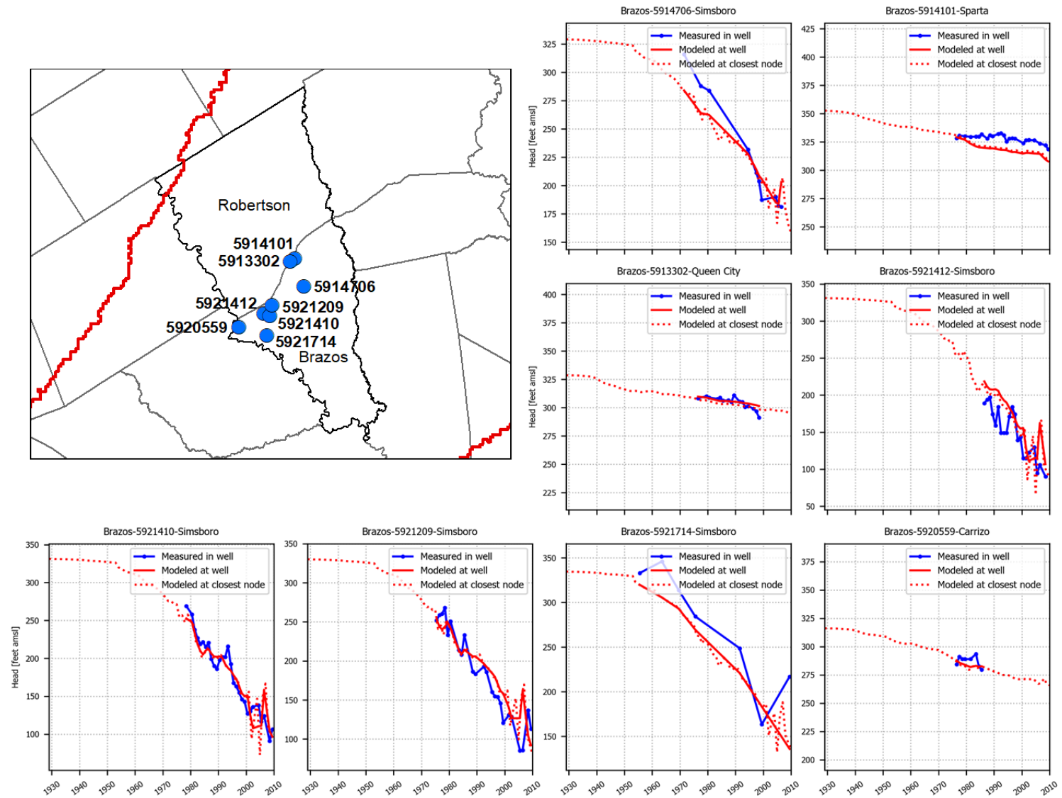
Figure 5.3.6d. Hydrographs showing simulated and measured hydraulic heads (in feet above mean sea level) in the Brazos Valley Groundwater Conservation District at eight wells with state well numbers 5914706, 5914101, 5913302, 5921412, 5921410, 5921209, 5921714, and 5920559.
