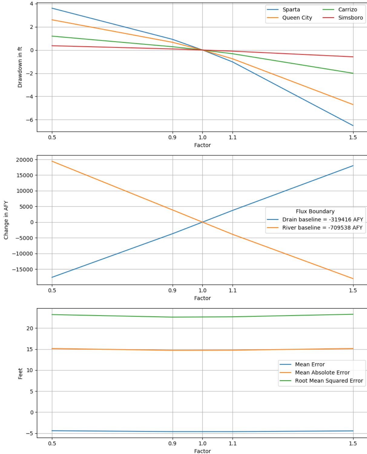
Figure 6.2.2a. Sensitivities of 2010 drawdown in hydrogeologic units (top), hydraulic boundary fluxes (center), and calibration statistics (bottom) to the horizontal hydraulic conductivity of the Sparta Aquifer for the transient model.
