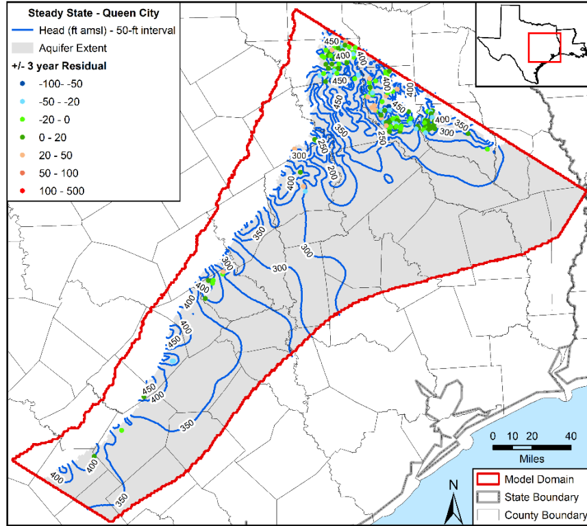
Figure 5.3.4p. Contours in feet (ft) above mean sea level (amsl) developed from simulated hydraulic heads for steady-state conditions in the Queen City Aquifer with residuals posted.
