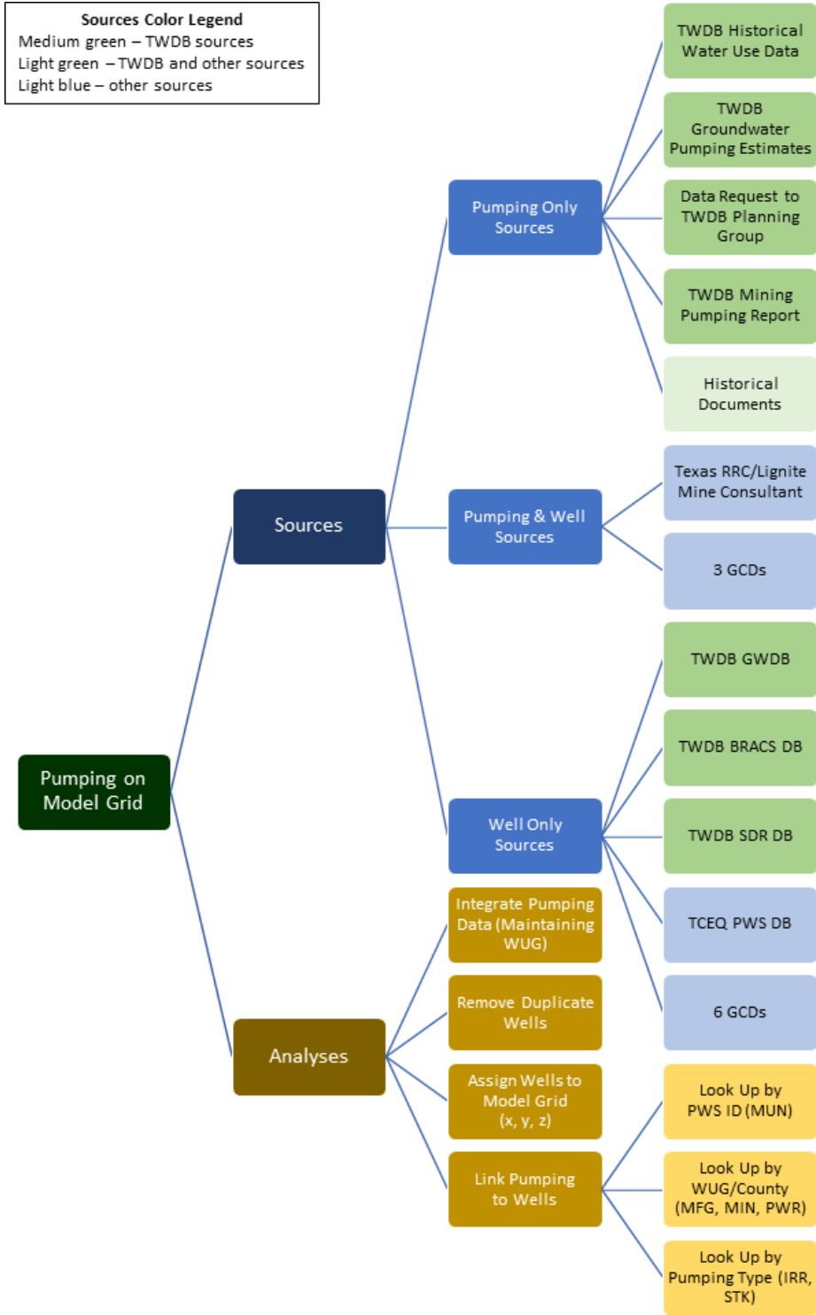
Figure 3.2a. Flow chart showing the data sources and analyses used to assign historical pumping to the model grid.
