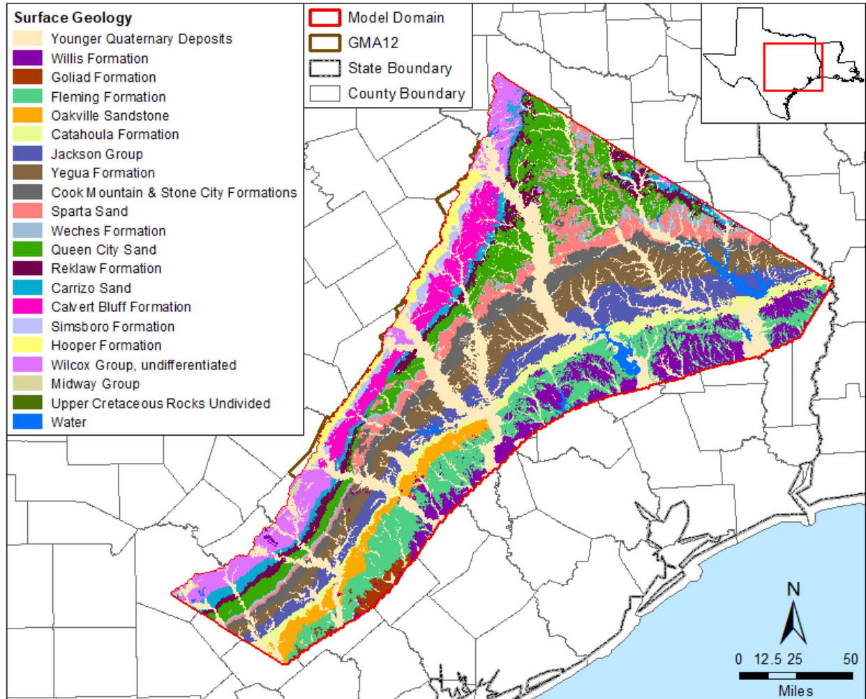
Figure 2.4b. Surface geology of the model area from the Geologic Atlas of Texas (Barnes, 1970, 1979, 1981; Stoeser and others, 2007).
