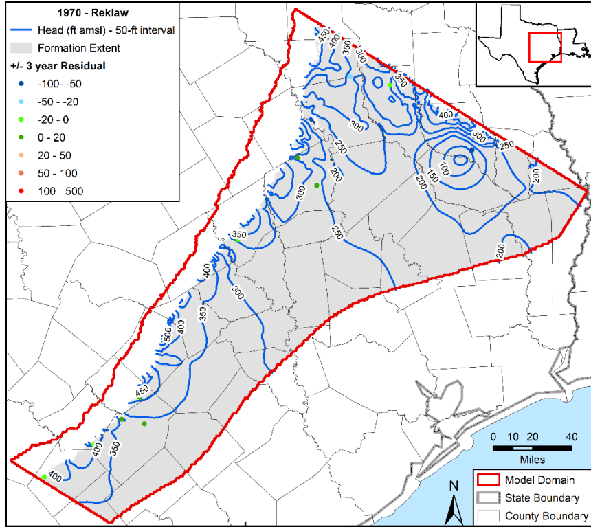
Figure 5.3.4w. Contours in feet (ft) above mean sea level (amsl) developed from simulated hydraulic heads for 1970 in the Reklaw Formation with residuals posted.
