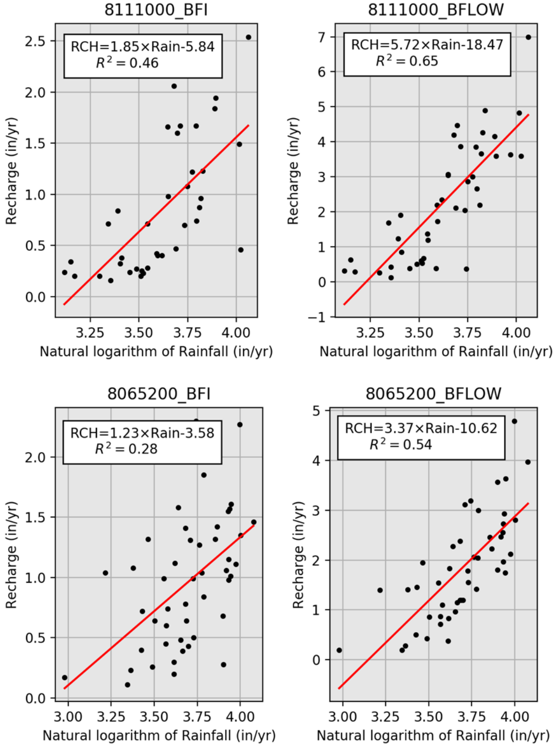
Figure 3.3.3c. Regression of recharge versus annual precipitation values produced by the application of the Base Flow Index Program and Baseflow Program hydrograph separation techniques for river gage 8111000 on the Navasota River in Brazos County and river gage 8065200 on the Upper Keechi Creek in Leon County.
