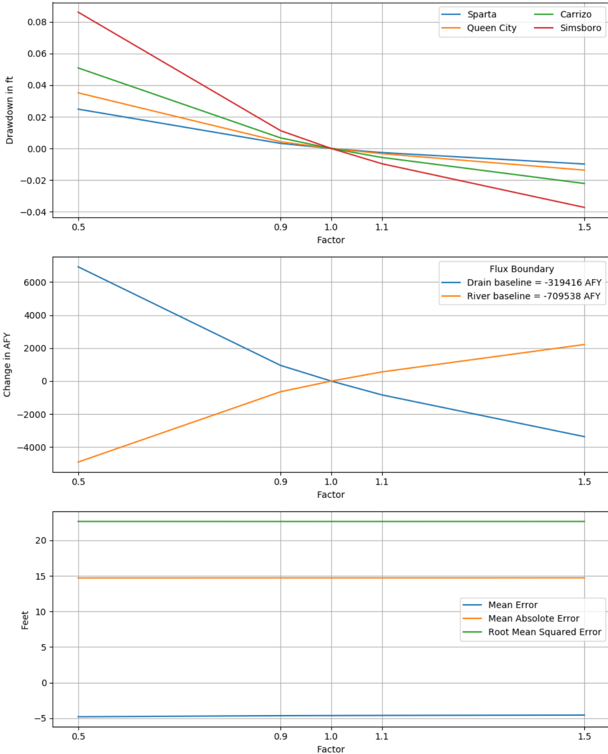
Figure 6.2.2r. Sensitivities of 2010 drawdown in hydrogeologic units (top), hydraulic boundary fluxes (center), and calibration statistics (bottom) to the conductance of drain cells for the transient model.
