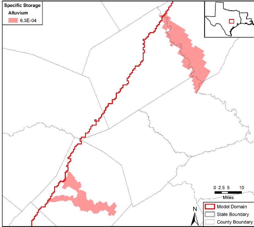
Figure 4.3.2u. Specific storage value in the calibrated model in feet -1 for the Colorado and Brazos rivers alluvium in model layer 1.
