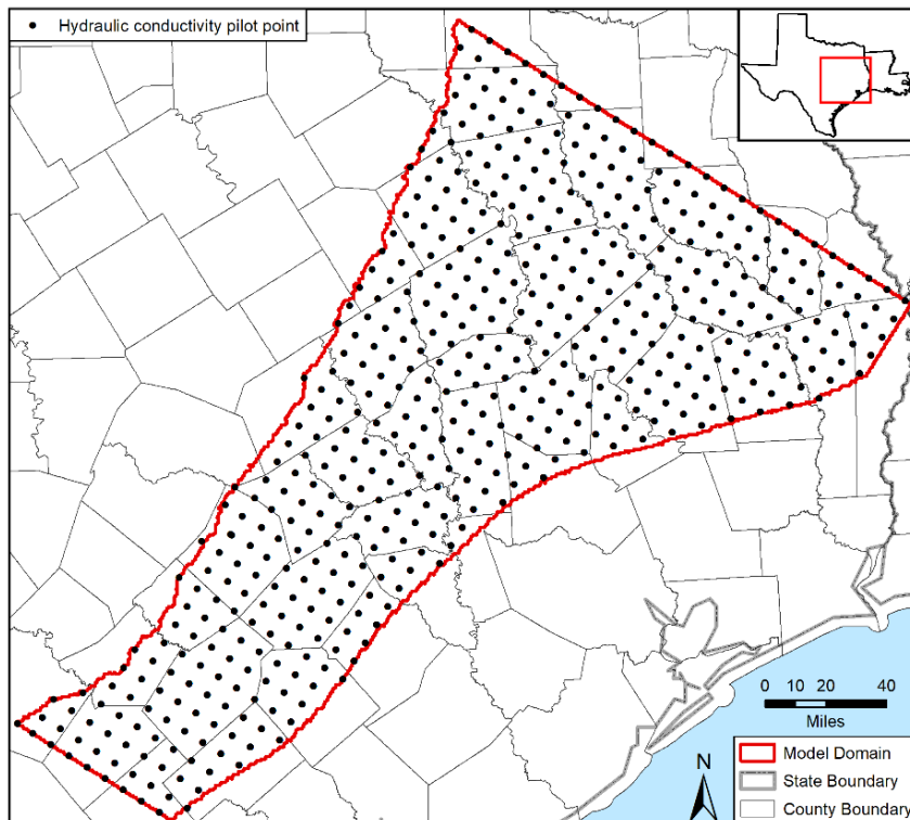
Figure 5.1b. Location of pilot points used for developing horizontal and vertical hydraulic conductivity values for model layers 2 through 10.
