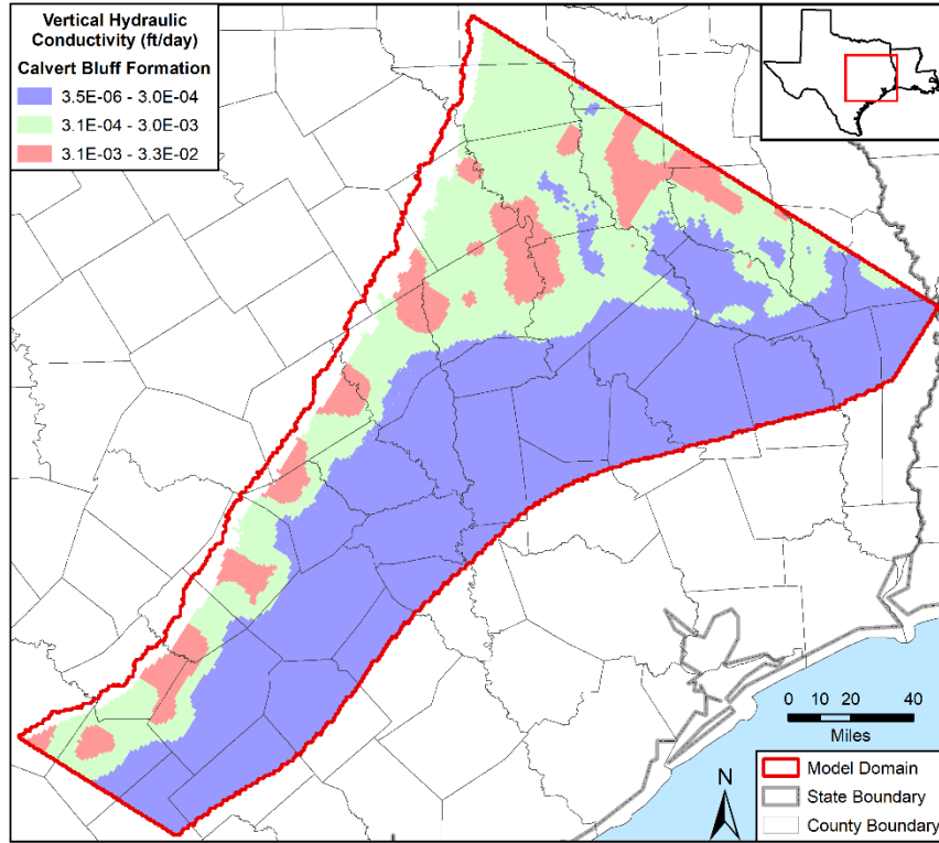
Figure 4.3.2q. Vertical hydraulic conductivity values in the calibrated model in feet per day (ft/day) for the Calvert Bluff Formation in model layers 2 and 8.
