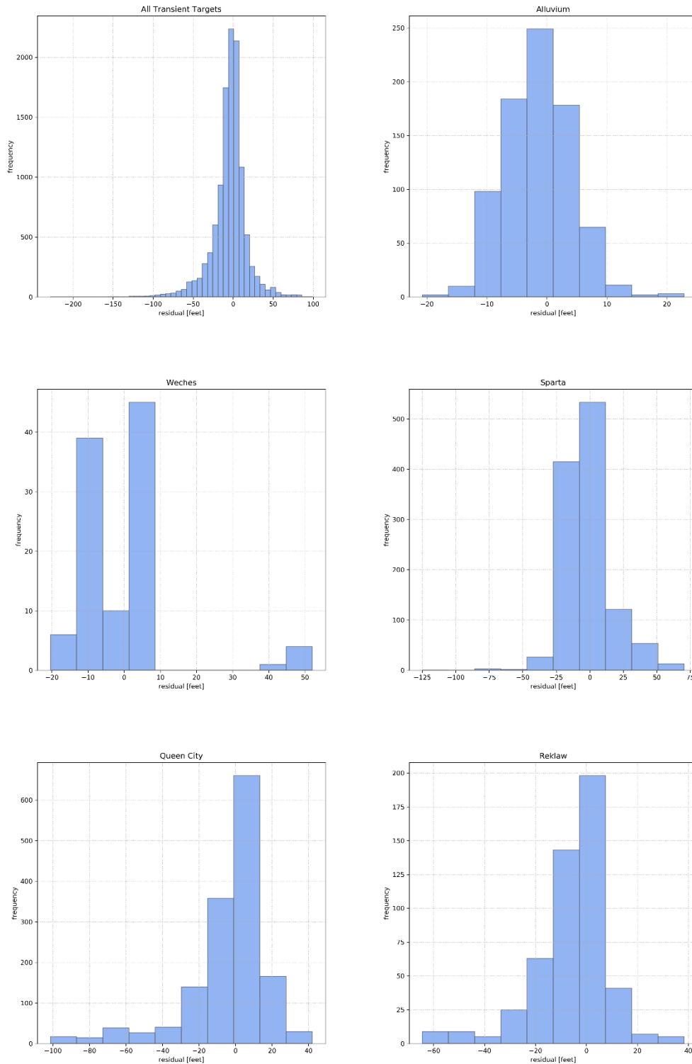
Figure 5.3.3k. Histograms of the hydraulic head residuals for all calibration targets in all wells in the entire model domain, the Brazos River alluvium, the Sparta Aquifer, the Weches Formation, the Queen City Aquifer, and the Reklaw Formation for the transient period 1930 to 2010.
