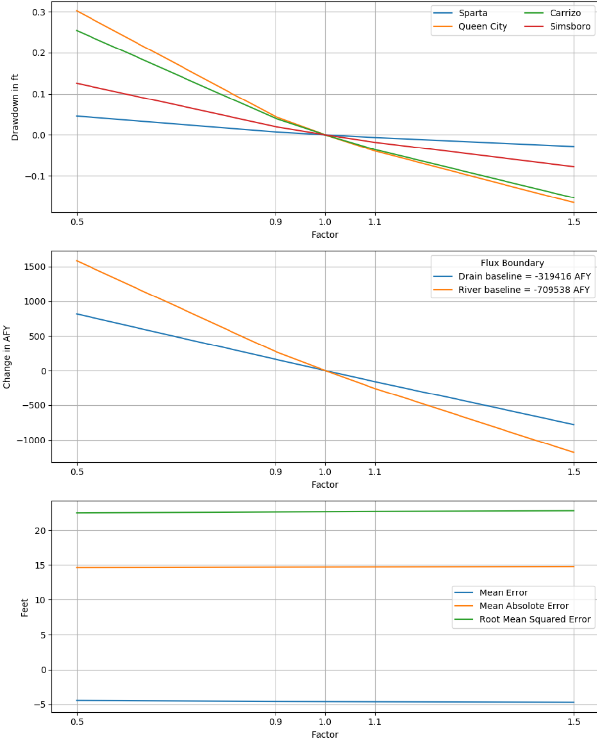
Figure 6.2.2l. Sensitivities of 2010 drawdown in hydrogeologic units (top), hydraulic boundary fluxes (center), and calibration statistics (bottom) to the specific yield of the Queen City Aquifer for the transient model.
