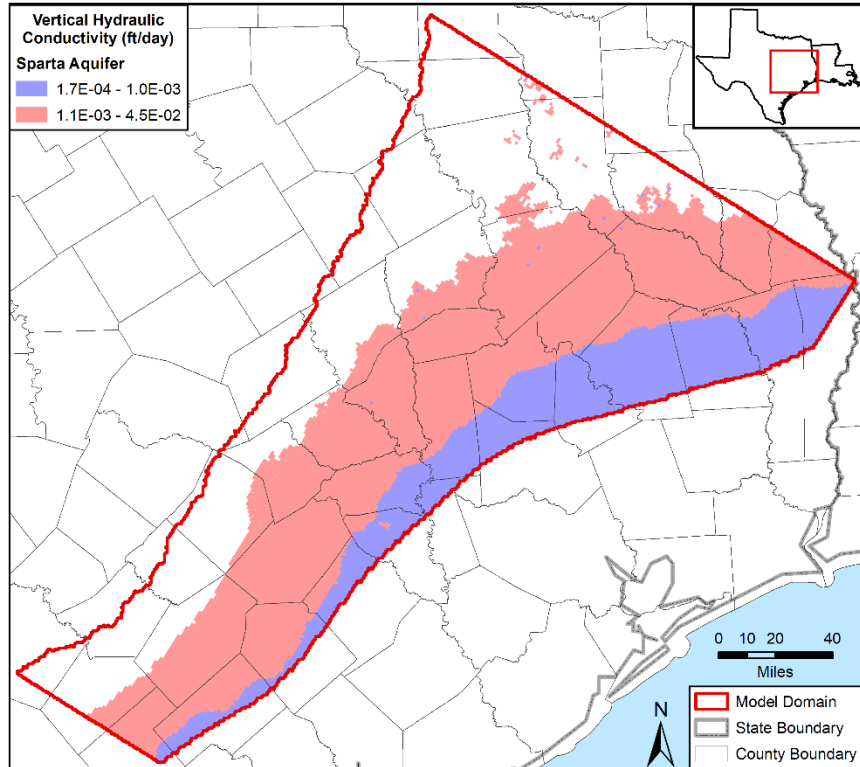
Figure 4.3.2l. Vertical hydraulic conductivity values in the calibrated model in feet per day (ft/day) for the Sparta Aquifer in model layers 2 and 3.
