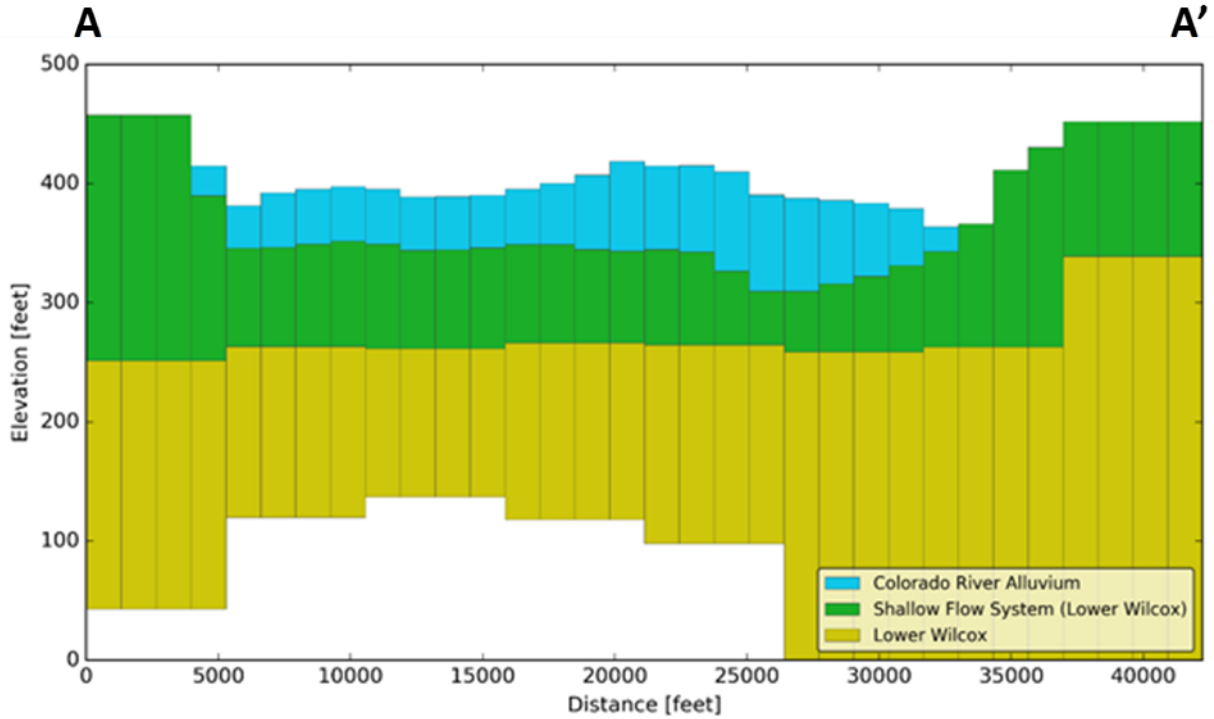
Figure 3.4.1b. Vertical cross-section for the updated model showing the model layers in the upper 400 feet along transect A-A' shown in Figure 3.4.1a.
