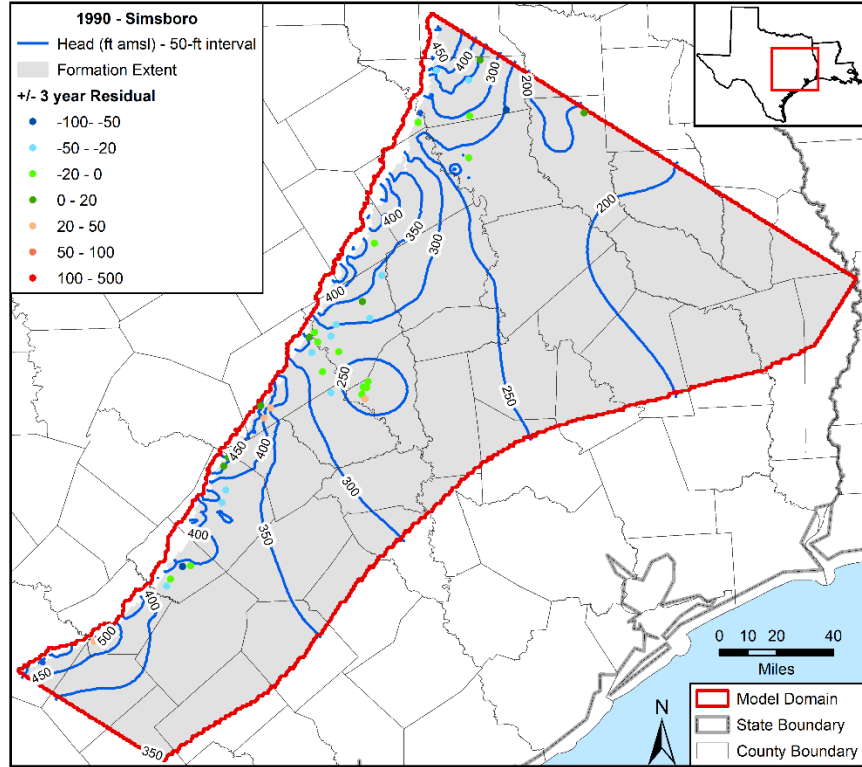
Figure 5.3.4mm. Contours in feet (ft) above mean sea level (amsl) developed from simulated hydraulic heads for 1990 in the Simsboro Formation with residuals posted.
