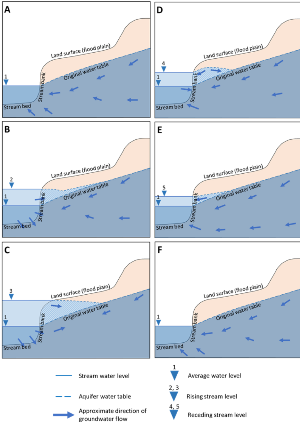
Figure 3.3.4.2a. Schematic showing groundwater flow toward a stream at sequential times. Water levels during average flow conditions at a gaining stream (A). Increase in stream elevation during a flooding event causes hydraulic gradient reversal at stream-aquifer interface. Streamflow enters aquifer and becomes bank storage in stream bank (B and C). Decrease in stream elevation after a flooding event. Bank storage flows back to the stream as bank flow as water level in the stream lowers over time (D and E). Water levels in stream and aquifer return to conditions that existed prior to flood event (F).
