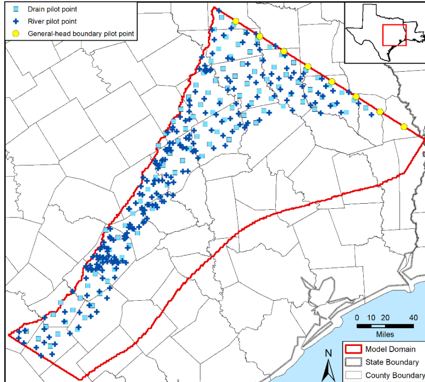
Figure 5.1a. Location of pilot points used for developing conductance values for general-head boundary, drain, and river cells.
