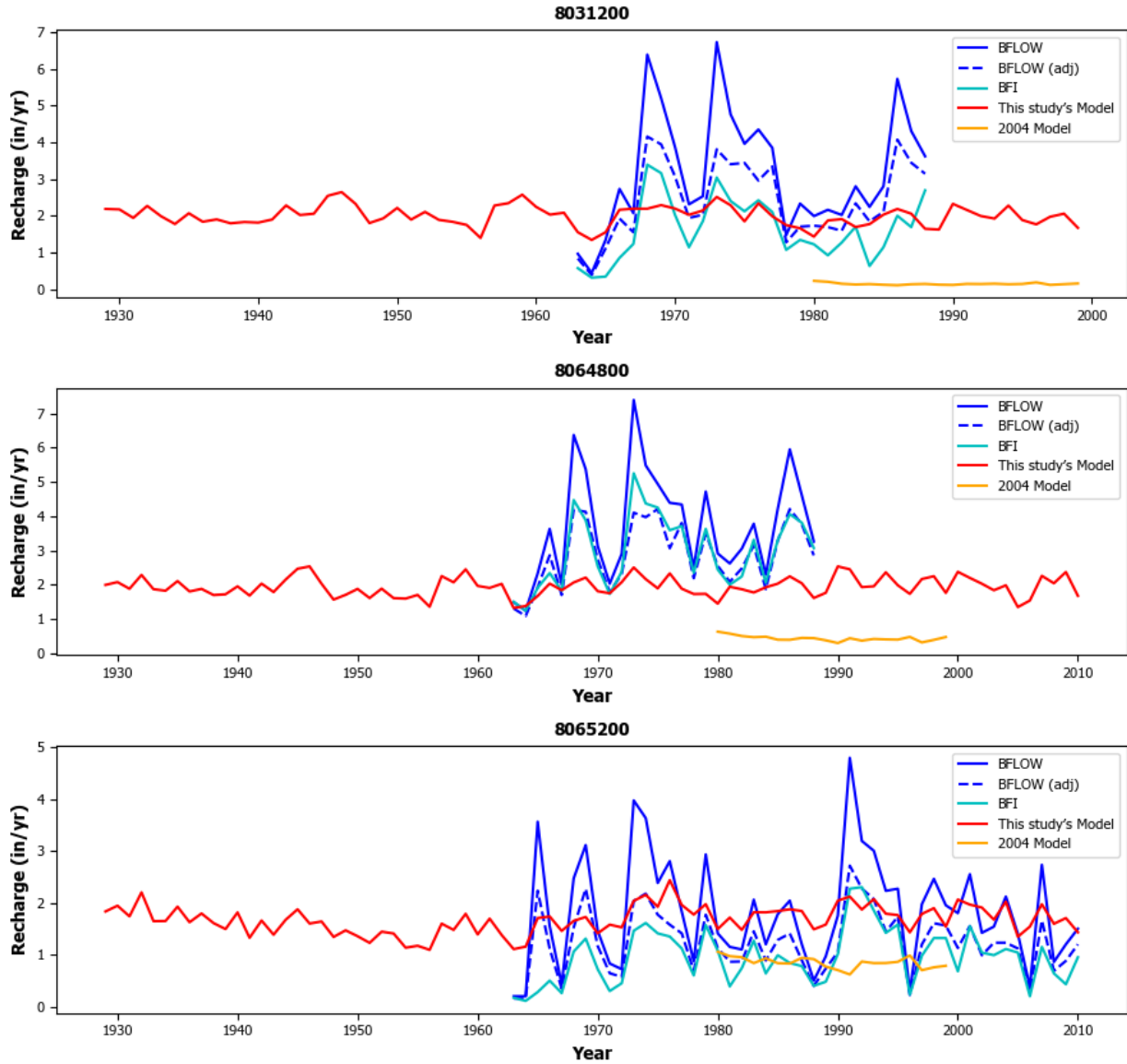
Figure 5.4.2a Comparison of recharge rates (in inches per year) calculated from base flow for river gages 8031200, 8064800, and 8065200 based on the Baseflow Program analysis and adjusted Baseflow Program values, the Base Flow Index Program analysis, and calculated from this study's model and the 2004 groundwater availability model by Kelley and others (2004). The model values equal the model calculated discharge to rivers/streams.
