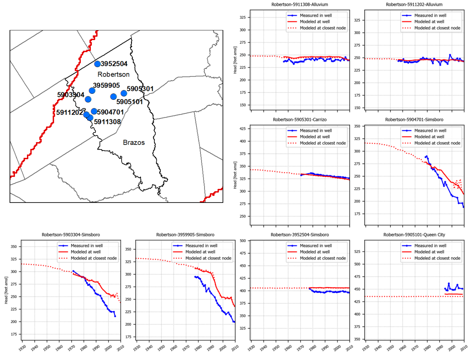
Figure 5.3.6c. Hydrographs showing simulated and measured hydraulic heads (in feet above mean sea level) in the Brazos Valley Groundwater Conservation District at eight wells with state well numbers 5911308, 5911202, 05905301, 05904701, 05903304, 03959905, 03952504, 03952504, 05905101.
