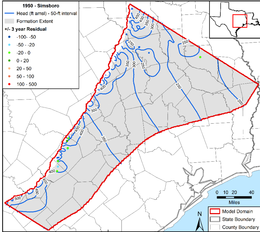
Figure 5.3.4kk. Contours in feet (ft) above mean sea level (amsl) developed from simulated hydraulic heads for 1950 in the Simsboro Formation with residuals posted.
