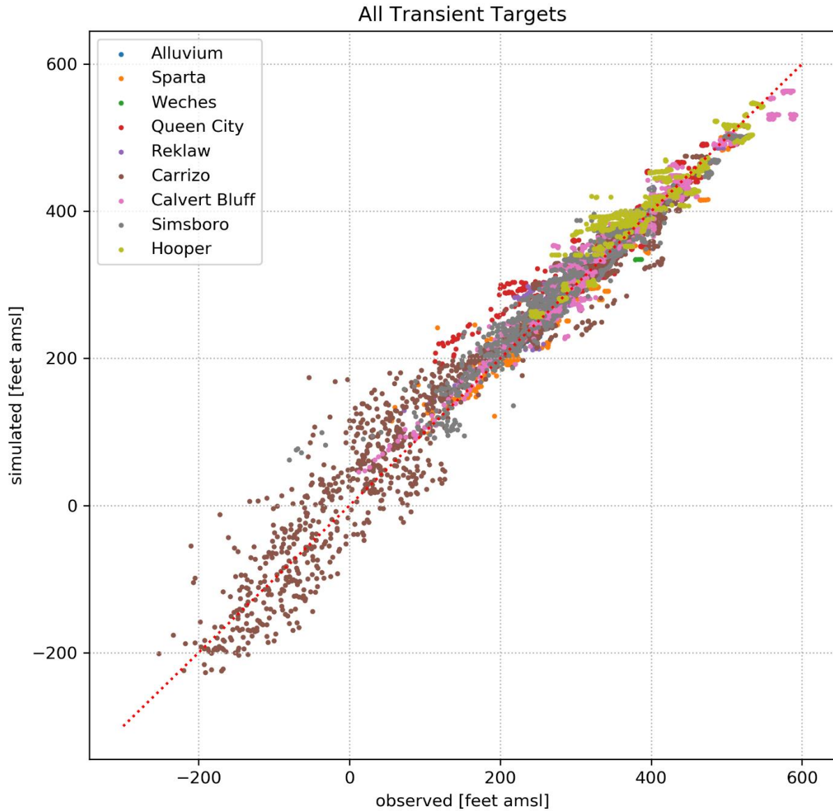
Figure 5.3.3g. Scatter plot of simulated versus observed hydraulic heads for the 11,378 water levels used as calibration targets across the entire model for the transient period 1930 to 2010.
