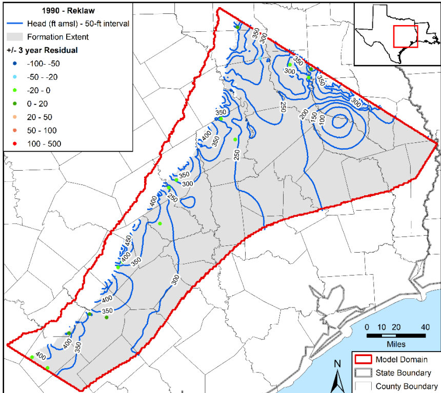
Figure 5.3.4x. Contours in feet (ft) above mean sea level (amsl) developed from simulated hydraulic heads for 1990 in the Reklaw Formation with residuals posted.
