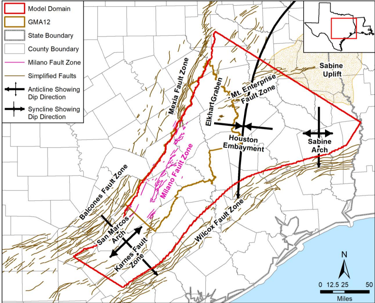
Figure 2.4a. Map of major faults and structural features in the vicinity of the model area. Wilcox and Balcones Fault Zones modified from Ewing and others (1990), Milano Fault Zone developed by this study; and structural axes modified from Guevara and Garcia (1972), Galloway (1982), and Galloway and others (2000).
