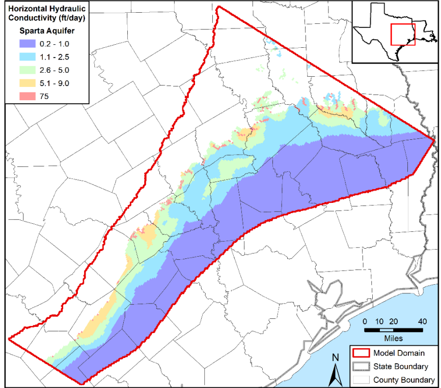
Figure 4.3.2b. Horizontal hydraulic conductivity values in the calibrated model in feet per day (ft/day) for the Sparta Aquifer in model layers 2 and 3.
