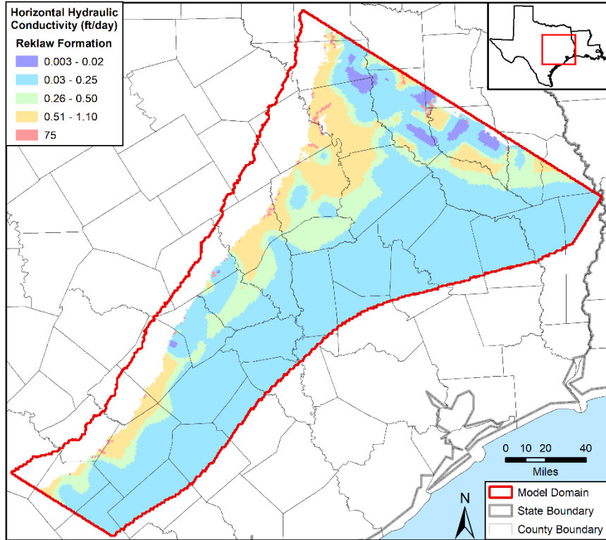
Figure 4.3.2e. Horizontal hydraulic conductivity values in the calibrated model in feet per day (ft/day) for the Reklaw Formation in model layers 2 and 6.
