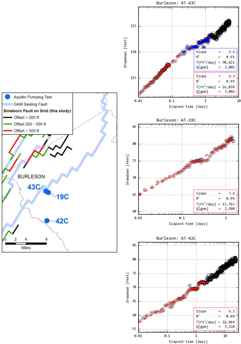
Figure 3.1.4.1f. Location of aquifer pumping tests near faults in Burleson County that produced a CJSL-calculated late-time transmissivity value equal to or greater than the early-time transmissivity value, which provides little evidence that faults could be affecting groundwater flow. For aquifer tests AT-43C, AT-19C, and AT-42C, the values for the late-to early-time transmissivity ratio are 1.82, 1.0, and 1.0, respectively.
