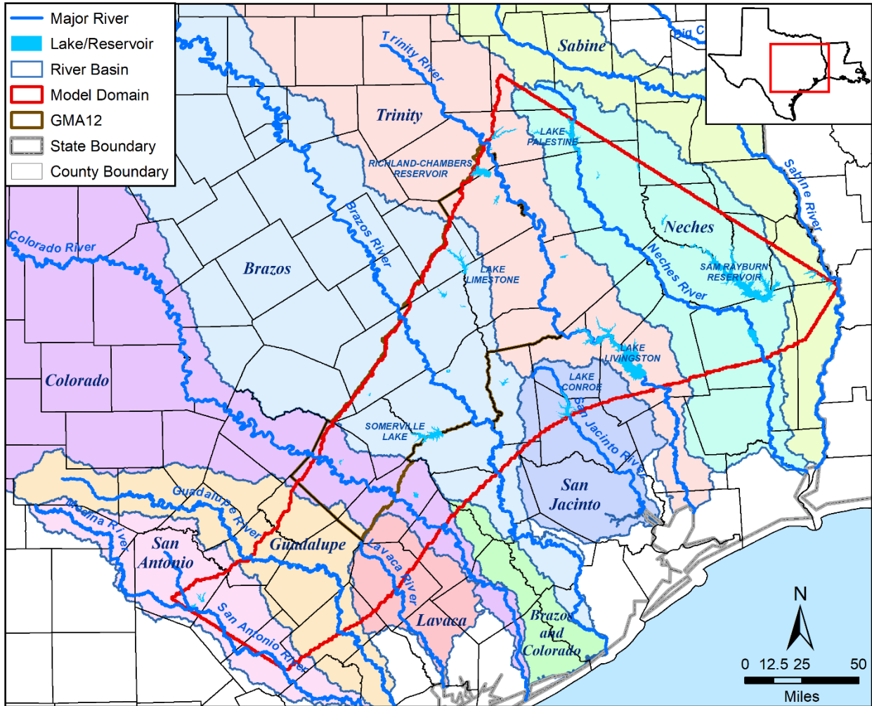
Figure 2.2c. Rivers, lakes, reservoirs, and river basins in the active model area (TWDB, 2009; TWDB, 2014b, c).
