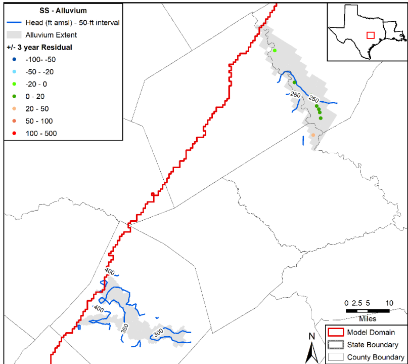
Figure 5.3.4a. Contours in feet (ft) above mean sea level (amsl) developed from simulated hydraulic heads for steady-state conditions in the Colorado and Brazos rivers alluvium with residuals for the Brazos River alluvium posted.
