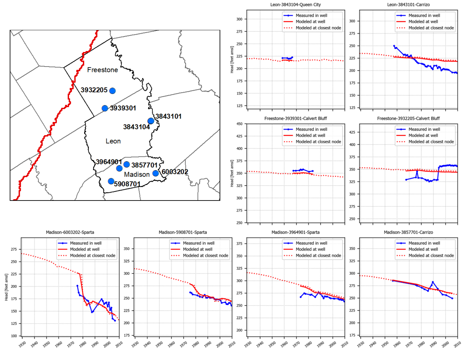
Figure 5.3.6g. Hydrographs showing simulated and measured hydraulic heads (in feet above mean sea level) in the Mid-East Texas Groundwater Conservation District at eight wells with state well numbers 3843104, 3843101, 3939301, 3932205, 6003202, 5908701, 3964901, and 3857701.
