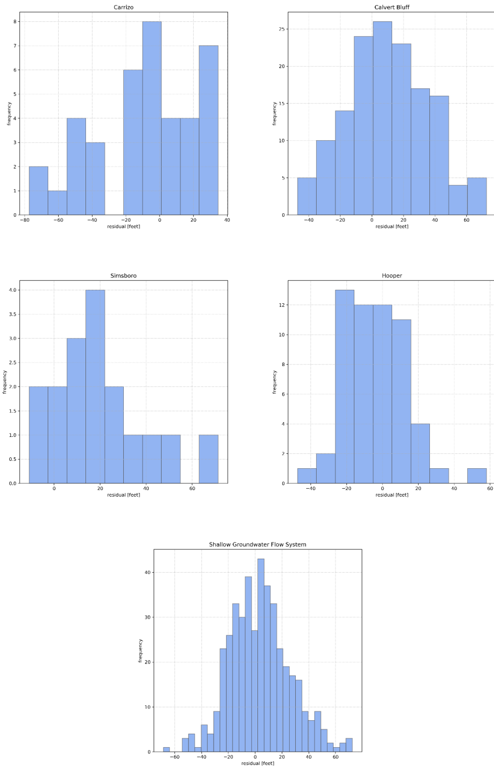
Figure 5.3.2e. Histograms of the hydraulic head residuals for the Carrizo Aquifer, the Calvert Bluff Formation, the Simsboro Aquifer, the Hooper Aquifer, and the shallow groundwater flow system the across the entire model domain for the steady-state period.
