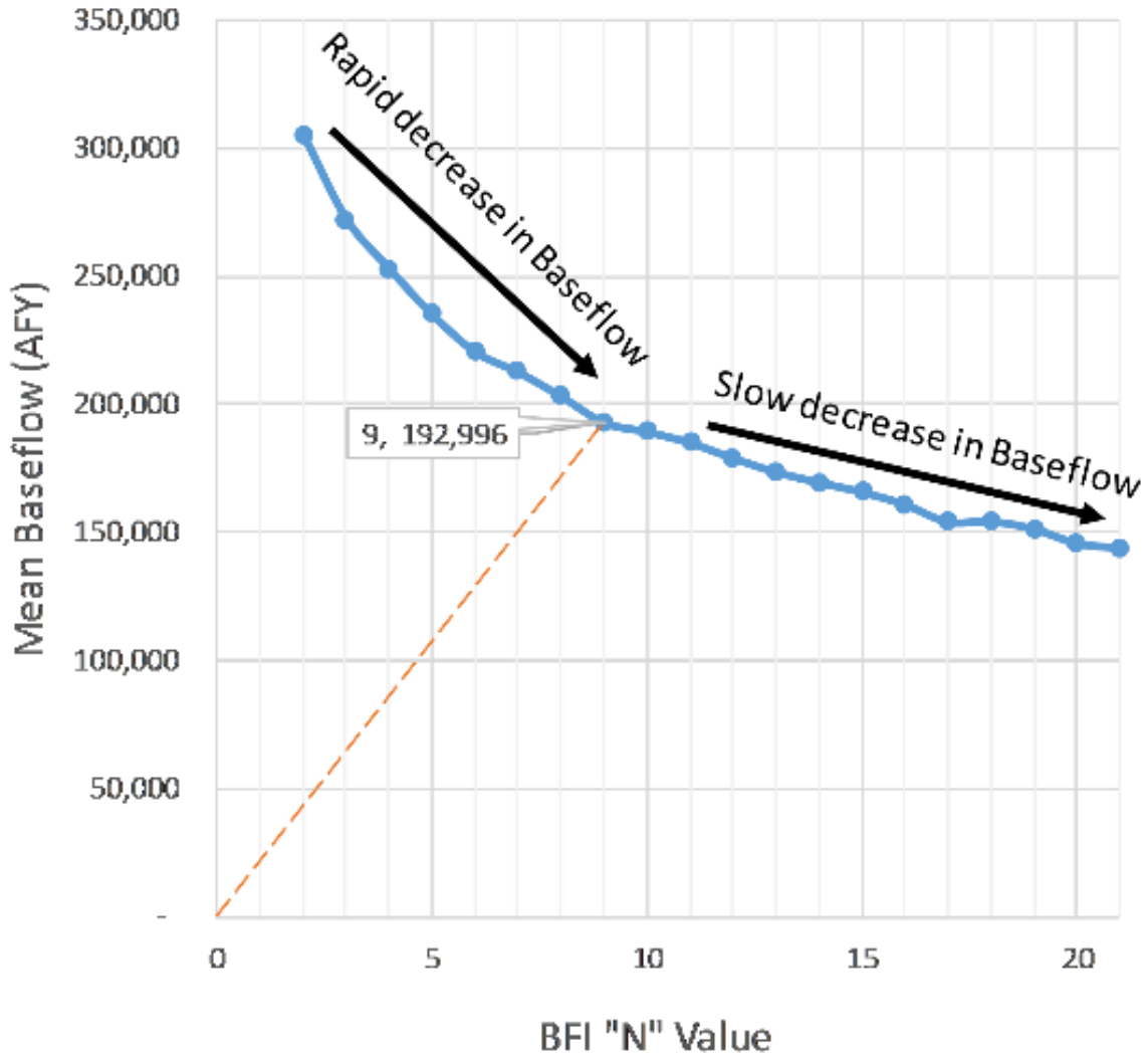
Figure 3.3.2.1b. Mean base flow from the Base Flow Index Program (BFI) analysis for river gage 08041500 for different values of the N parameter, which shows that the greatest change in slope occurs for an N value of 9.
