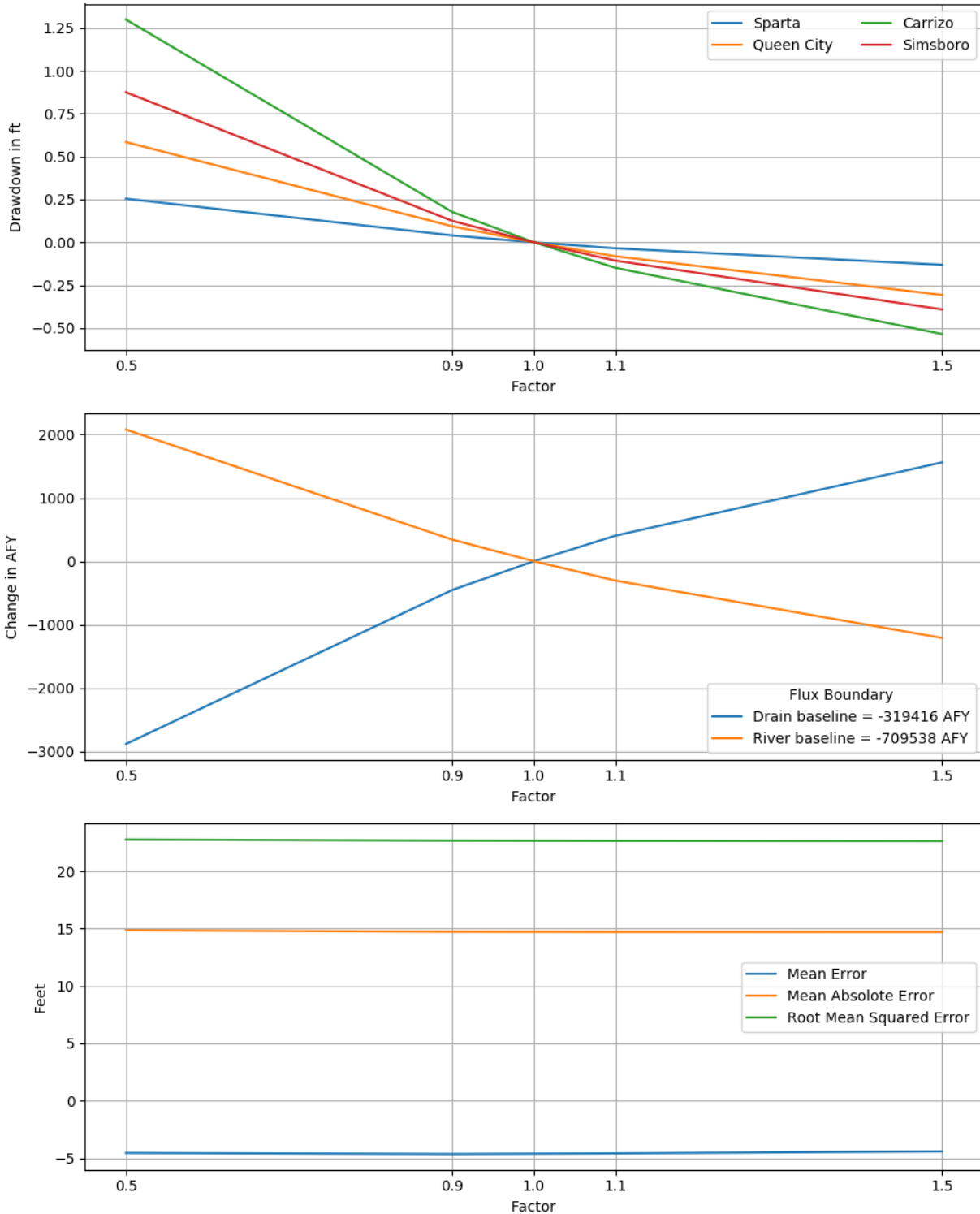
Figure 6.2.2f. Sensitivities of 2010 drawdown in hydrogeologic units (top), hydraulic boundary fluxes (center), and calibration statistics (bottom) to the vertical hydraulic conductivity of the Carrizo Aquifer for the transient model.
