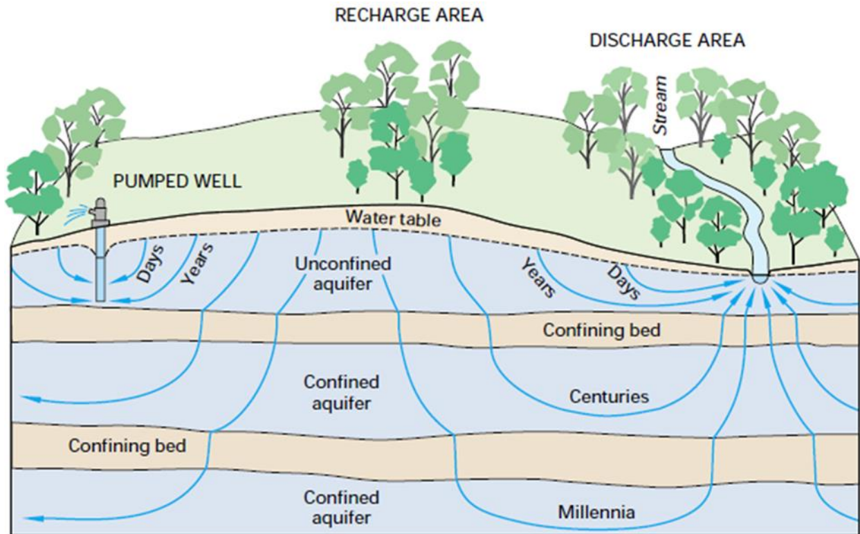
Figure 3.4a Schematic illustration of the different spatial and time scales of groundwater flow paths (Winter and others, 1999).
