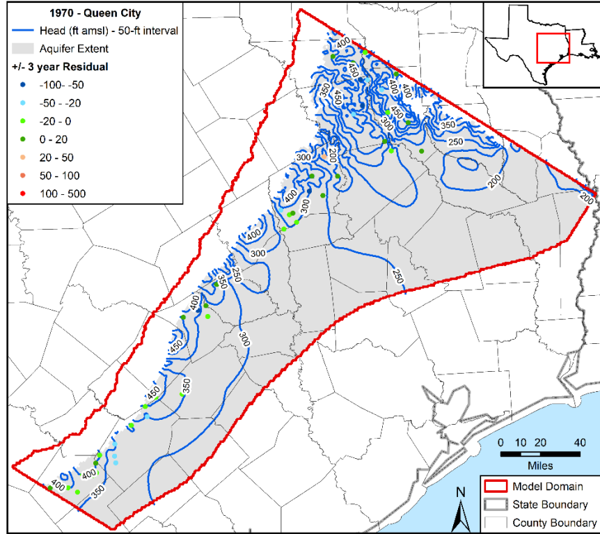
Figure 5.3.4r. Contours in feet (ft) above mean sea level (amsl) developed from simulated hydraulic heads for 1970 in the Queen City Aquifer with residuals posted.
