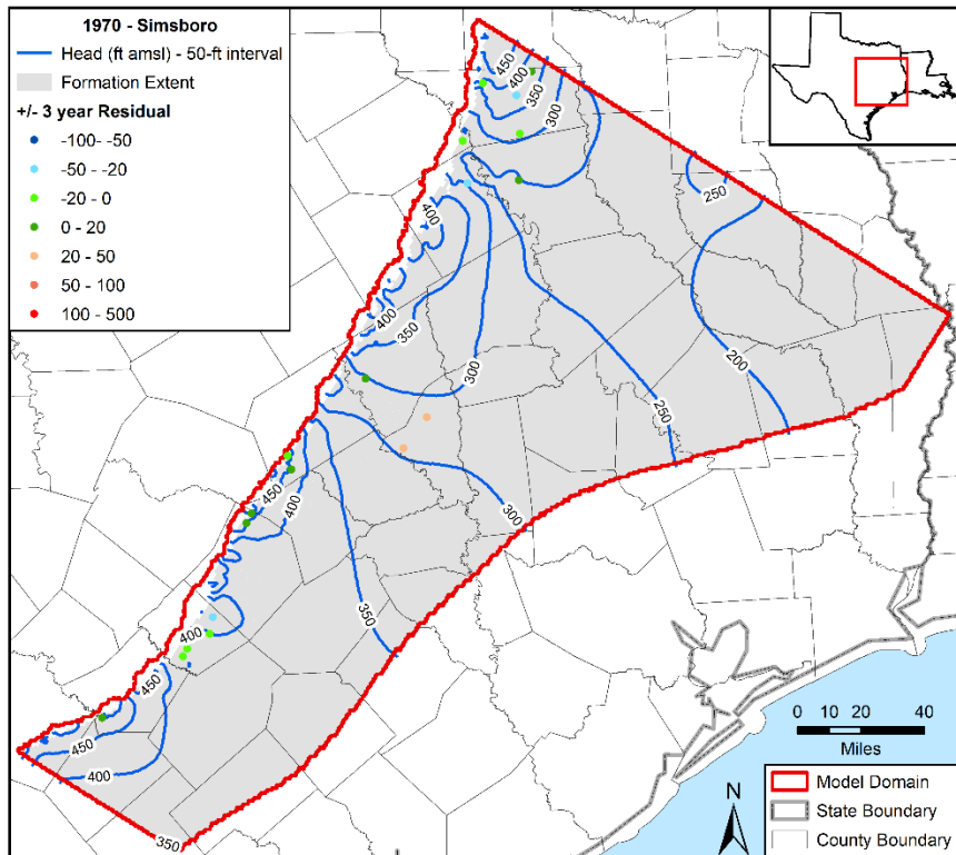
Figure 5.3.4ll. Contours in feet (ft) above mean sea level (amsl) developed from simulated hydraulic heads for 1970 in the Simsboro Formation with residuals posted.
