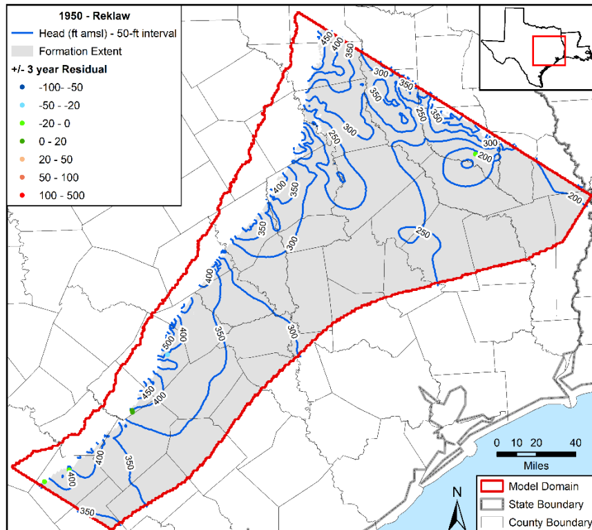
Figure 5.3.4v. Contours in feet (ft) above mean sea level (amsl) developed from simulated hydraulic heads for 1950 in the Reklaw Formation with residuals posted.
