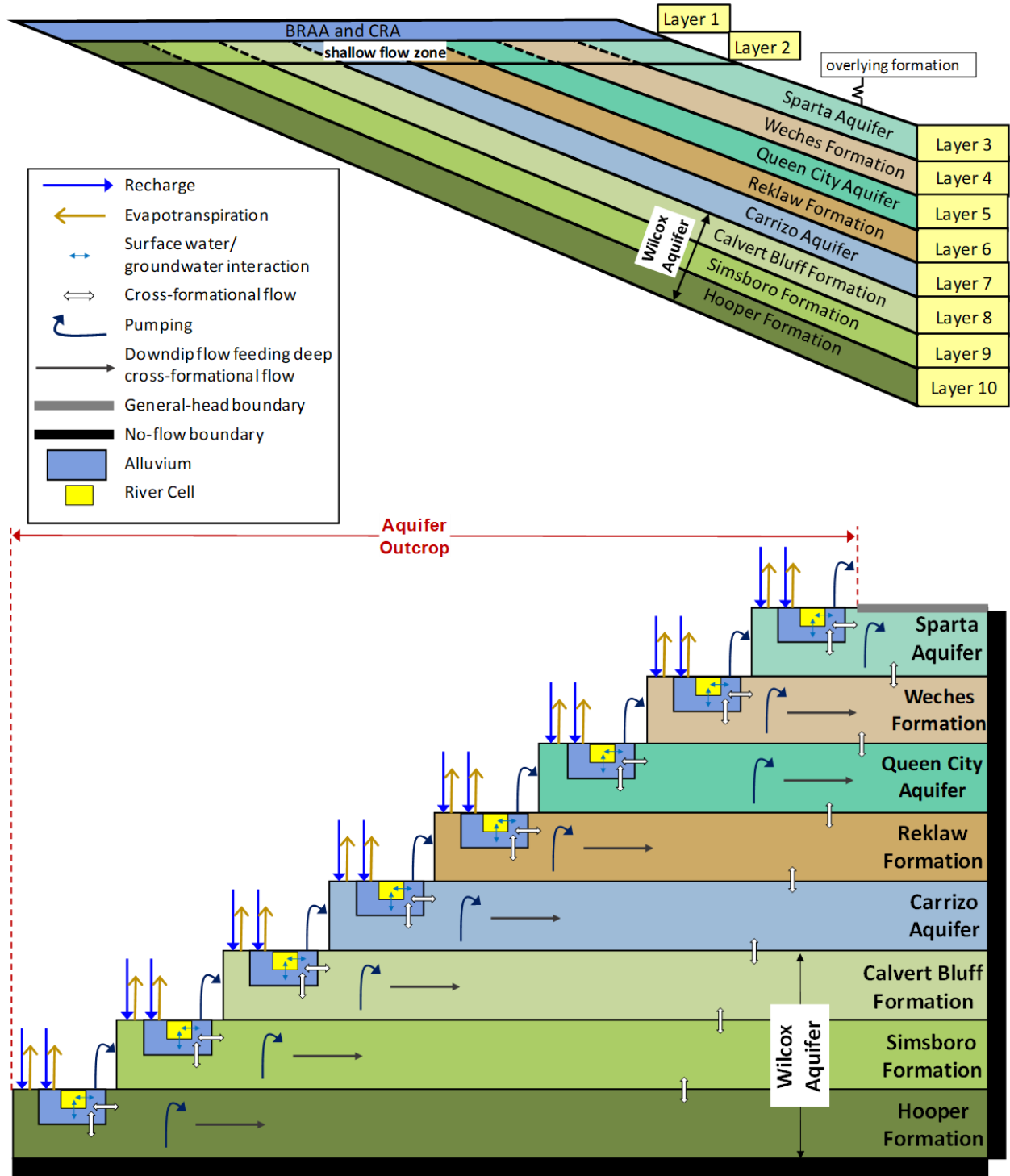
Figure 3.5a. Conceptual groundwater flow model for the updated groundwater availability model for the central portion of the Carrizo-Wilcox, Queen City, and Sparta aquifers.
