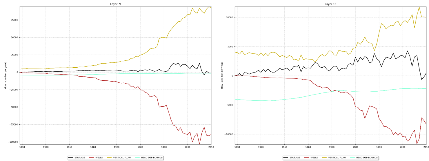
Figure 5.5.2c. Transient water budget for entire the model domain for model layers 9 and 10.
