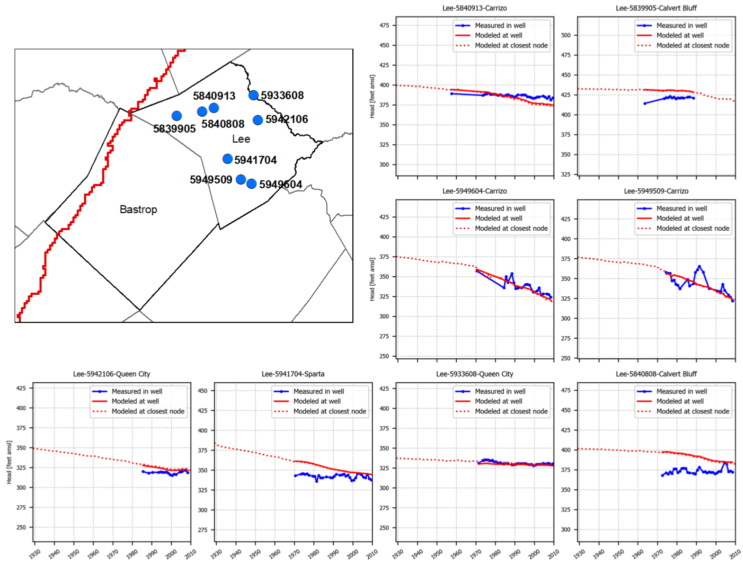
Figure 5.3.6e. Hydrographs showing simulated and measured hydraulic heads (in feet above mean sea level) in the Lost Pines Groundwater Conservation District at eight wells with state well numbers 5840913, 5839905, 5949604, 5949509, 5942106, 5941704, 5933608, and 5840808.
