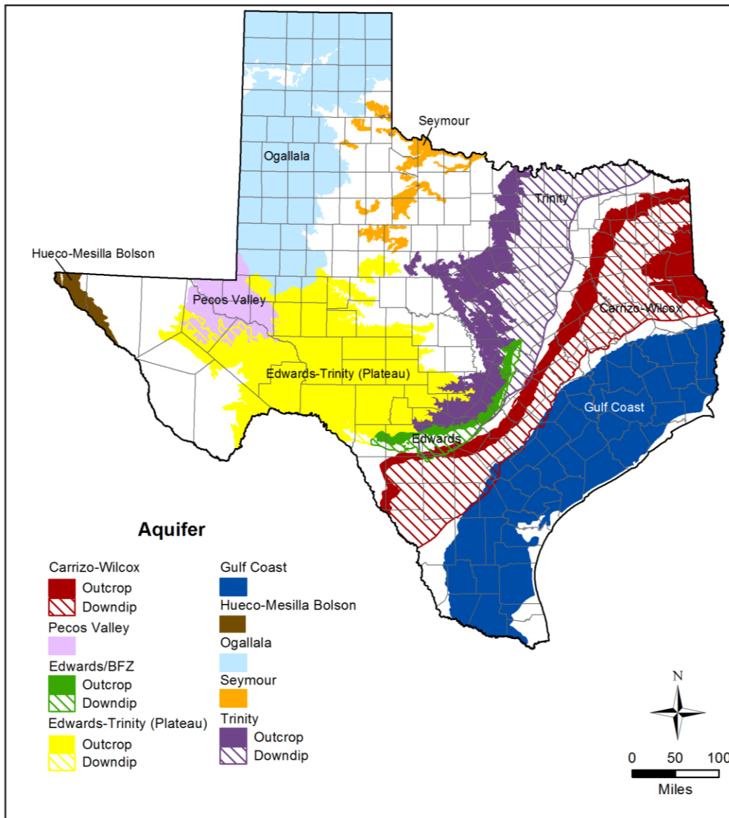
Figure 2.0a. Major Texas aquifers (TWDB, 2006).
