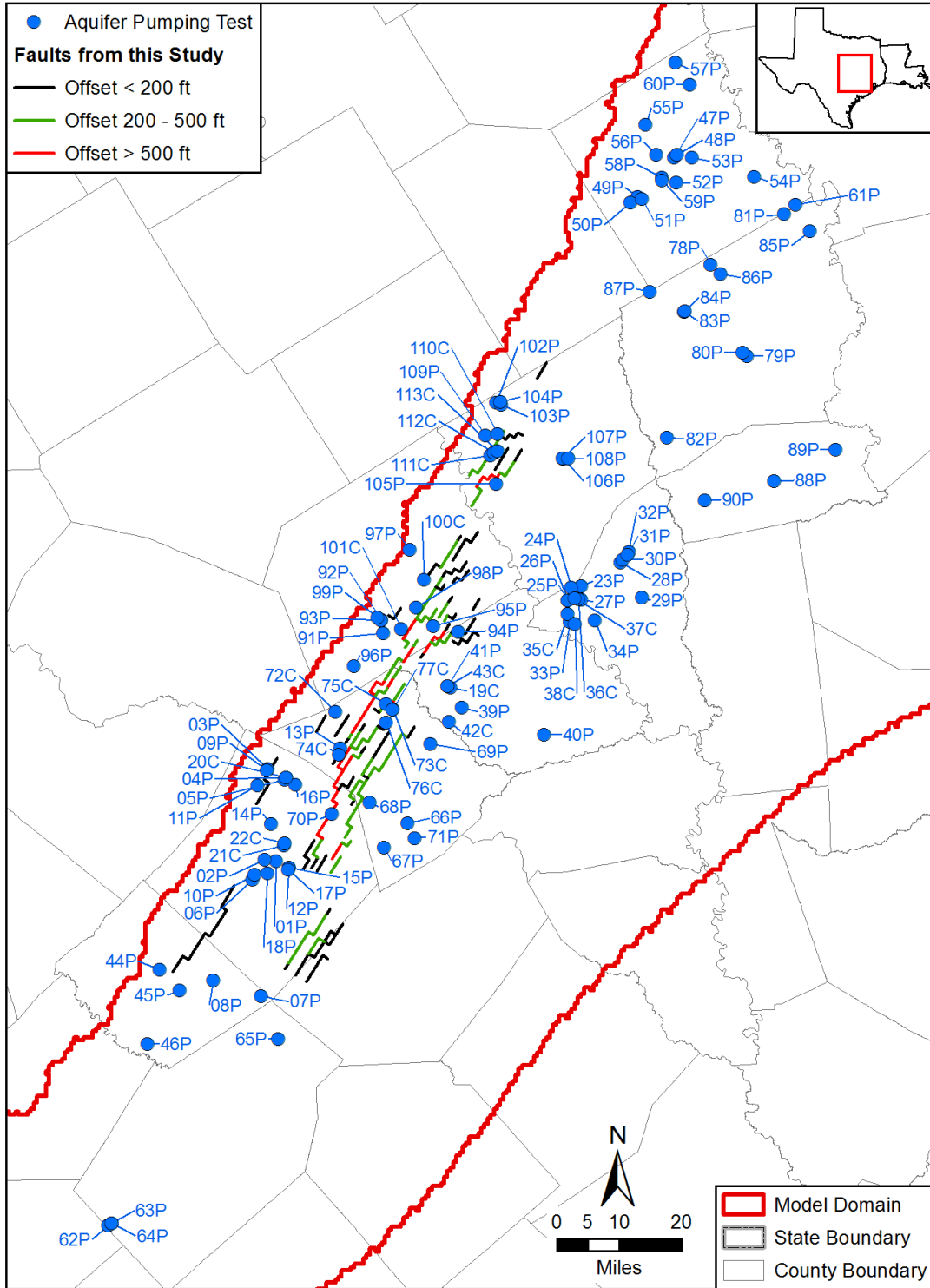
Figure 3.1.4.1a. Location of wells with aquifer pumping test data and the faults identified by this study mapped to the numerical grid of the groundwater availability model for the central portion of the Carrizo-Wilcox, Queen City, and Sparta aquifers.
