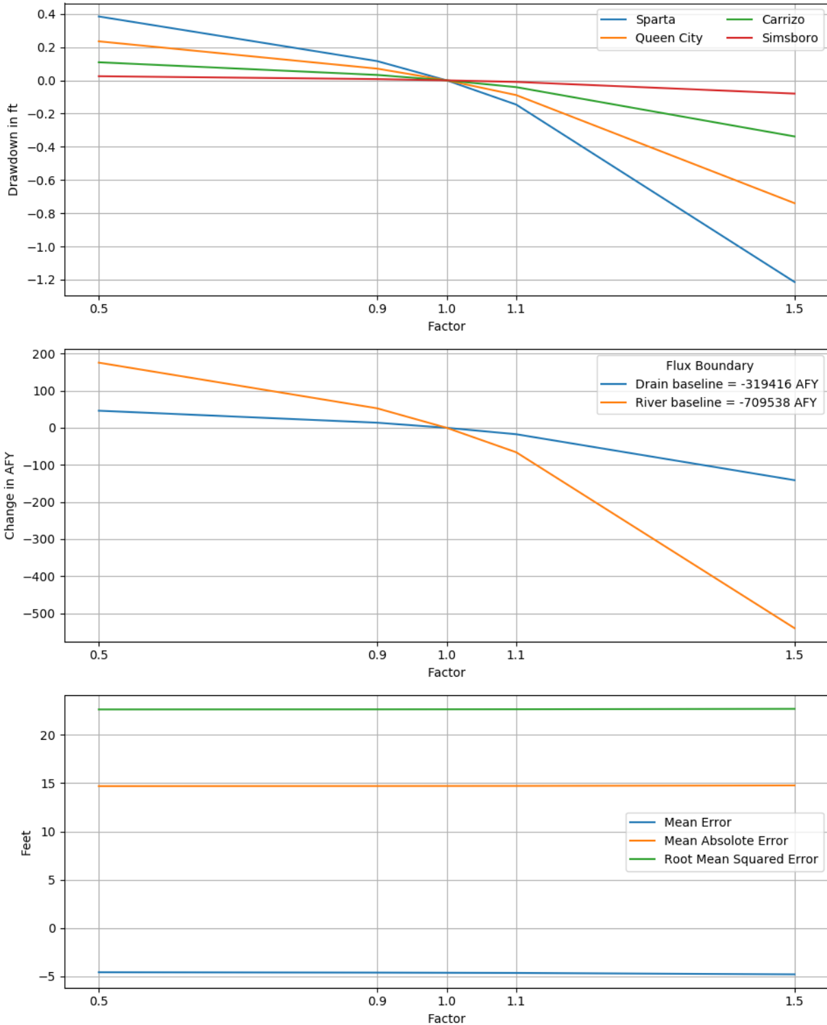
Figure 6.2.2i. Sensitivities of 2010 drawdown in hydrogeologic units (top), hydraulic boundary fluxes (center), and calibration statistics (bottom) to the specific storage of the Sparta Aquifer for the transient model.
