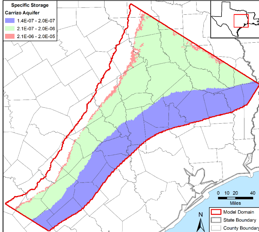
Figure 4.3.2z. Specific storage values in the calibrated model in feet -1 for the Carrizo Aquifer in model layers 2 and 7.
