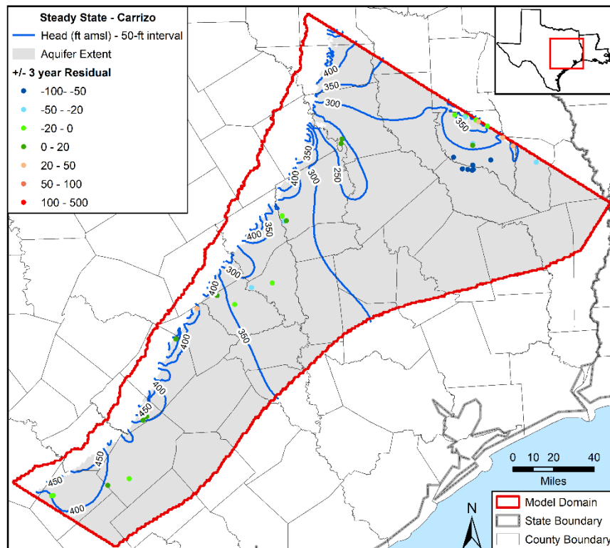
Figure 5.3.4z. Contours in feet (ft) above mean sea level (amsl) developed from simulated hydraulic heads for steady-state conditions in the Carrizo Aquifer with residuals posted.
