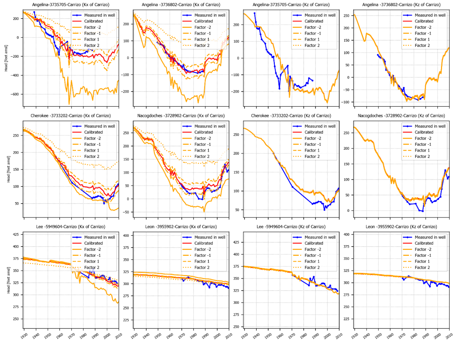
Figure 6.2.2w. Hydrographs showing sensitivity of heads (in feet above mean sea level) to changes in the horizontal and vertical hydraulic conductivity of the Carrizo Aquifer for select wells completed in the Carrizo Aquifer.
