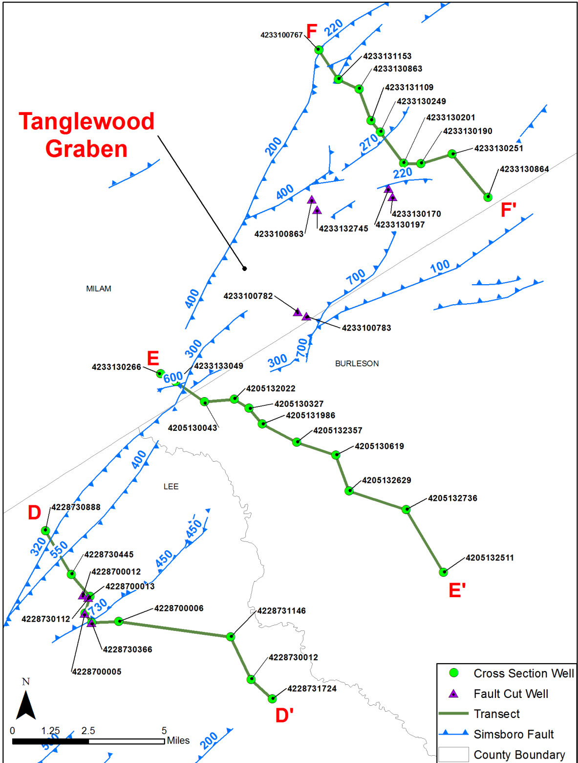
Figure 3.1.2.3a. Simsboro Formation faults and estimated fault offset (in feet) in the Tanglewood Graben in Lee, Milam and Burleson counties. Fault arrows point to the down-thrown side of the fault. The wells are labeled with their American Petroleum Institute number.
