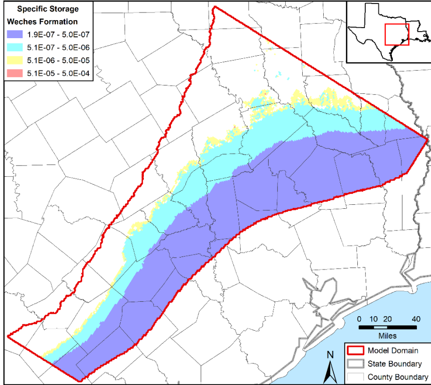
Figure 4.3.2w. Specific storage values in the calibrated model in feet -1 for the Weches Formation in model layers 2 and 4.
