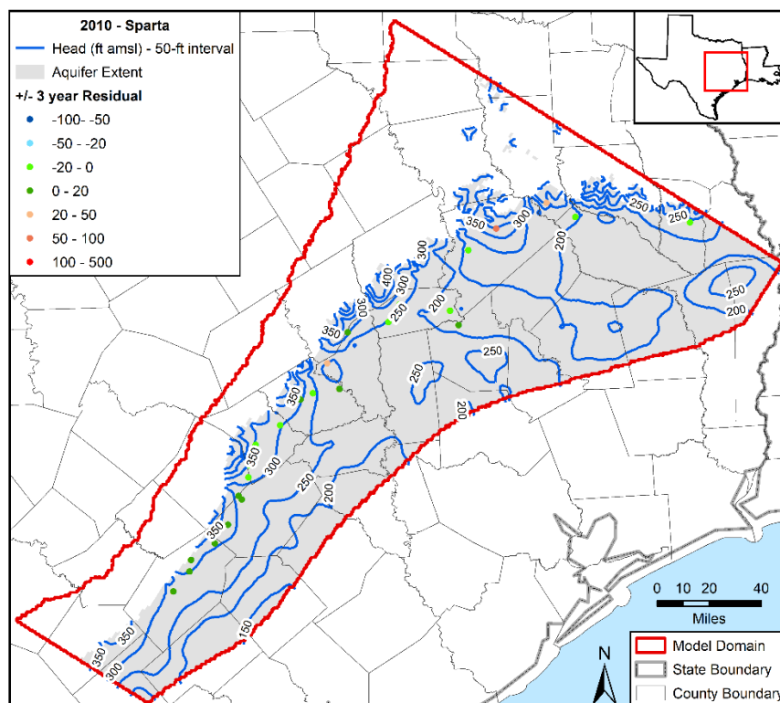
Figure 5.3.4j. Contours in feet (ft) above mean sea level (amsl) developed from simulated hydraulic heads for 2010 in the Sparta Aquifer with residuals posted.
