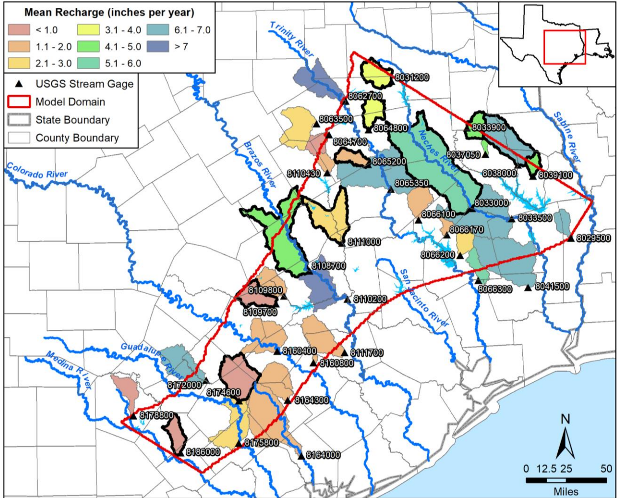
Figure 3.3.3b. Long-term average annual recharge calculated from hydrograph separation using the Baseflow Program. The twelve watersheds outlined in black are those listed in Table 3.3.4a.
