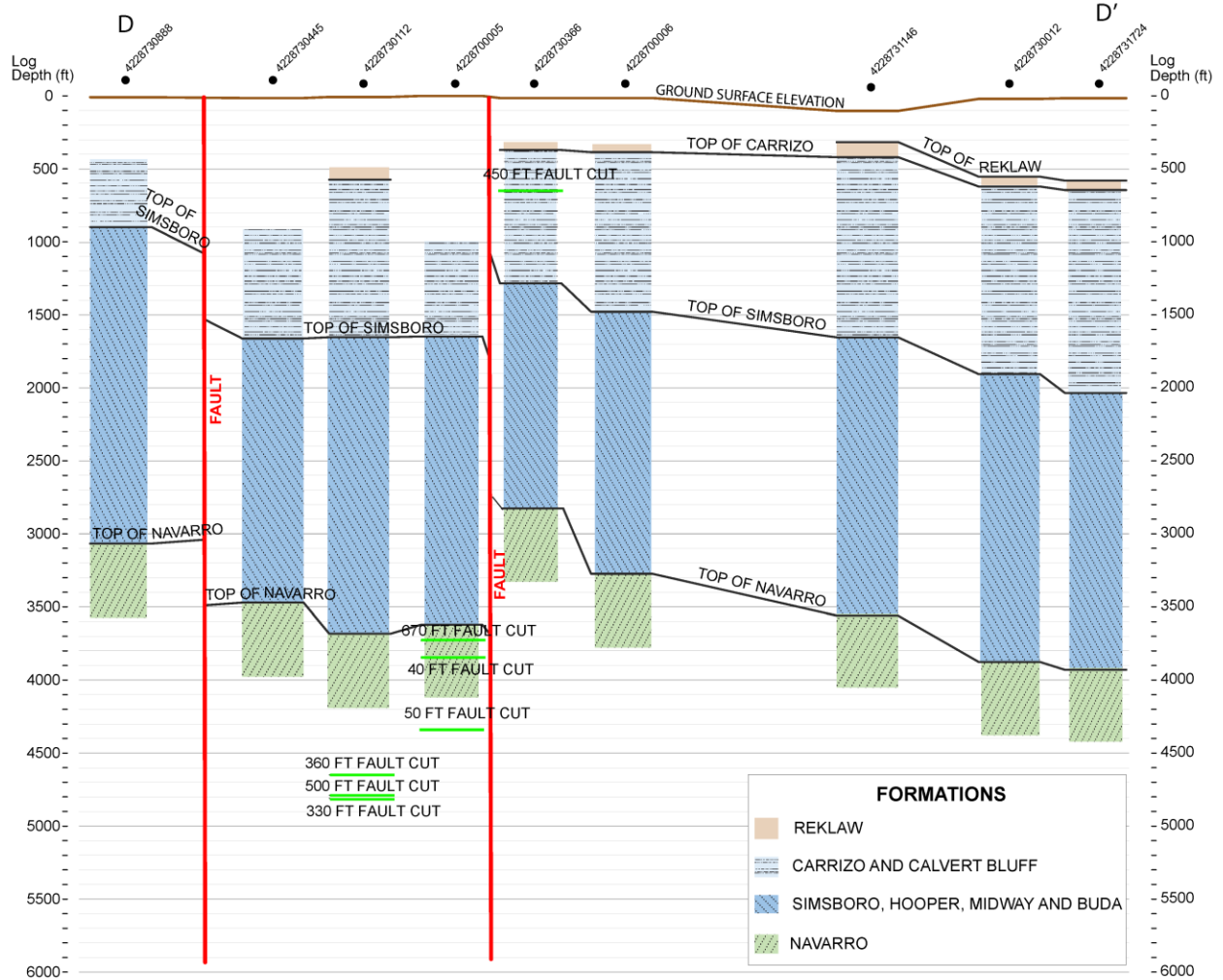
Figure 3.1.2.3b. Cross-section D-D' through the southern portion of the Tanglewood Graben showing the top surface of selected formations and mapped fault locations based on interpretation of geophysical logs in and near cross-section D-D'.
