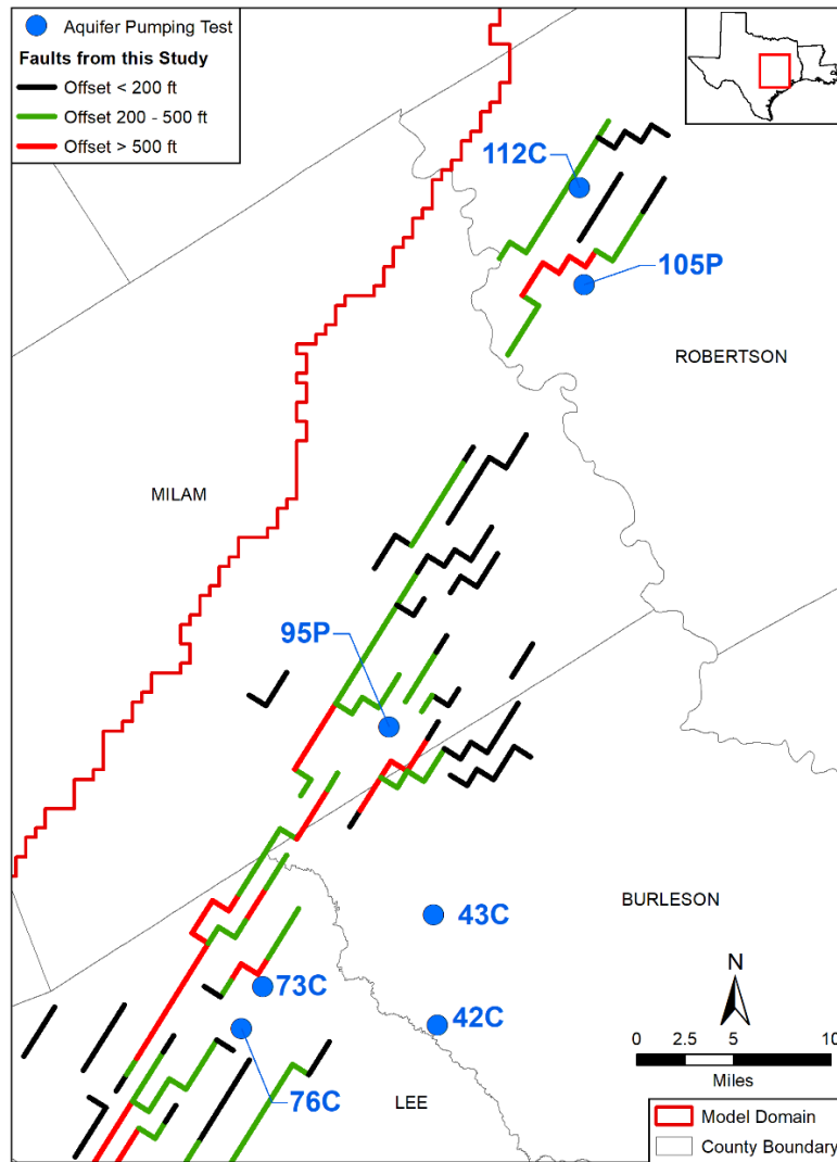
Figure 3.1.4.2a Location of aquifer pumping tests for which T_{Tim} -generated time-drawdown data were analyzed using the Cooper-Jacob method.
