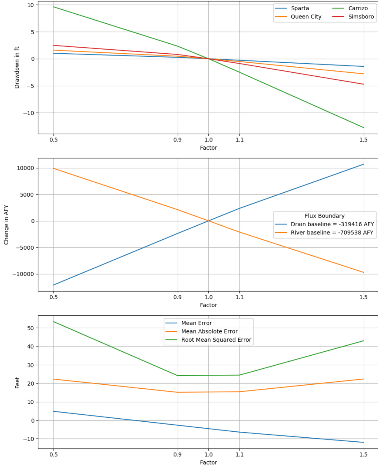
Figure 6.2.2e. Sensitivities of 2010 drawdown in hydrogeologic units (top), hydraulic boundary fluxes (center), and calibration statistics (bottom) to the horizontal hydraulic conductivity of the Carrizo Aquifer for the transient model.
