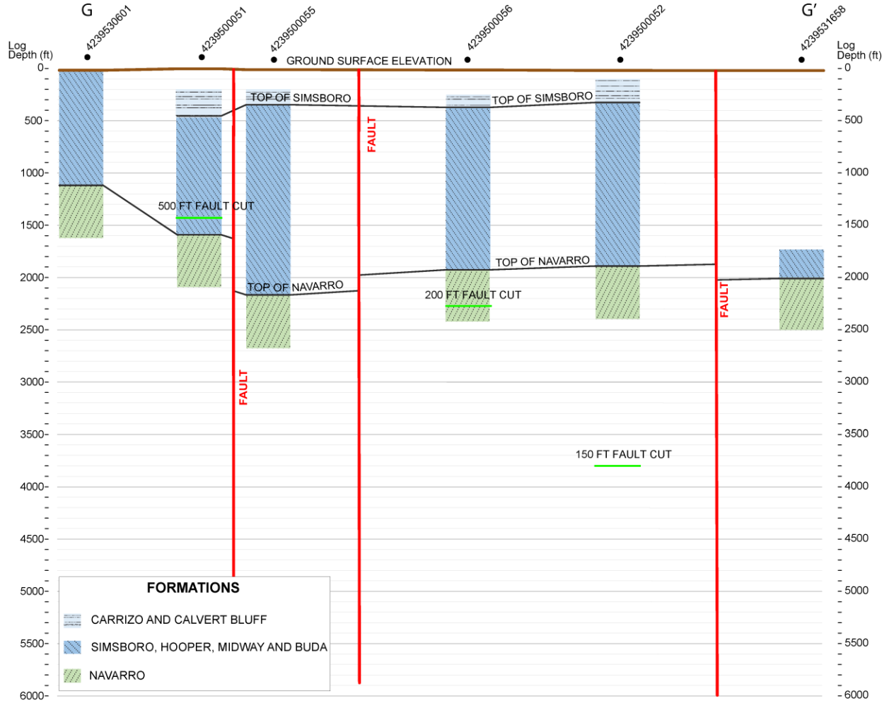
Figure 3.1.2.4b. Cross-section G-G' through the Calvert Graben showing the top surface of selected formations and mapped fault locations based on interpretation of geophysical logs in and near cross-section G-G'.
