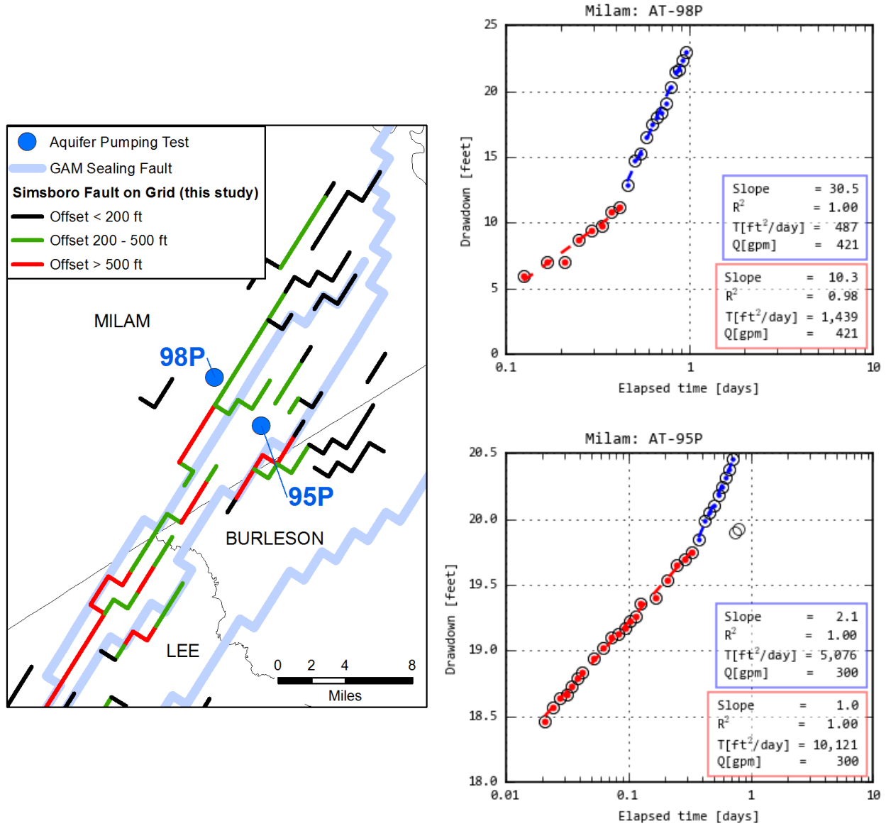
Figure 3.1.4.1c. Location of aquifer pumping tests near faults in Milam County that produced a CJSL-calculated late-time transmissivity value less than the early-time transmissivity value, which provides a line of evidence that faults could be affecting groundwater flow. For aquifer tests AT-98P and AT-95P, the values for the late-to early-time transmissivity ratio are 0.33 and 0.50, respectively.
