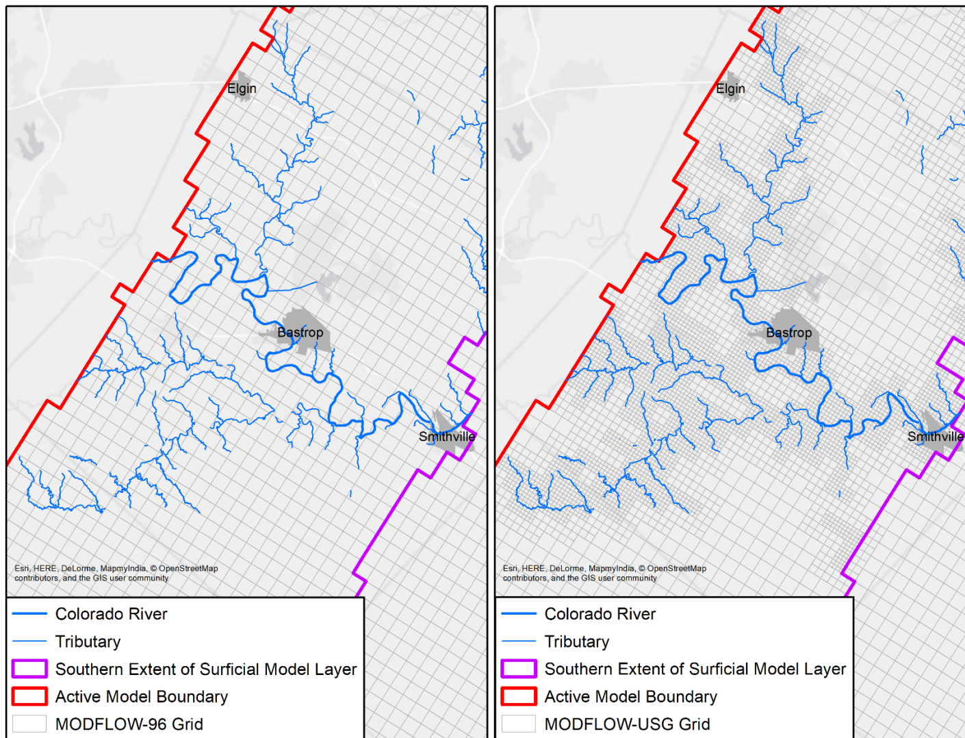
Figure 3.4.2a. Numerical grid showing the uniform 1-mile by 1-mile square grid cells in the 2004 groundwater availability model for the central portion of the Carrizo-Wilcox, Queen City, and Sparta aquifers (left) and the locally-refined grid with 0.25-mile by 0.25-mile square grid cells in the vicinity of the Colorado River and its major tributaries in the updated model (right).
