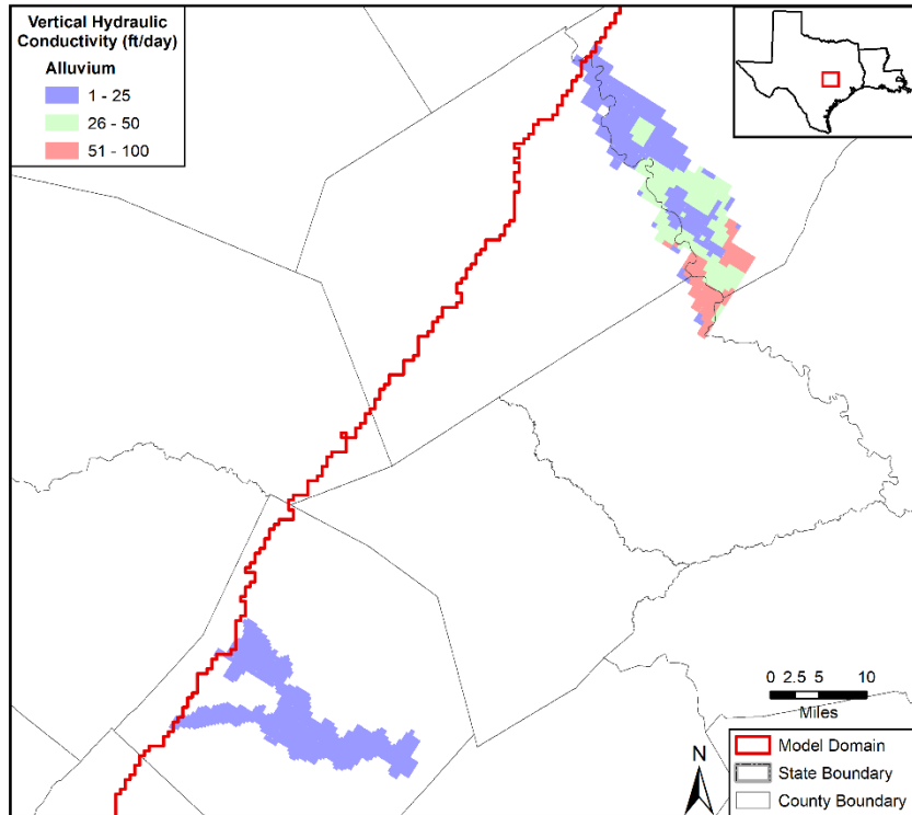
Figure 4.3.2k. Vertical hydraulic conductivity values in the calibrated model in feet per day (ft/day) for the Colorado and Brazos rivers alluvium in model layer 1.
