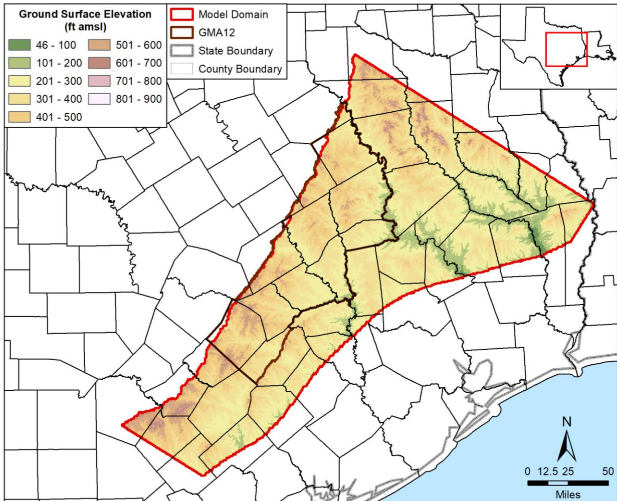
Figure 2.3a. Topographic map of the active model area (United States Geological Survey, 2014).
