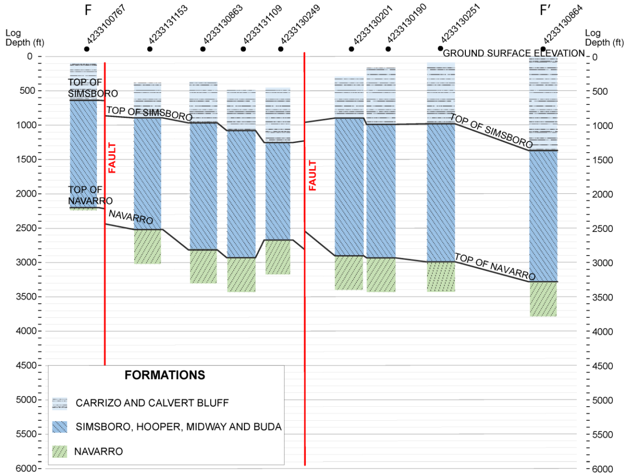
Figure 3.1.2.3d. Cross-section F-F' through the northeastern portion of the Tanglewood Graben showing the top surface of selected formations and mapped fault locations based on interpretation of geophysical logs in and near cross-section F-F'.
