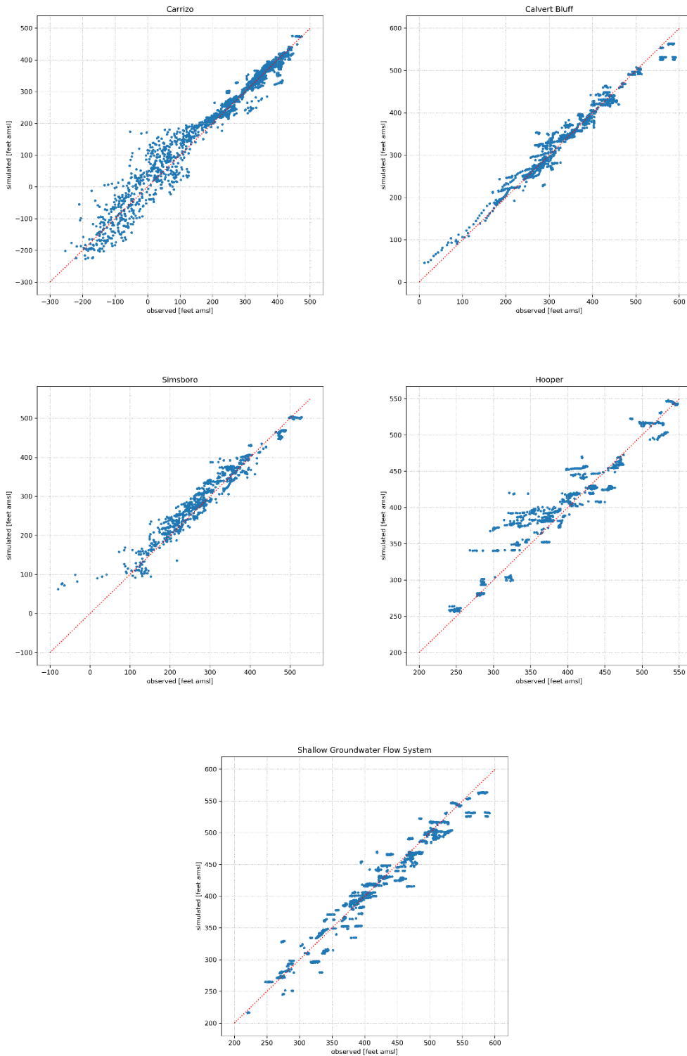
Figure 5.3.3j. Scatter plots of simulated versus observed hydraulic heads for all calibration targets in all wells in the Carrizo Aquifer, the Calvert Bluff Formation, the Simsboro Formation, the Hooper Formation and the shallow groundwater flow system for the transient period 1930 to 2010.
