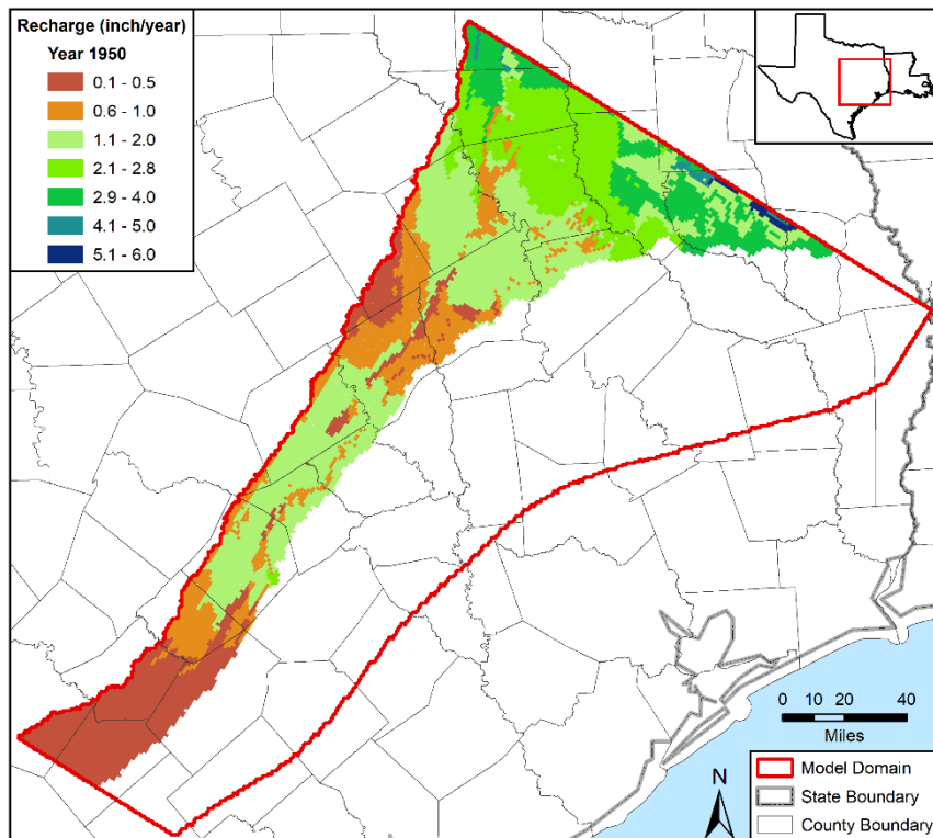
Figure 4.6b. Spatial distribution of recharge in inches per year for 1950.
