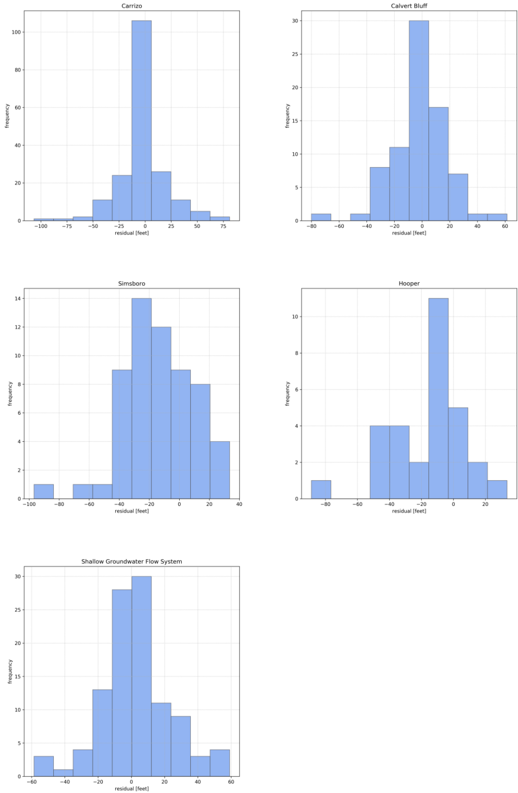
Figure 5.3.3f. Histograms of the average hydraulic head residuals for wells in the Carrizo Aquifer, the Calvert Bluff Formation, the Simsboro Aquifer, the Hooper Aquifer, and the shallow groundwater flow system for the transient period 1930 to 2010.
