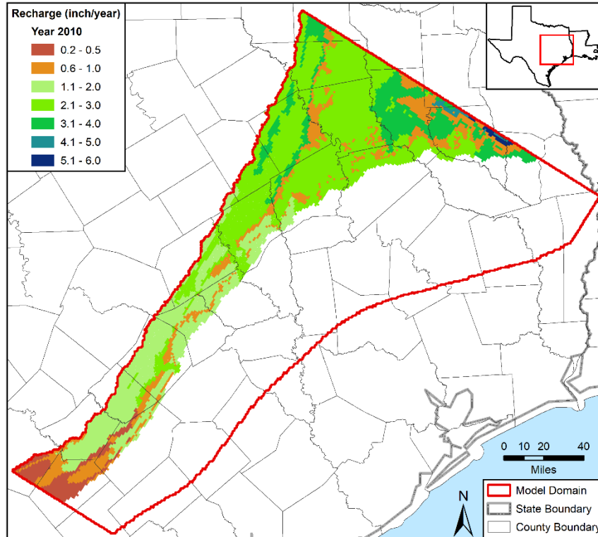
Figure 4.6e. Spatial distribution of recharge in inches per year for 2010.
