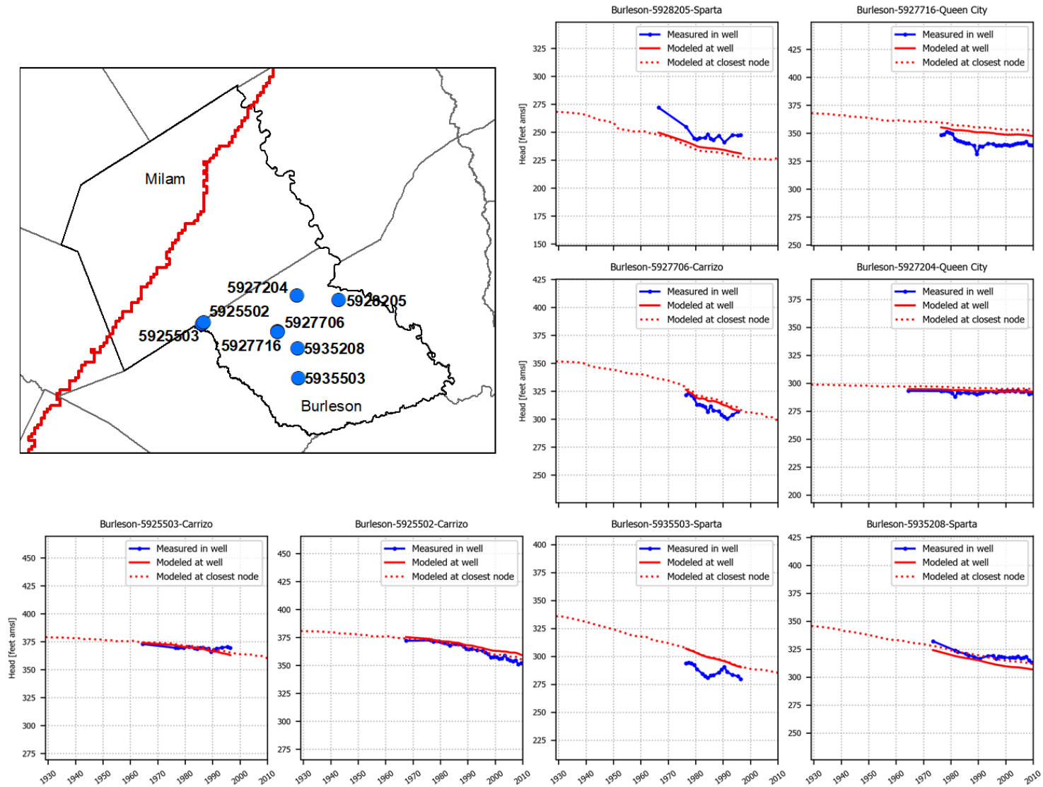
Figure 5.3.6b. Hydrographs showing simulated and measured hydraulic heads (in feet above mean sea level) in the Post Oak Savannah Groundwater Conservation District at eight wells with state well numbers 5928205, 5927716, 5927706, 5927204, 5925503, 5925502, 5935503, 5935208.
