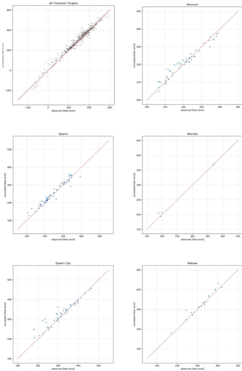
Figure 5.3.3c. Scatter plots of the average simulated versus average observed hydraulic heads at wells with calibration targets in the entire model domain, the Brazos River alluvium, the Sparta Aquifer, the Weches Formation, the Queen City Aquifer, and the Reklaw Formation for the transient period 1930 to 2010.
