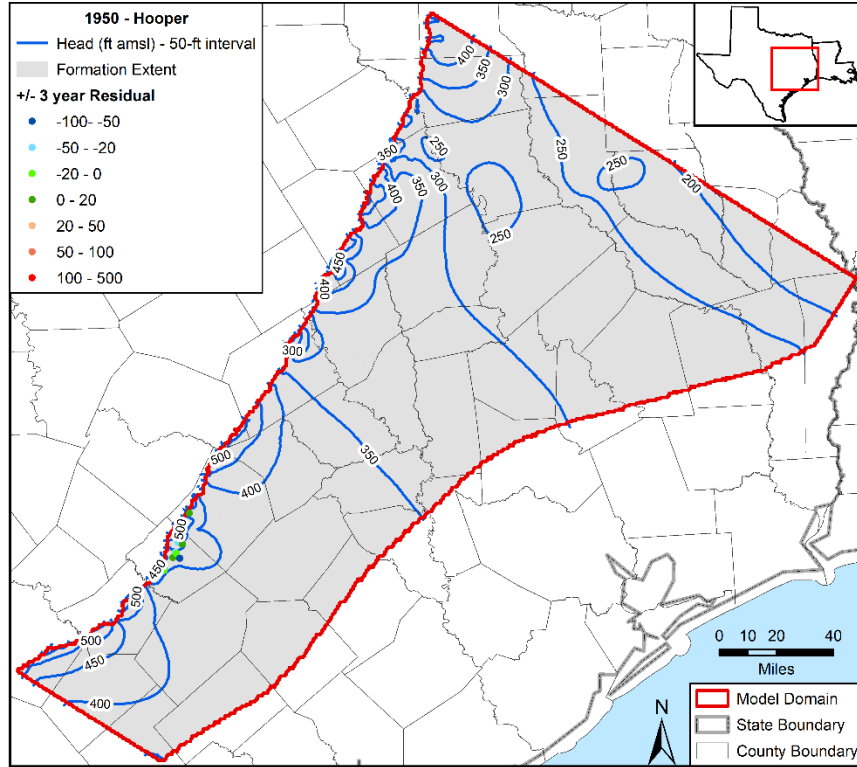
Figure 5.3.4pp. Contours in feet (ft) above mean sea level (amsl) developed from simulated hydraulic heads for 1950 in the Hooper Formation with residuals posted.
