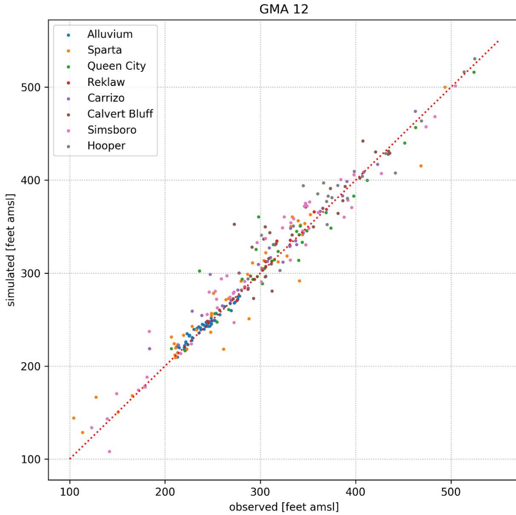
Figure 5.3.3b. Scatter plot of the average simulated versus average observed hydraulic heads at each of the 267 wells in Groundwater Management Area 12 with calibration targets for the transient period 1930 to 2010.
