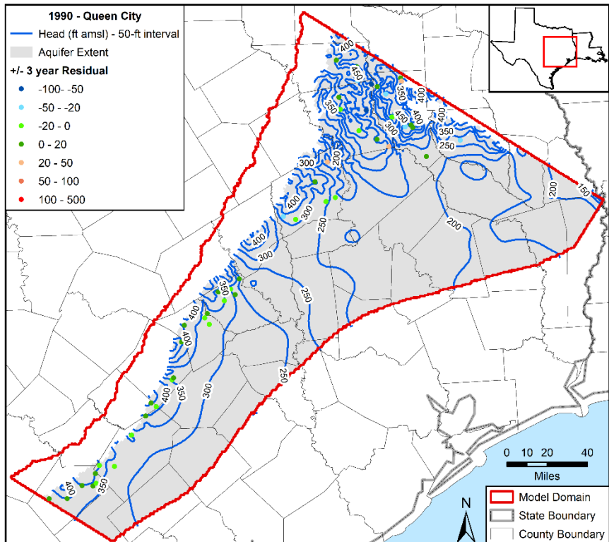
Figure 5.3.4s. Contours in feet (ft) above mean sea level (amsl) developed from simulated hydraulic heads for 1990 in the Queen City Aquifer with residuals posted.
