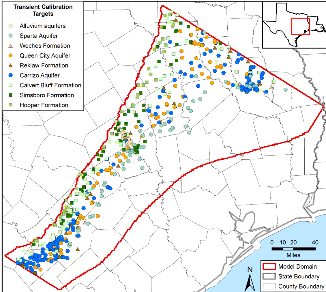
Figure 5.2d. Spatial distribution of hydraulic heads targets for transient conditions from 1930 to 2010.
