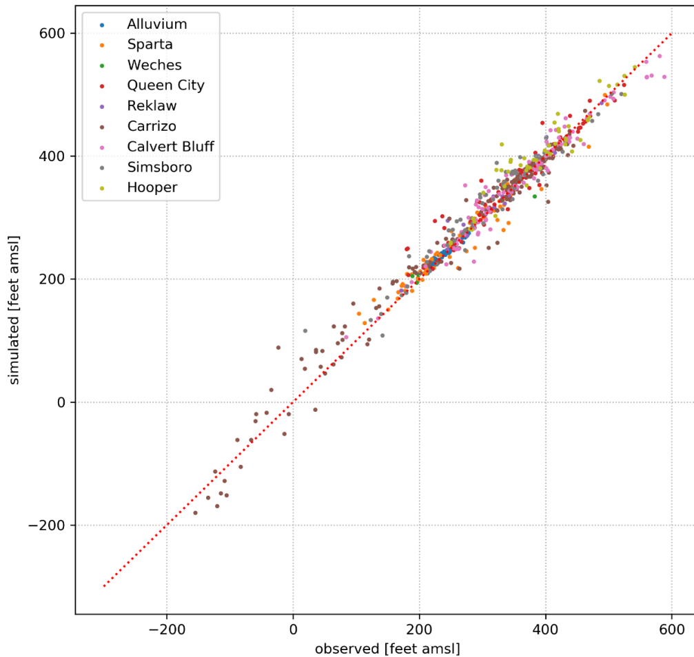
Figure 5.3.3a. Scatter plot of the average simulated versus average observed hydraulic heads at each of the 467 wells in the entire model domain with calibration targets for the transient period 1930 to 2010.
