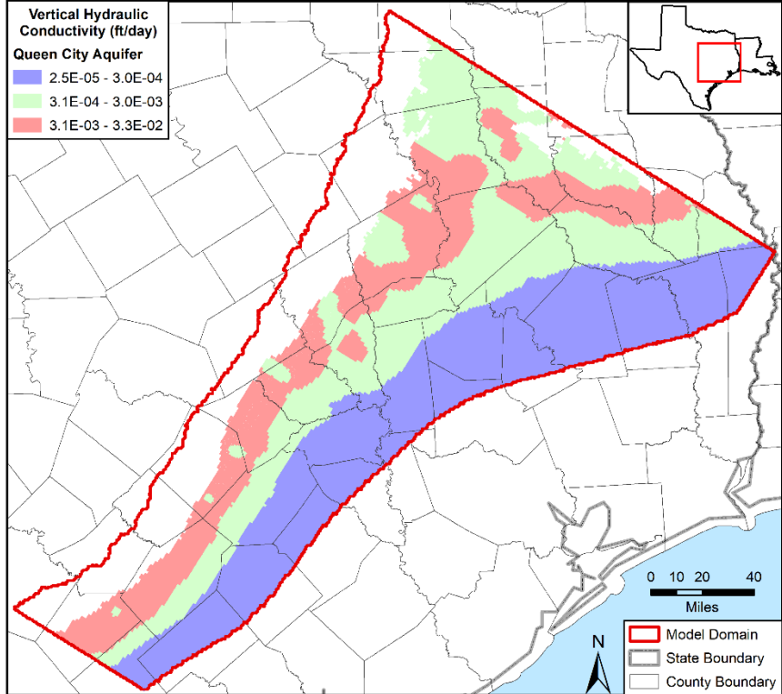
Figure 4.3.2n. Vertical hydraulic conductivity values in the calibrated model in feet per day (ft/day) for the Queen City Aquifer in model layers 2 and 5.
