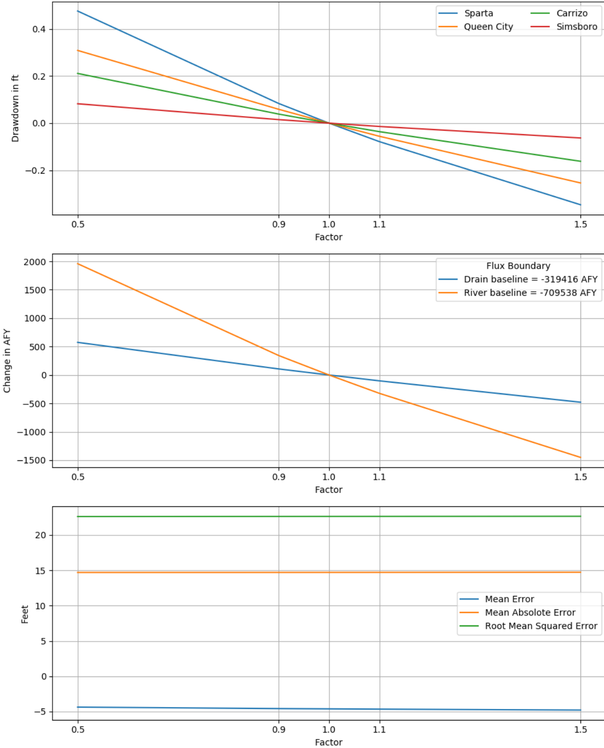
Figure 6.2.2j. Sensitivities of 2010 drawdown in hydrogeologic units (top), hydraulic boundary fluxes (center), and calibration statistics (bottom) to the specific yield of the Sparta Aquifer for the transient model.
