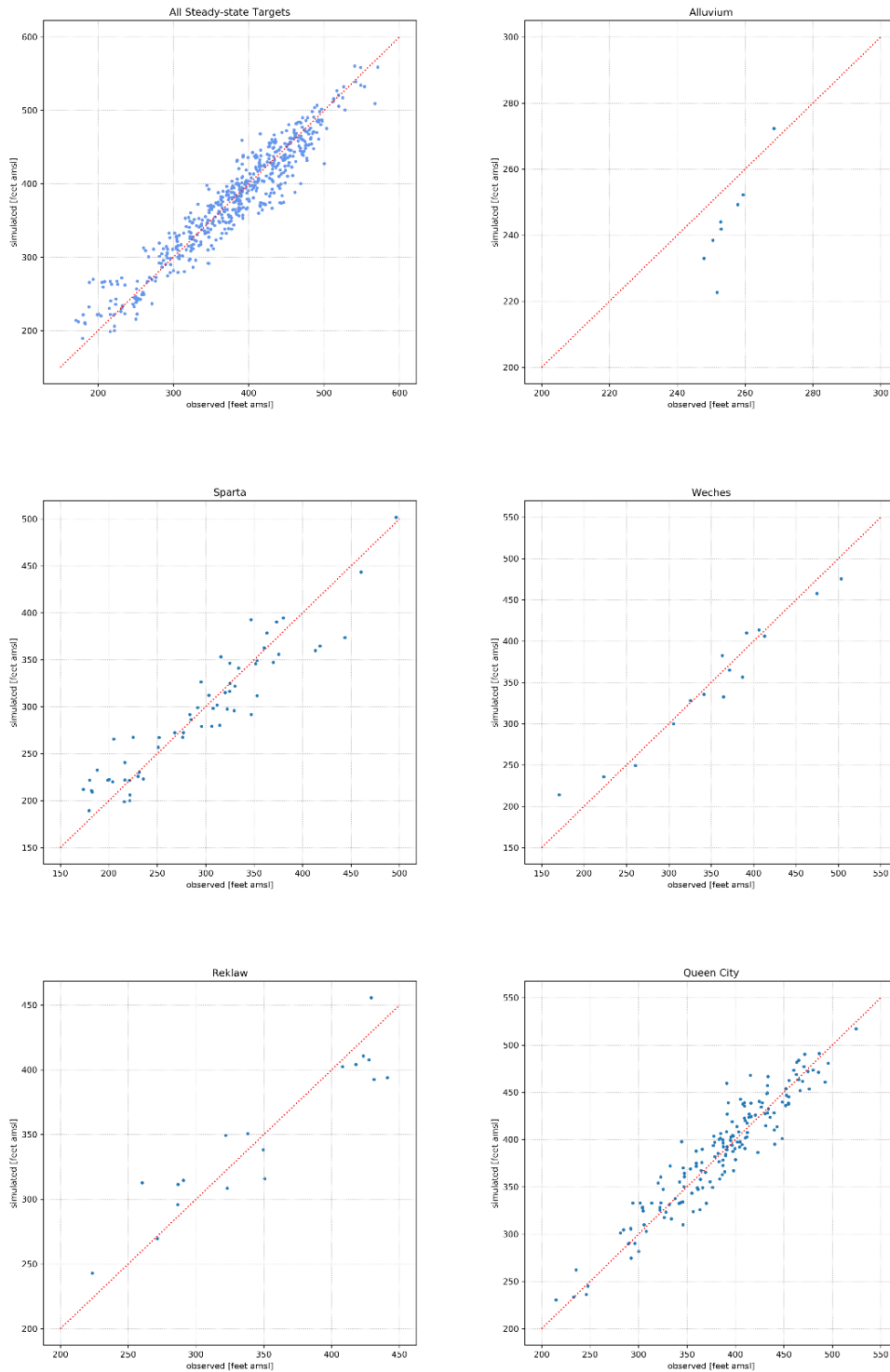
Figure 5.3.2b. Scatter plots of simulated versus observed hydraulic heads for calibration targets in the entire model domain, the Brazos River alluvium, the Sparta Aquifer, the Weches Formation, the Queen City Aquifer, and the Reklaw Formation across the entire model domain for the steady-state period.
