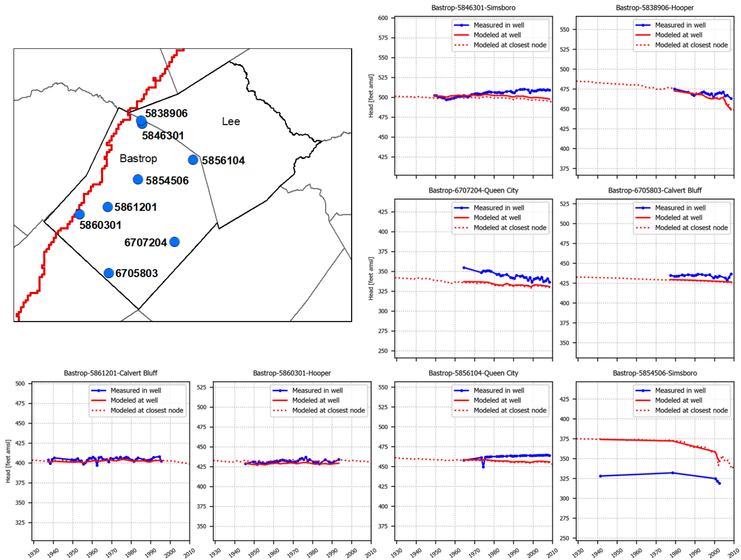
Figure 5.3.6f. Hydrographs showing simulated and measured hydraulic heads (in feet above mean sea level) in the Lost Pines Groundwater Conservation District at eight wells with state well numbers 5846301, 5838906, 6707204, 6705803, 5861201, 5860301, 5856104, and 5854506.
