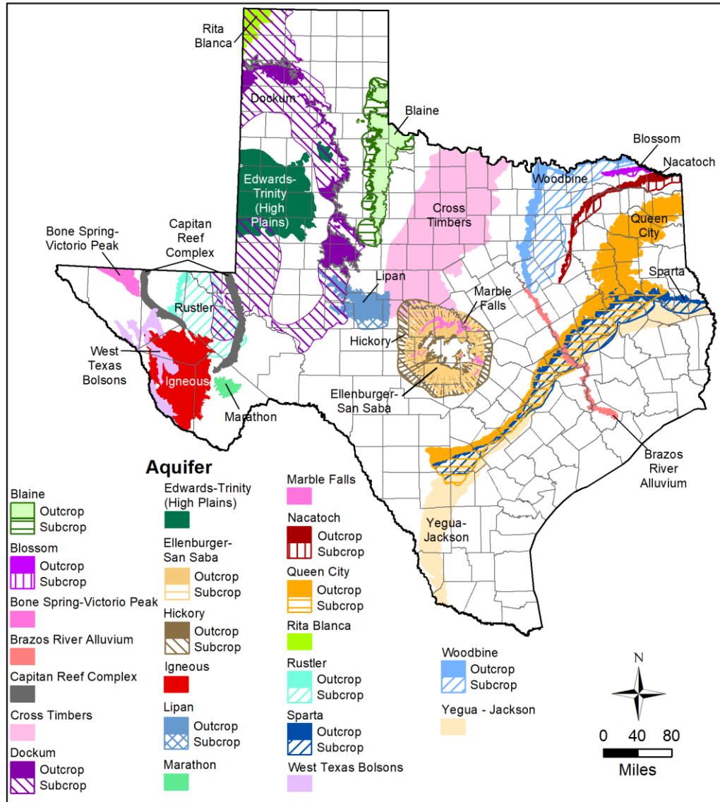
Figure 2.0b. Minor Texas aquifers (TWDB, 2017a).
