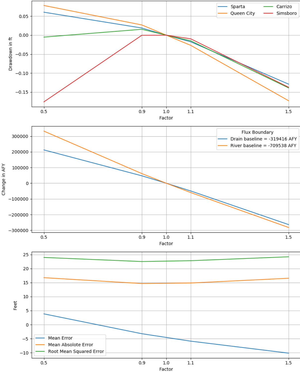
Figure 6.2.2q. Sensitivities of 2010 drawdown in hydrogeologic units (top), hydraulic boundary fluxes (center), and calibration statistics (bottom) to the recharge rate for the transient model.
