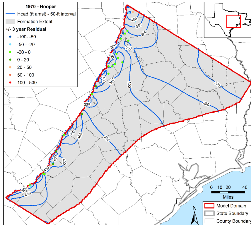
Figure 5.3.4qq. Contours in feet (ft) above mean sea level (amsl) developed from simulated hydraulic heads for 1970 in the Hooper Formation with residuals posted.
