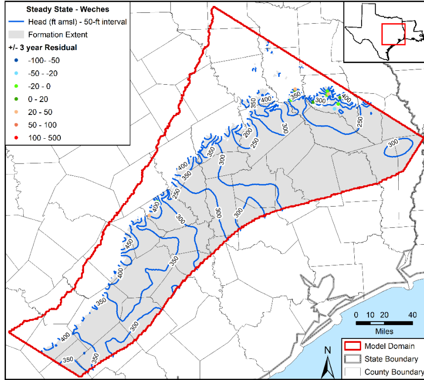
Figure 5.3.4k. Contours in feet (ft) above mean sea level (amsl) developed from simulated hydraulic heads for steady-state conditions in the Weches Formation with residuals posted.
