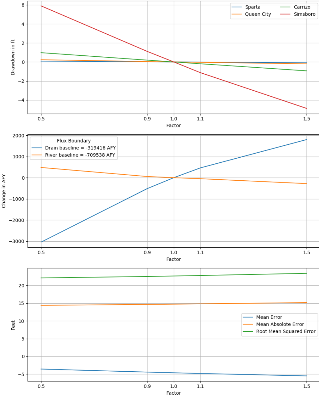
Figure 6.2.2h. Sensitivities of 2010 drawdown in hydrogeologic units (top), hydraulic boundary fluxes (center), and calibration statistics (bottom) to the vertical hydraulic conductivity of the Simsboro Formation for the transient model.
