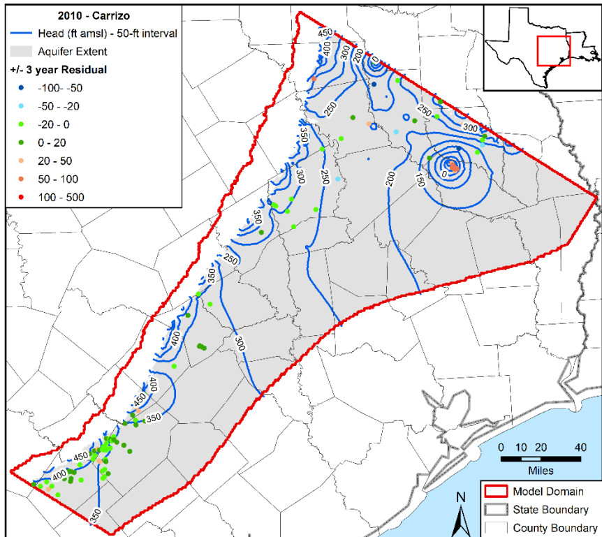
Figure 5.3.4dd. Contours in feet (ft) above mean sea level (amsl) developed from simulated hydraulic heads for 2010 in the Carrizo Aquifer with residuals posted.
