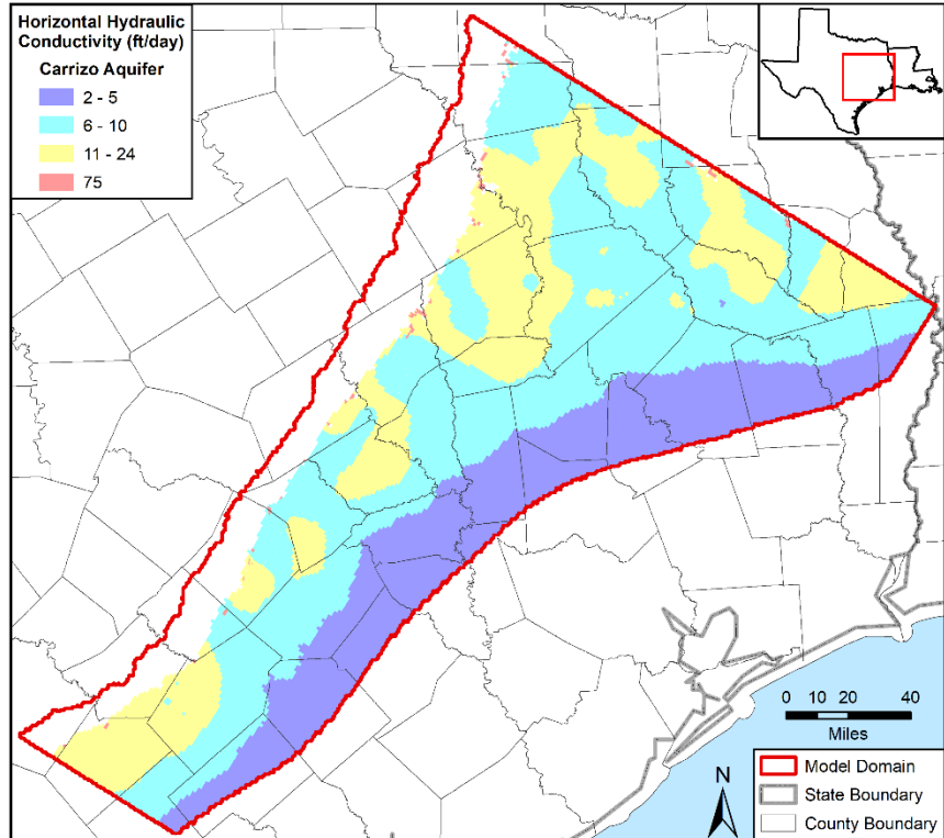
Figure 4.3.2f. Horizontal hydraulic conductivity values in the calibrated model in feet per day (ft/day) for the Carrizo Aquifer in model layers 2 and 7.
