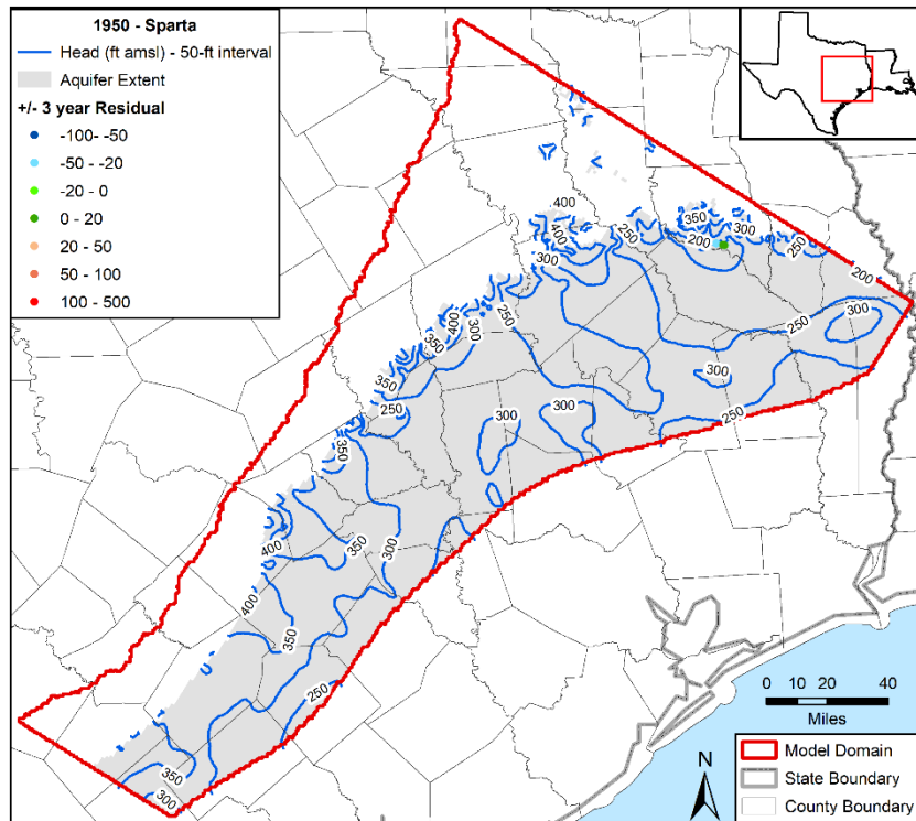
Figure 5.3.4g. Contours in feet (ft) above mean sea level (amsl) developed from simulated hydraulic heads for 1950 in the Sparta Aquifer with residuals posted.
