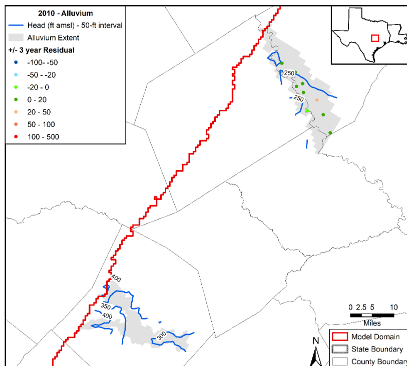
Figure 5.3.4e. Contours in feet (ft) above mean sea level (amsl) developed from simulated hydraulic heads for 2010 in the Colorado and Brazos rivers alluvium with residuals for the Brazos River alluvium posted.
