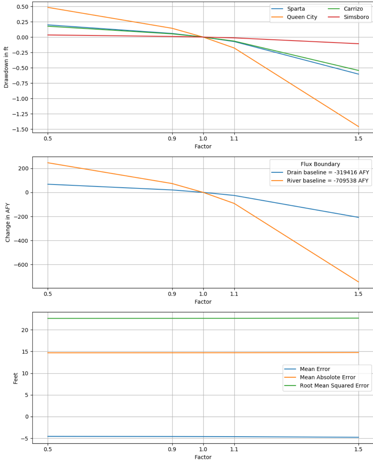
Figure 6.2.2k. Sensitivities of 2010 drawdown in hydrogeologic units (top), hydraulic boundary fluxes (center), and calibration statistics (bottom) to the specific storage of the Queen City Aquifer for the transient model.
