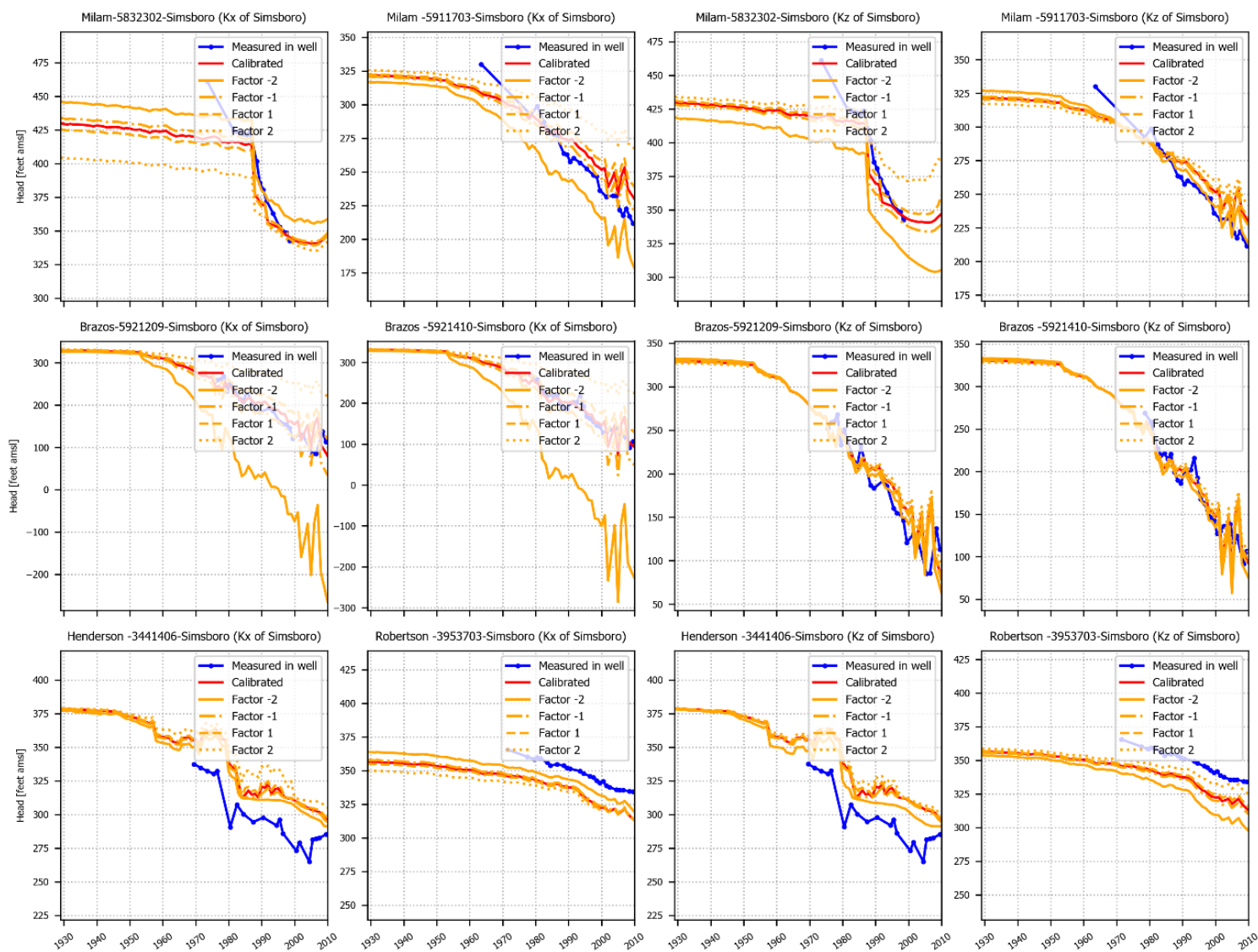
Figure 6.2.2x. Hydrographs showing sensitivity of heads (in feet above mean sea level) to changes in the horizontal and vertical hydraulic conductivity of the Simsboro Formation for select wells completed in the Simsboro Formation.
