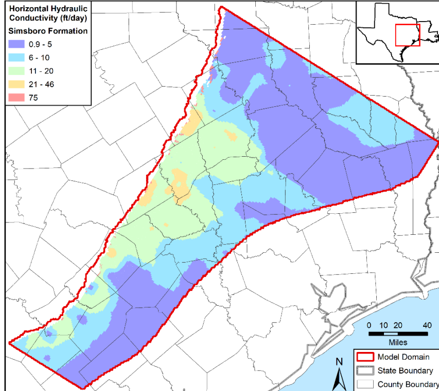
Figure 4.3.2h. Horizontal hydraulic conductivity values in the calibrated model in feet per day (ft/day) for the Simsboro Formation in model layers 2 and 9.
