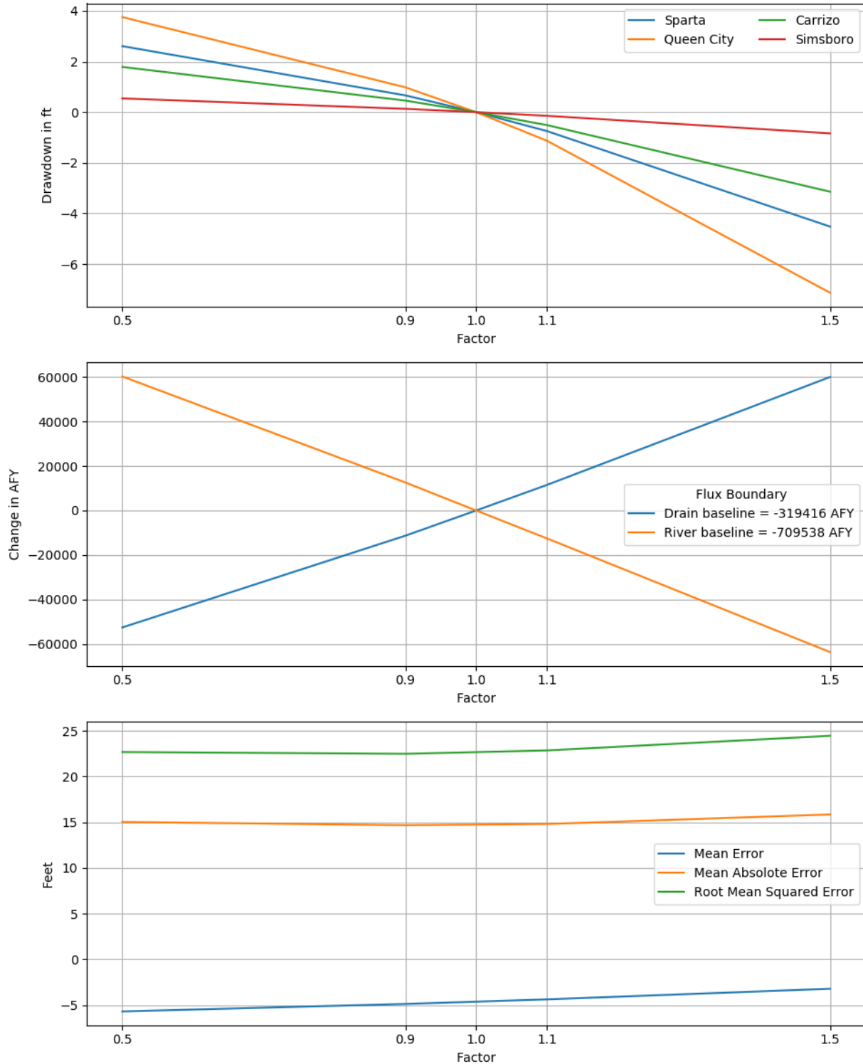
Figure 6.2.2c. Sensitivities of 2010 drawdown in hydrogeologic units (top), hydraulic boundary fluxes (center), and calibration statistics (bottom) to the horizontal hydraulic conductivity of the Queen City Aquifer for the transient model.
