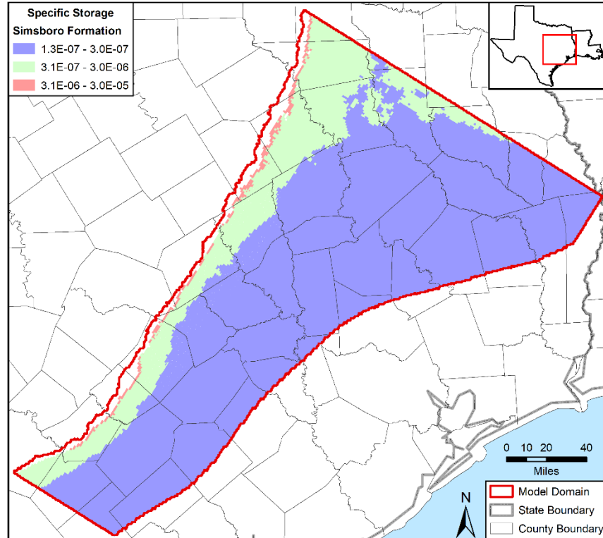
Figure 4.3.2bb. Specific storage values in the calibrated model in feet -1 for the Simsboro Formation in model layers 2 and 9.
