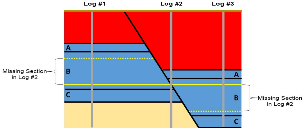
Figure 3.1.2c. Schematic representation of how fault-cut logs are identified. Log #1 intersects all three portions of Sections A, B and C. Log #2 intersects all of Section A, the top part of Section B on the down-thrown side and the bottom part of Section B on the up-thrown side, and all of Section C. Log #3 intersects all three portions of Sections A, B, and C. Using all three of these logs together, geologists can piece together missing sections within geologic units. The amount of missing section is referred to as a fault cut and can be used as a quantitative way to characterize the offset associated with faults.
