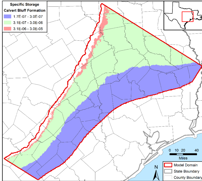
Figure 4.3.2aa. Specific storage values in the calibrated model in feet -1 for the Calvert Bluff Formation model layers 2 and 8.
