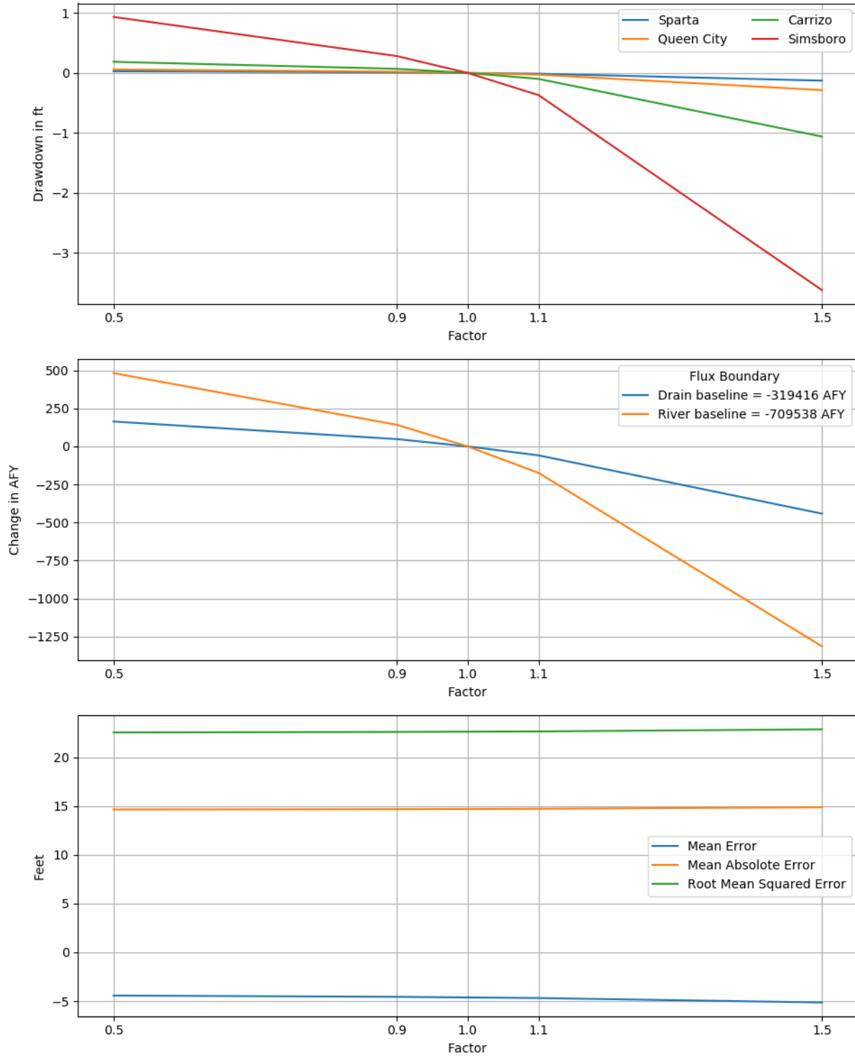
Figure 6.2.2o. Sensitivities of 2010 drawdown in hydrogeologic units (top), hydraulic boundary fluxes (center), and calibration statistics (bottom) to the specific storage of the Simsboro Formation for the transient model.
