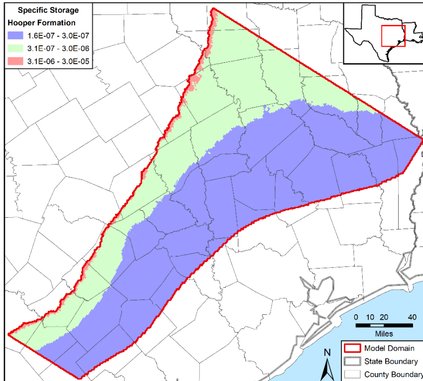
Figure 4.3.2cc. Specific storage values in the calibrated model in feet -1 for the Hooper Formation in model layers 2 and 10.
