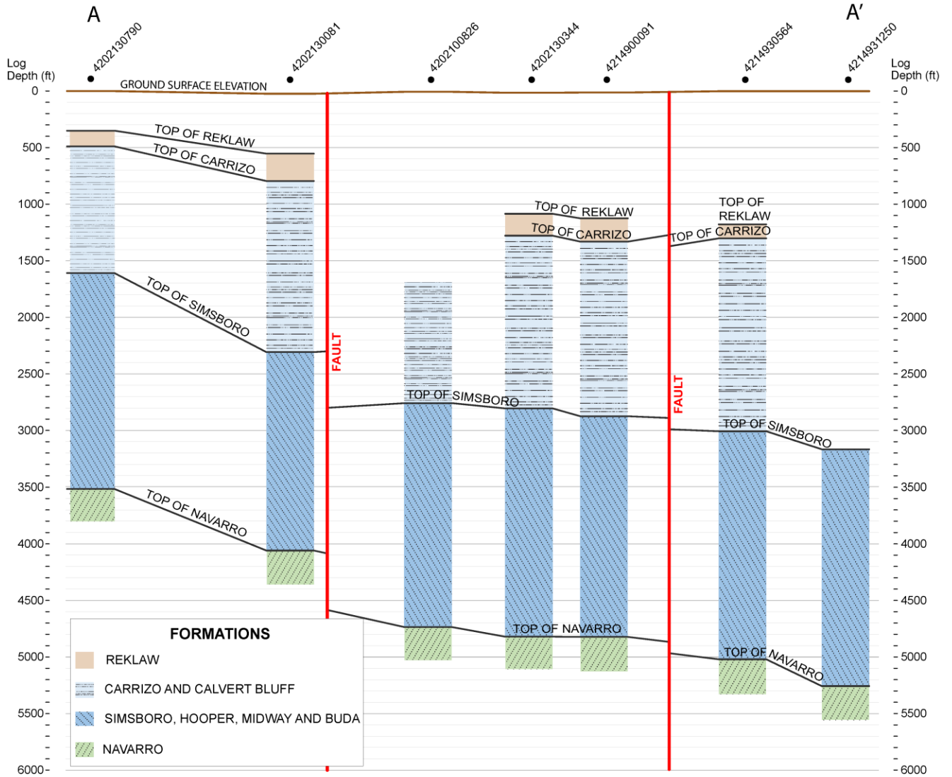
Figure 3.1.2.1b. Cross-section A-A' through the Kovar Complex showing the top surface of selected formations and mapped fault locations based on interpretation of geophysical logs in and near cross-section A-A'.
