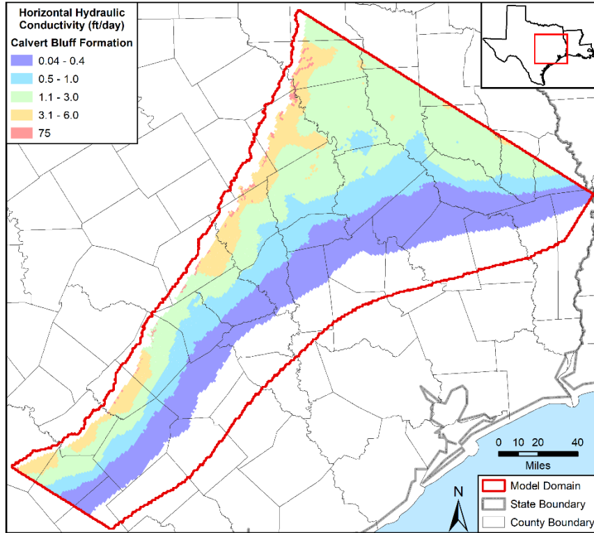
Figure 4.3.2g. Horizontal hydraulic conductivity values in the calibrated model in feet per day (ft/day) for the Calvert Bluff Formation in model layers 2 and 8.
