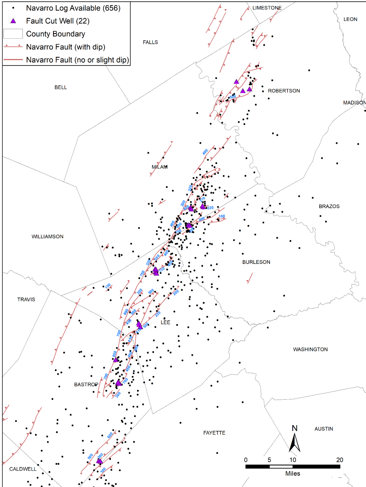
Figure 3.1.2b. Faults mapped onto the top of the Navarro Group determined primarily from the top of the Navarro Group picks from 656 geophysical logs with fault traces mapped on Geologic Atlas of Texas sheets (Barnes, 1970, 1979, 1981). Fault arrows point to the down-thrown side of the fault. Numerical values indicate fault offset in feet.
