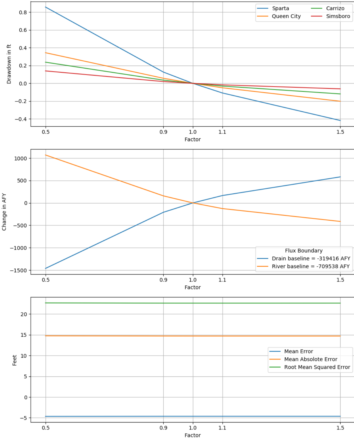
Figure 6.2.2b. Sensitivities of 2010 drawdown in hydrogeologic units (top), hydraulic boundary fluxes (center), and calibration statistics (bottom) to the vertical hydraulic conductivity of the Sparta Aquifer for the transient model.
