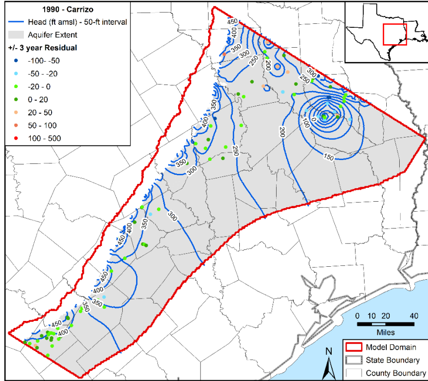
Figure 5.3.4cc. Contours in feet (ft) above mean sea level (amsl) developed from simulated hydraulic heads for 1990 in the Carrizo Aquifer with residuals posted.
