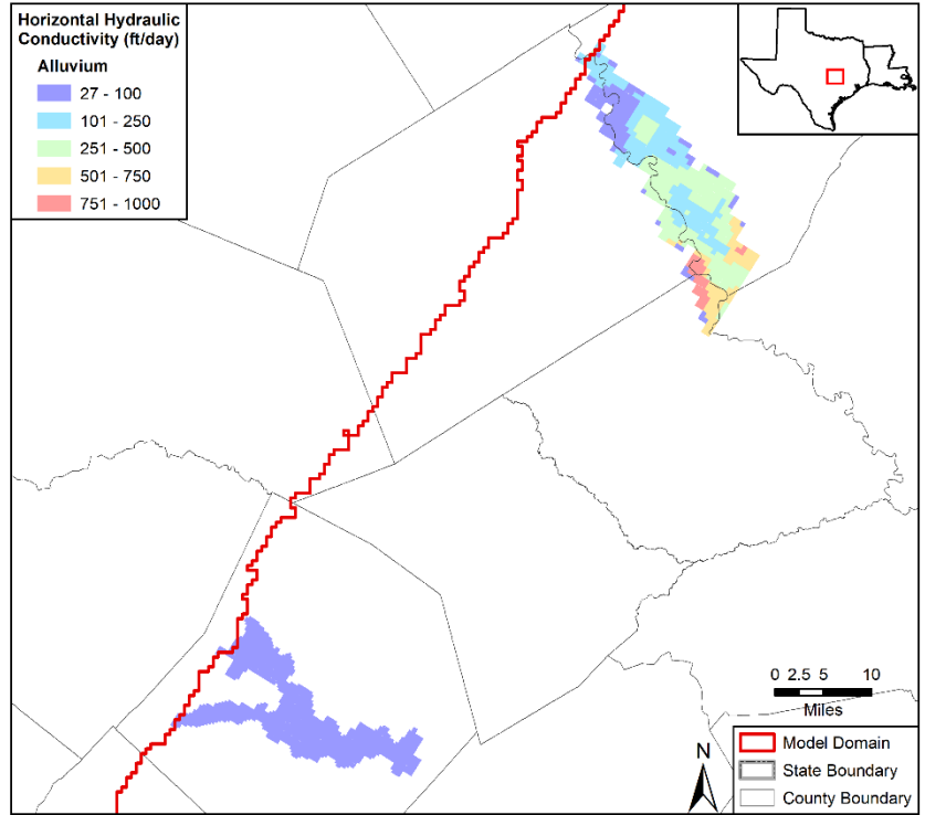
Figure 4.3.2a. Horizontal hydraulic conductivity values in the calibrated model in feet per day (ft/day) for the Colorado and Brazos rivers alluvium in model layer 1.
