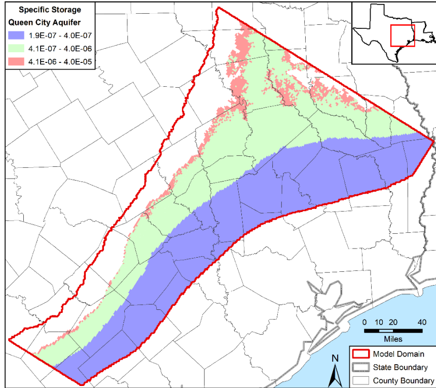
Figure 4.3.2x. Specific storage values in the calibrated model in feet -1 for the Queen City Aquifer in model layers 2 and 5.
