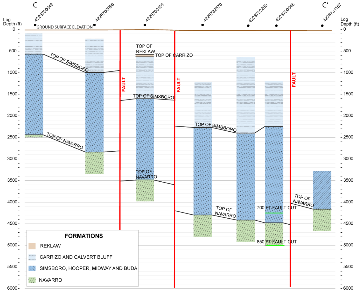
Figure 3.1.2.2c. Cross-section C-C' through the northeastern portion of the Paige Graben showing the top surface of selected formations and mapped fault locations based on interpretation of geophysical logs in and near cross-section C-C'.
