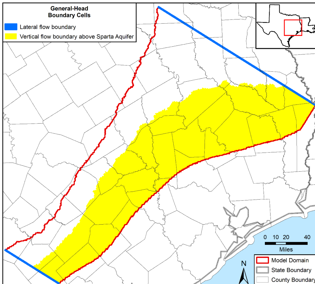
Figure 4.7a. Areal footprint showing the locations of general-head boundary cells.
