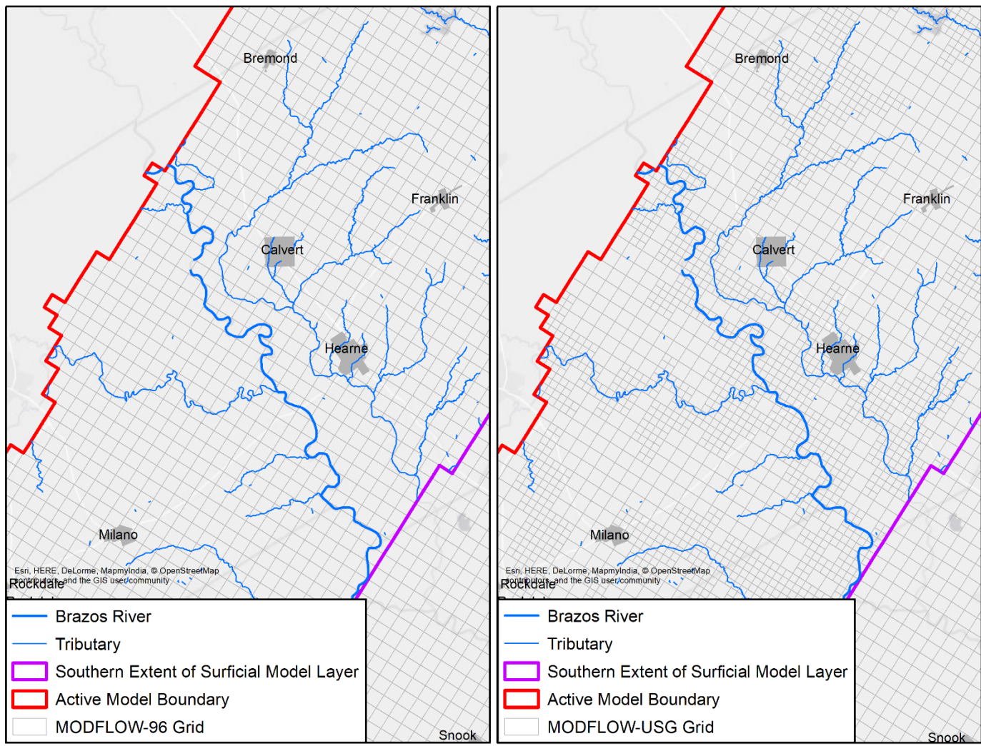
Figure 3.4.2b. Numerical grid showing the uniform 1-mile by 1-mile square grid cells in the 2004 groundwater availability model for the central portion of the Carrizo-Wilcox, Queen City, and Sparta aquifers (left) and the locally-refined grid with 0.5-mile by 0.5-mile square grid cells in the vicinity of the Brazos River and its major tributaries in the updated model (right).
