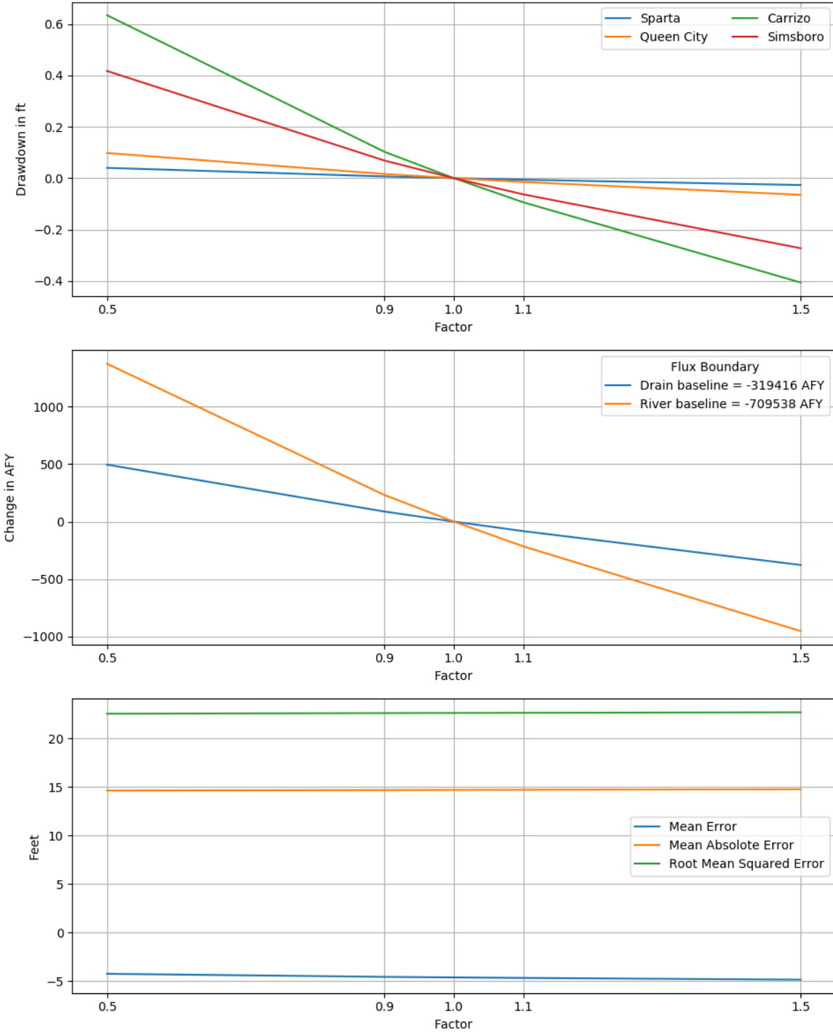
Figure 6.2.2n. Sensitivities of 2010 drawdown in hydrogeologic units (top), hydraulic boundary fluxes (center), and calibration statistics (bottom) to the specific yield of the Carrizo Aquifer for the transient model.
