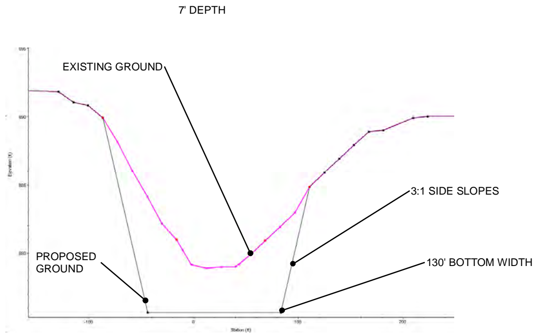
CROSS SECTION I-I
