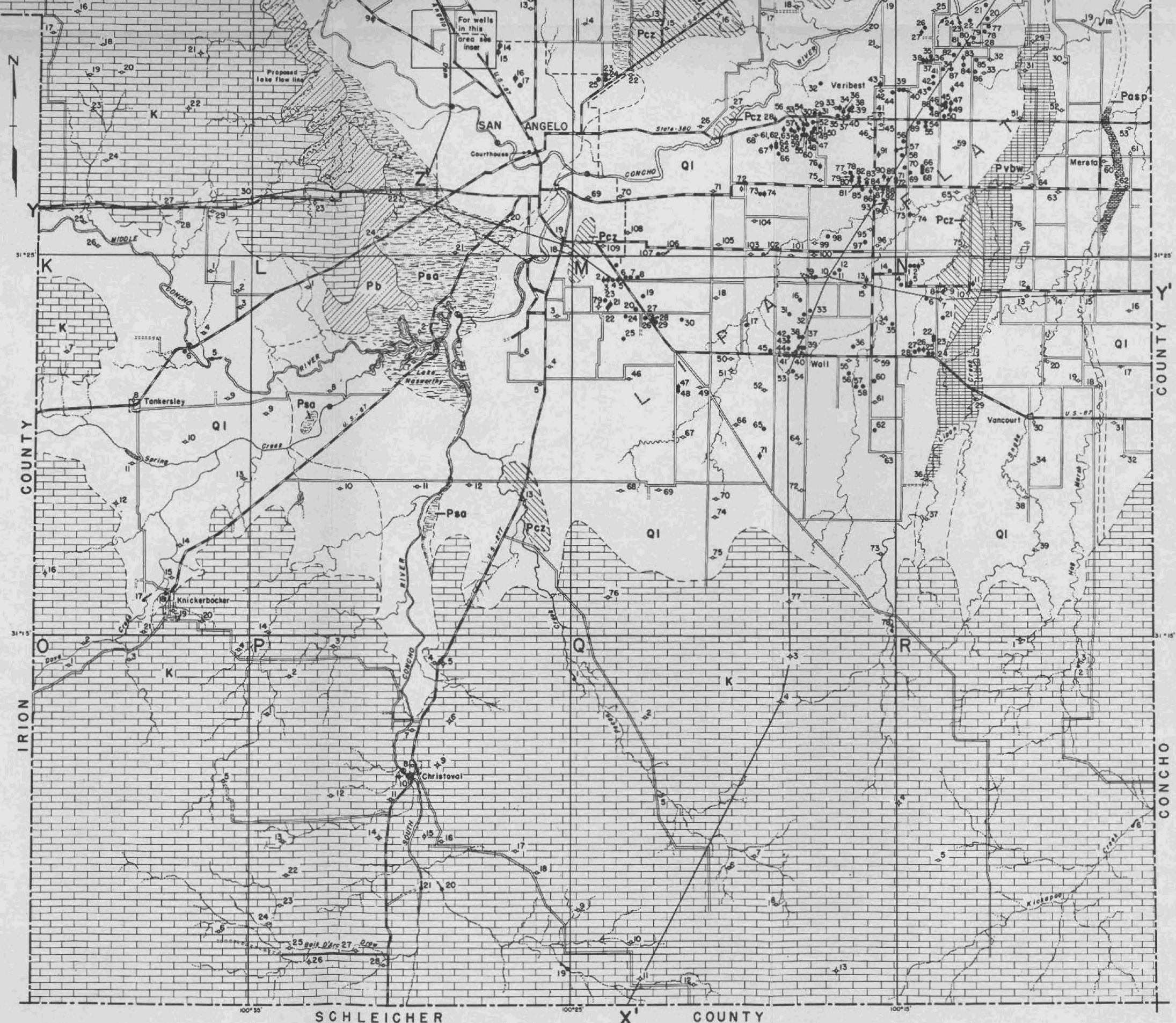
MAP OF TOM GREEN COUNTY, TEXAS, SHOWING WELLS, SPRINGS, AND GEOLOGIC FORMATIONS
