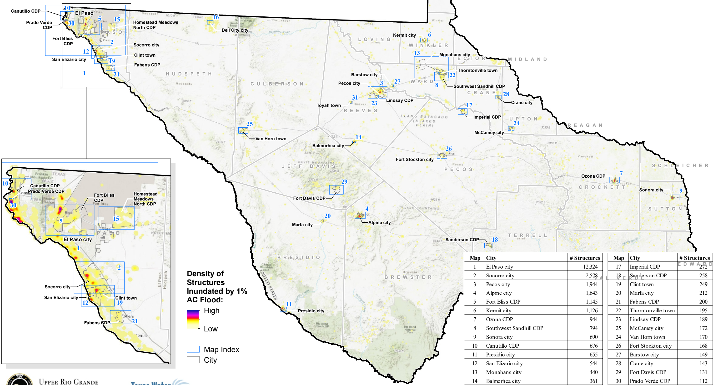
Map 15 Index: Greatest Flood Risk - Density of Structures Inundated by 1% AC Flood
