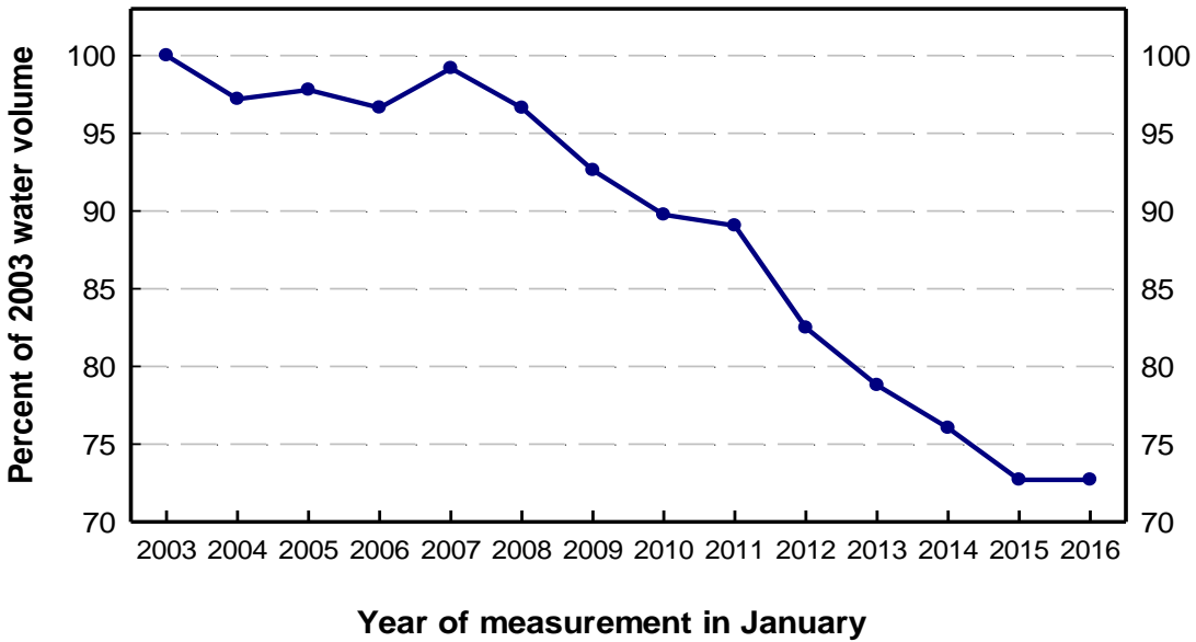
Figure 13. Change in water storage in TAWC project area from 2003 to 2016 expressed as percentage of the volume in 2003 (1,748,630 acre-feet).
